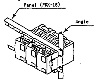
Fig.2 Wall Mounting
