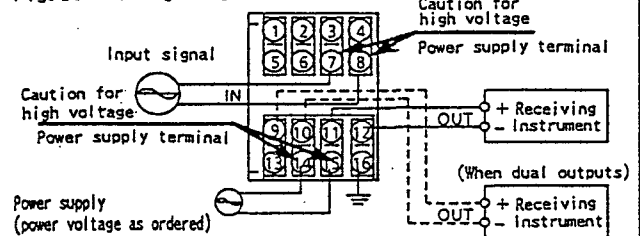
Fig.10 Wiring Diagram
