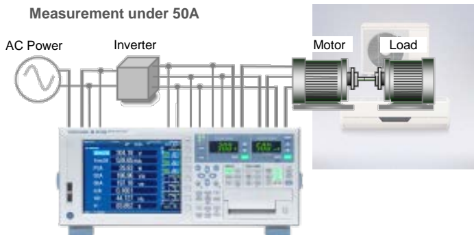
High Performance Power Analyzer WT1800E
