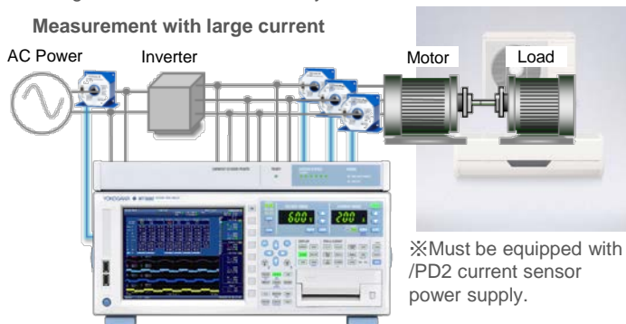
High Performance Power Analyzer WT1800E
