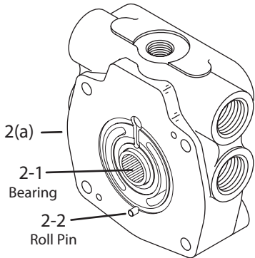
2(a) Accepts Gerotor Charge Pump
