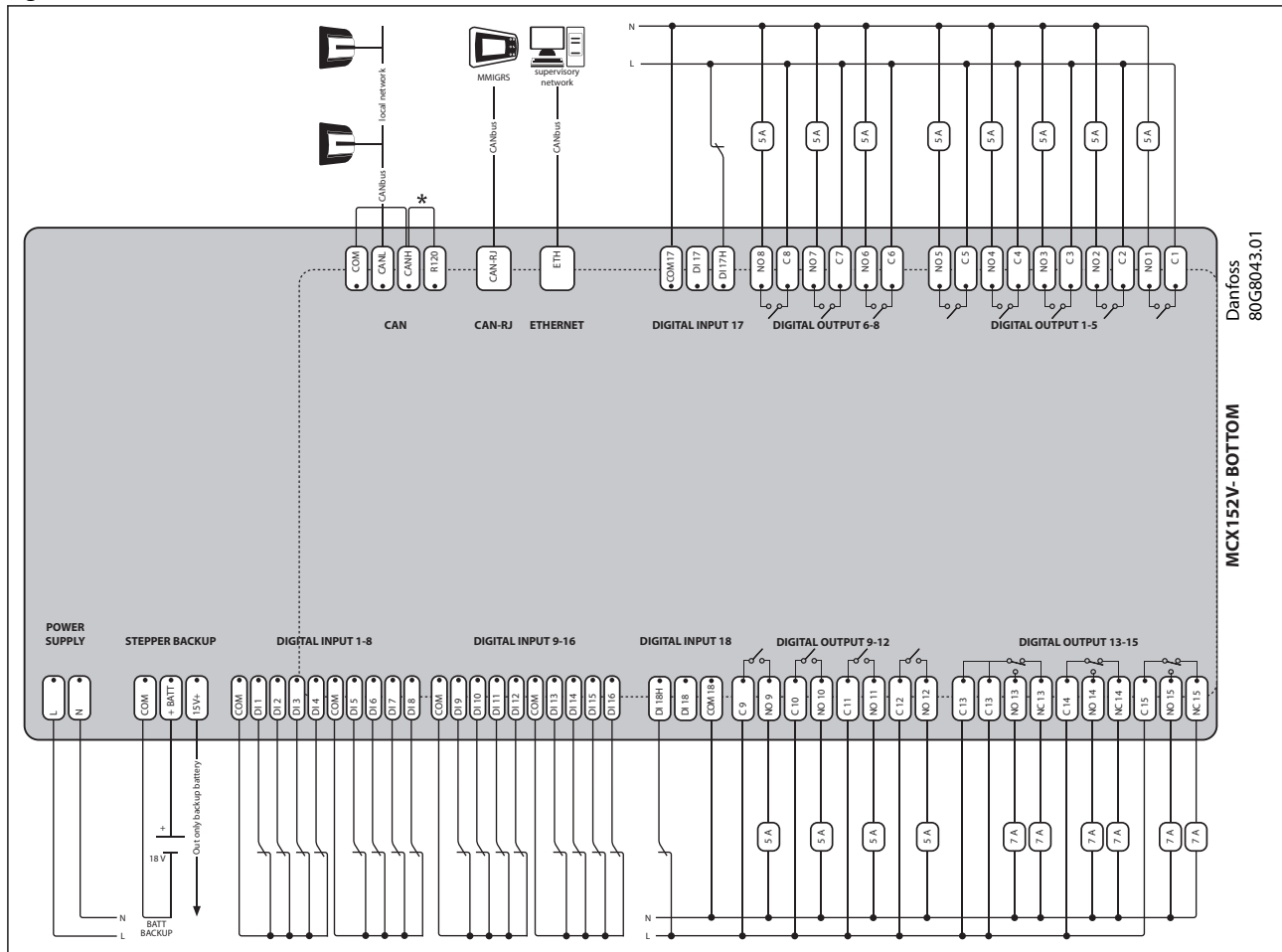
Figure 2: Bottom board
