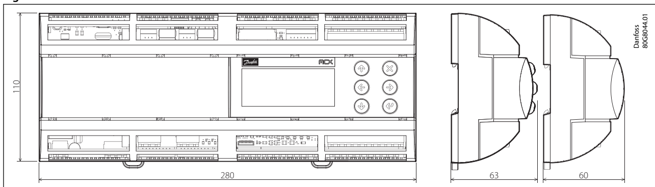
Figure 3: Dimensions
