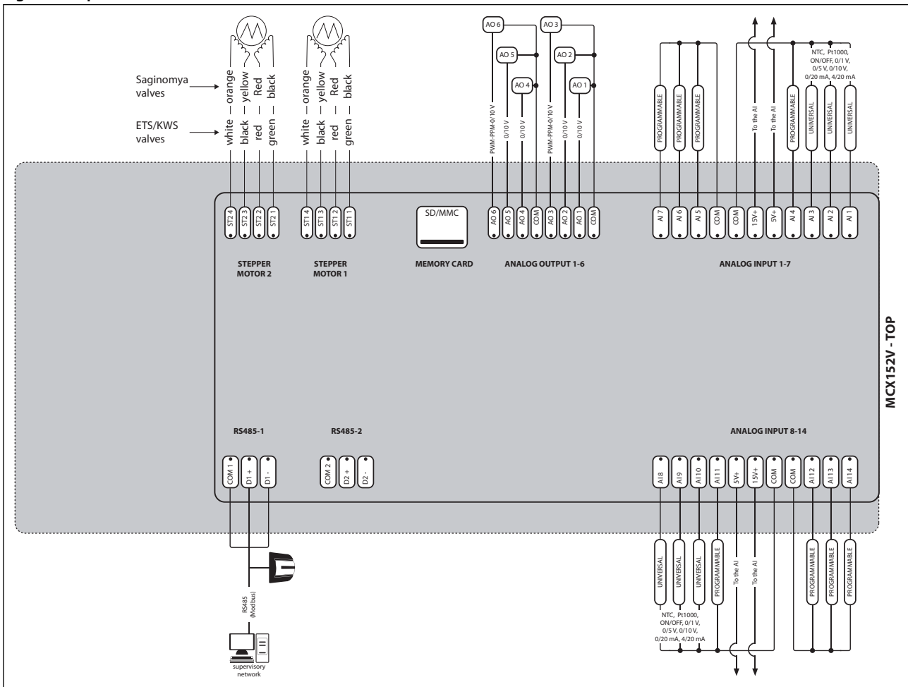
Figure 1: Top board
