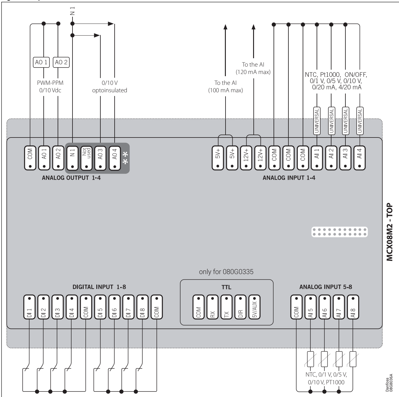
Figure 1: Top board
