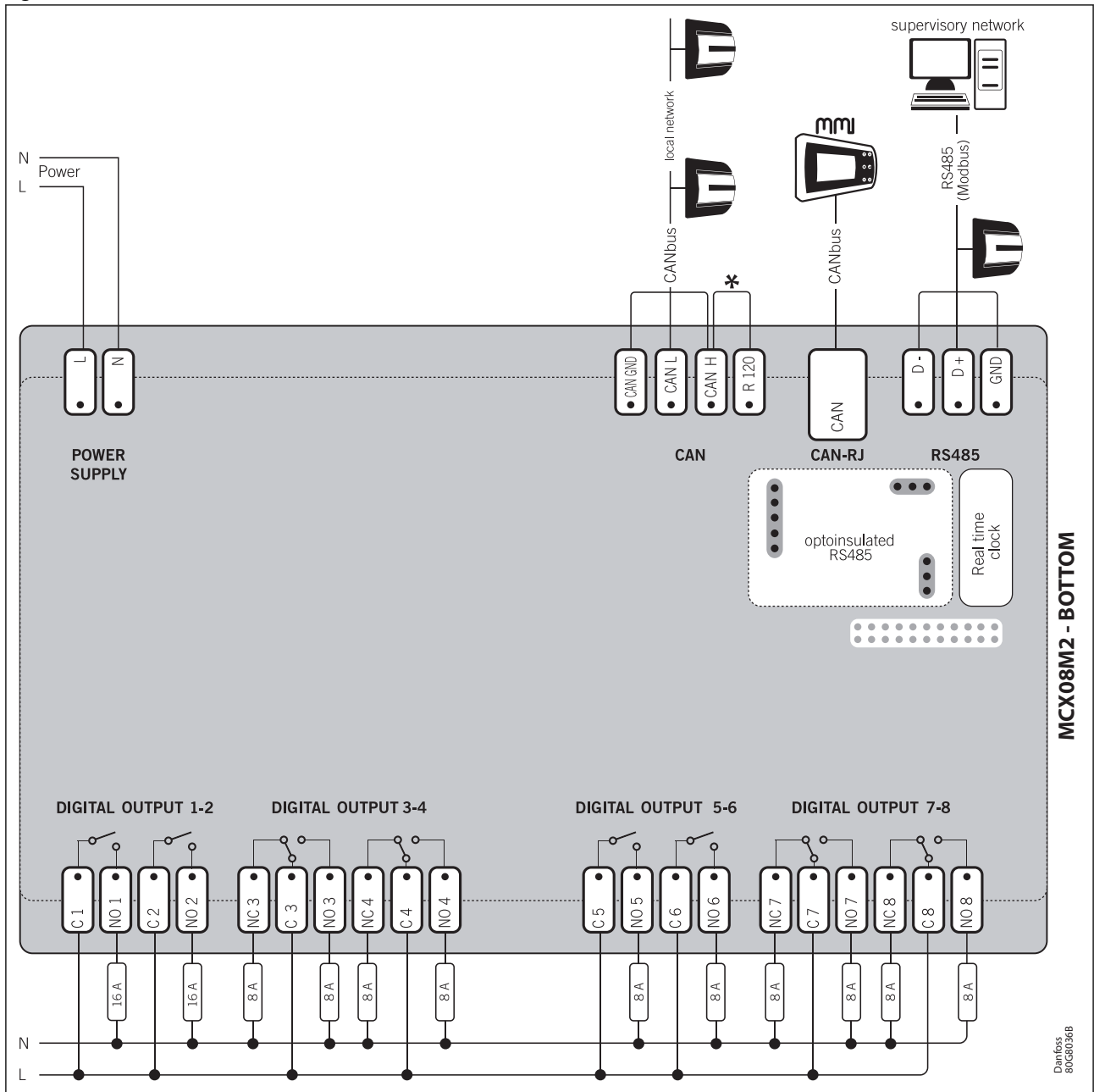
Figure 2: Bottom board
