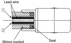
(Bore size G1/2 Tightening torque 0.5 to 0.6 N·m)
