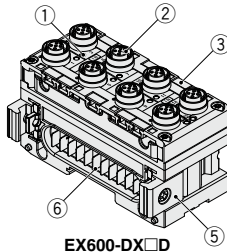
EX600-DX□D
