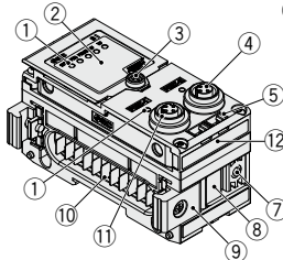
EX600-SEN7/8 EX600-SPN3/4 EX600-SEC3/4
