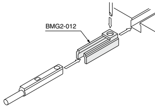
D-A9□(V)/M9□(V)/M9□W(V)
