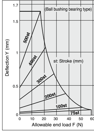
MGGL 25-Stroke
