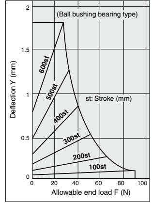
MGGL 32-Stroke
