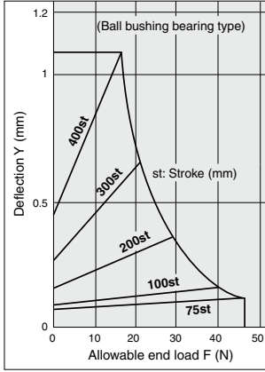
MGGL 20-Stroke
