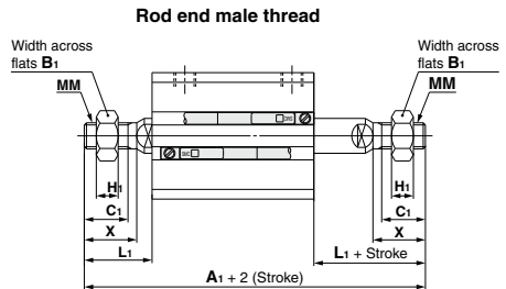
Rod End Male Thread
