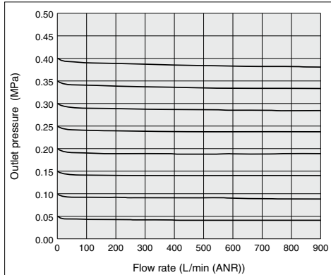
ARP40(K) Rc 1/2
