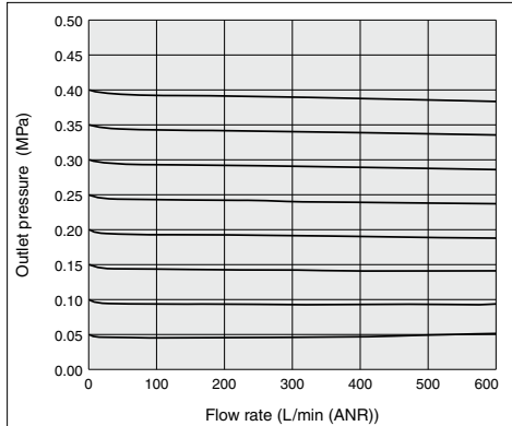
ARP30(K) Rc 3/8
