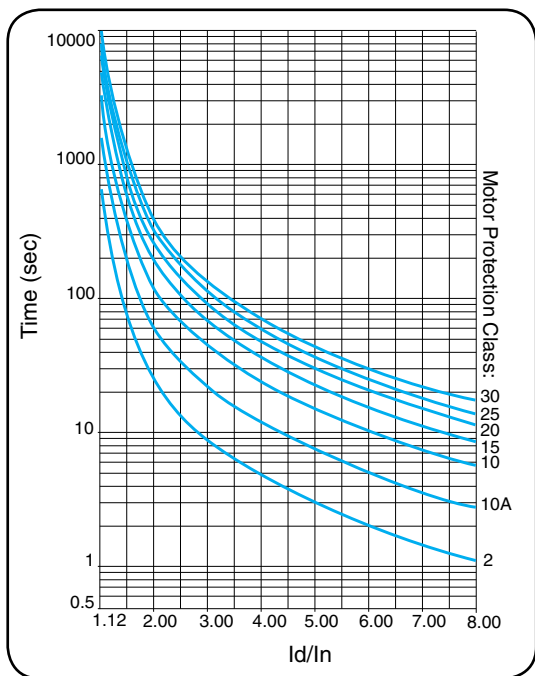
Motor thermal protection curves (cold)
