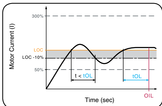
Motor overcurrent detection ( OIL )
