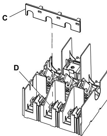
Figure / Figura / Figure 2 : Barrier Installation / Instalación de la barrera / Installation de la cloison
