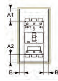
3P/4P
