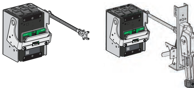
9422 Operating Mechanism with Flange-Mounted Handle
