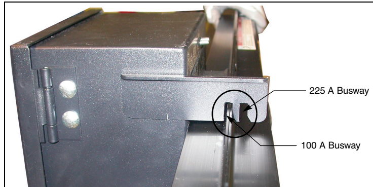
Figure 5: Plug-In Unit Top Flange Engagement
