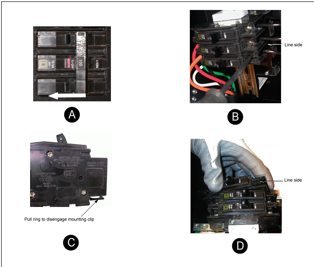
Figure 8: Removing/Replacing the QOU Circuit Breaker
