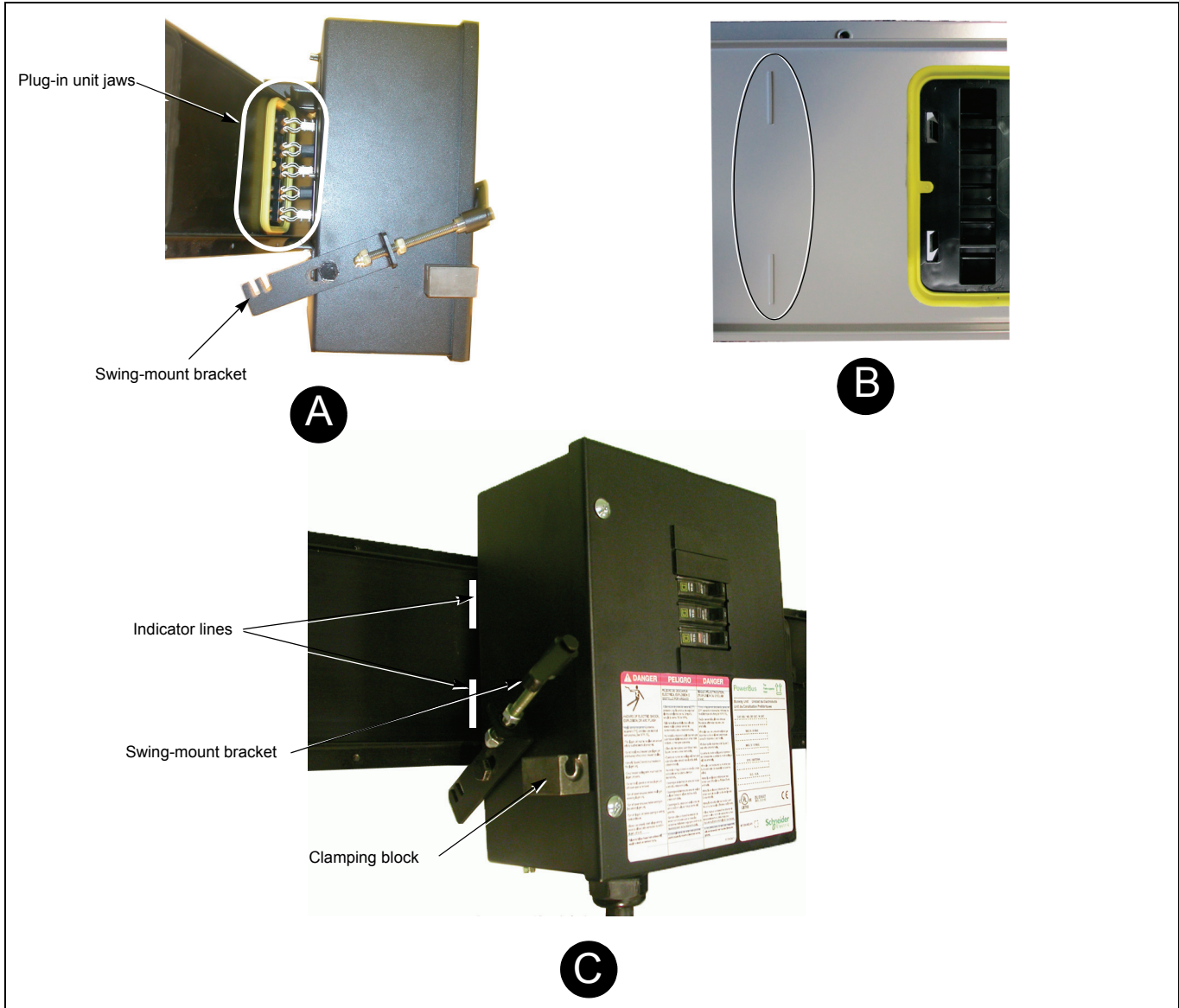
Figure 6: Plug-In Location
