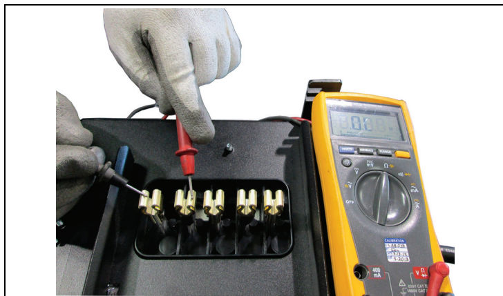
Figure 2: Testing for Plug-In Unit Continuity Prior to Installation
