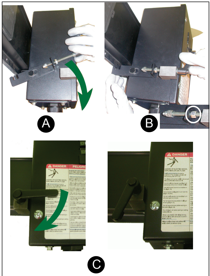
Figure 7: Securing the Plug-In Unit Onto the Busway
