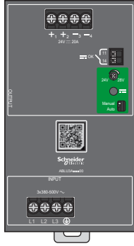
ABLU3A24200 ABLU3A48100
