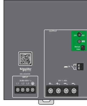
ABLU3A24400
