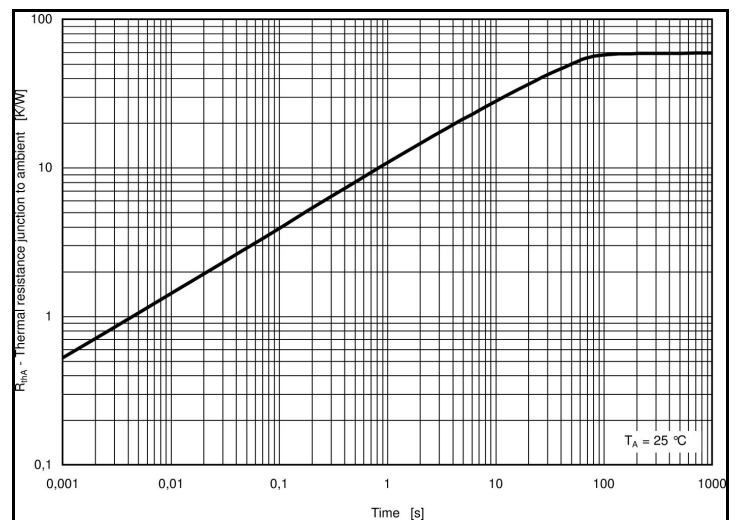
Fig. 1, Typical Transient Thermal Impedance
