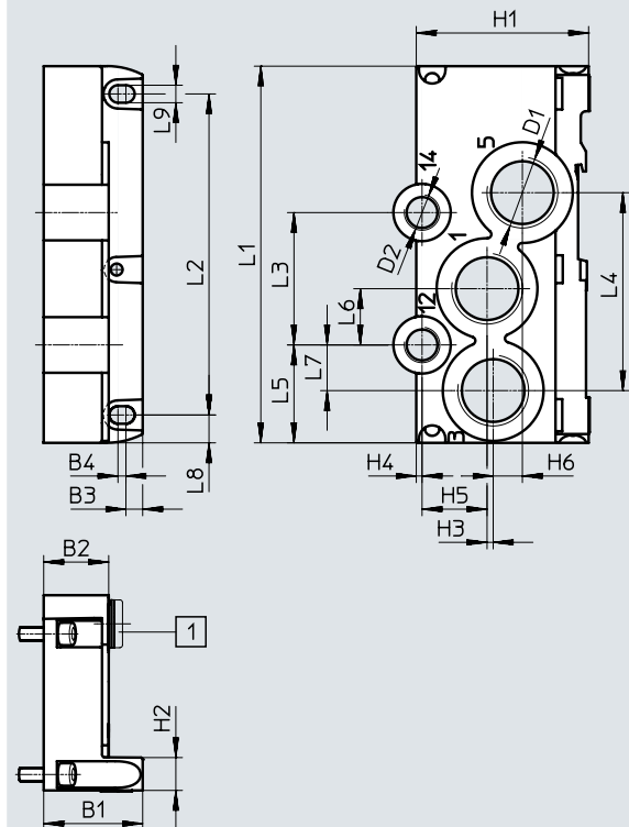
[1] Blanking plug
