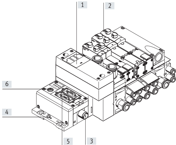
Electrical connection and display elements for VTSA-F-CB
