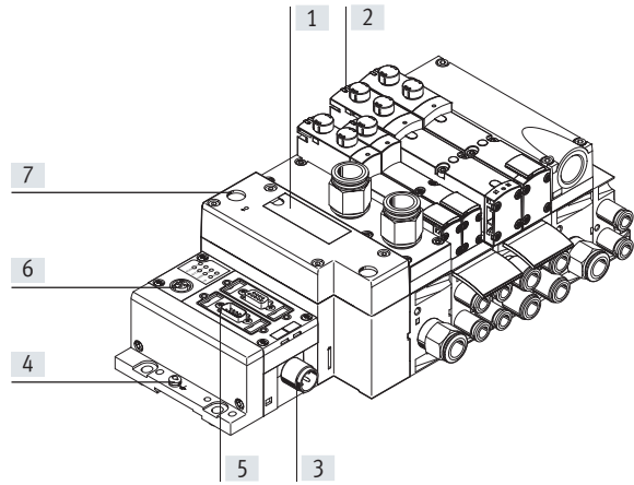
Electrical connection and display elements for VTSA-F-CB
