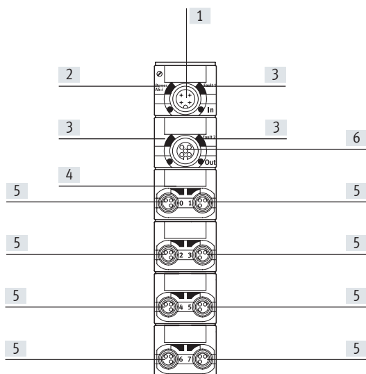
Pin allocation for sensor connections ASI-8DI-M8-3POL
