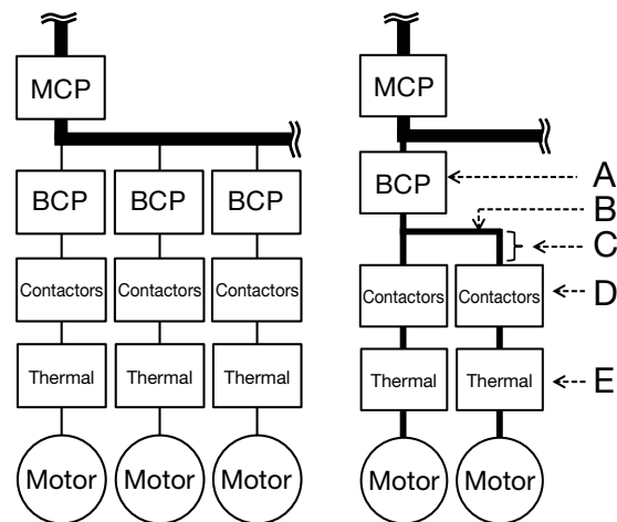
General Protection Circuit Example
