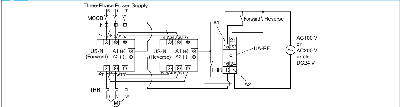
Fig. 2 Connecting US-N□(TE) and UA-RE Types
