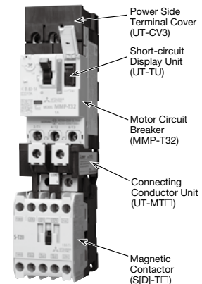
Combination Motor Controller Type F
