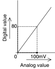
Voltage input characteristic(0 to 5V)
