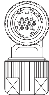
For CMV1-AP10S-M_
