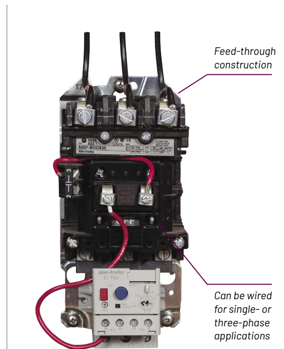
509 Open Starter
