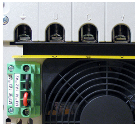
Shown with terminals jumpered for internal armature voltage feedback.
