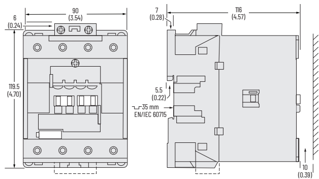
Figure 71 - 100-E80 4-Pole Contactors
