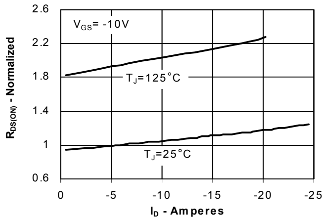
Fig. 5. R DS(ON) Normalized to I D25 Value vs. I D
