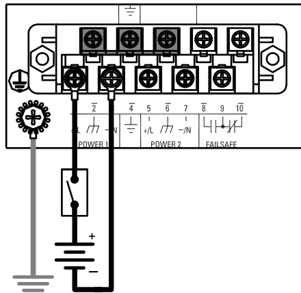
Figure 2.7 Single DC Power Supply
