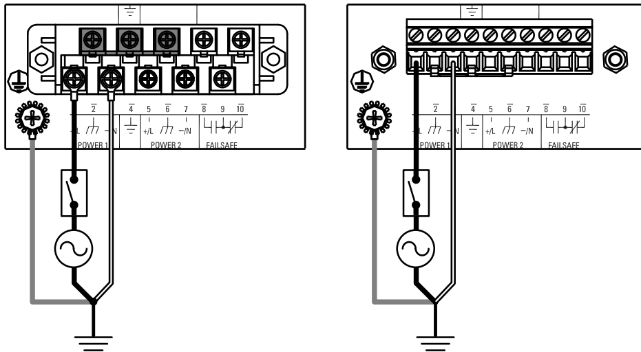
Figure 2.6 Single AC Power Supply
