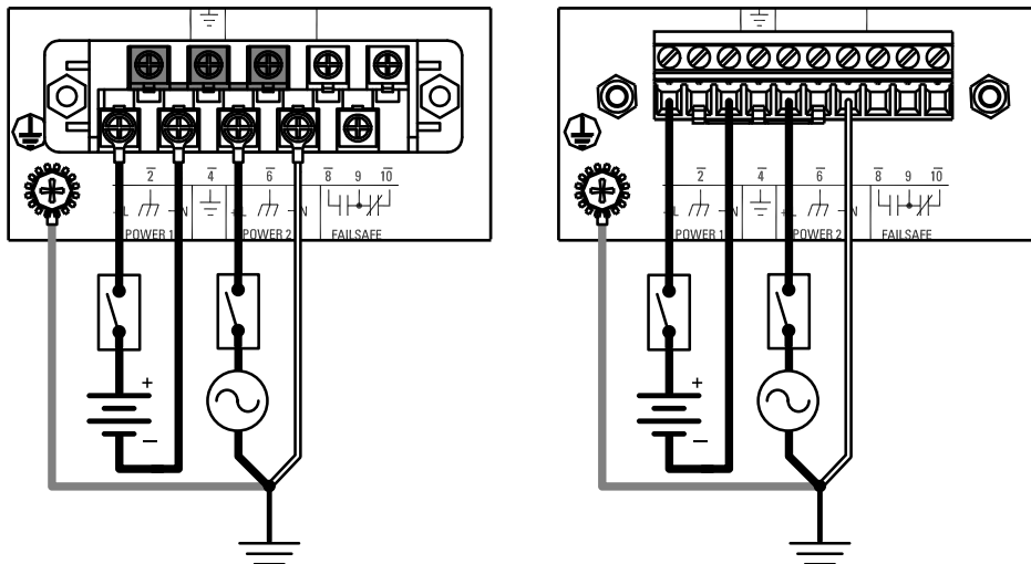
Figure 2.10 Dual AC/DC Power Supply
