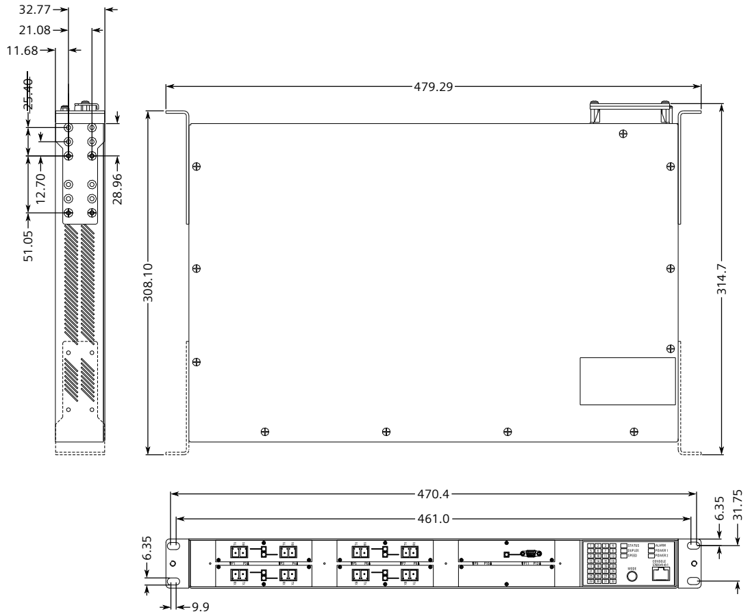
Figure 5.2 Rack Mount Dimensions
