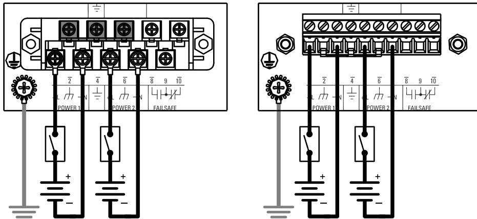
Figure 2.9 Dual DC Power Supply
