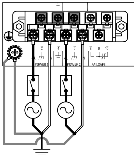
Figure 2.8 Dual AC Power Supply
