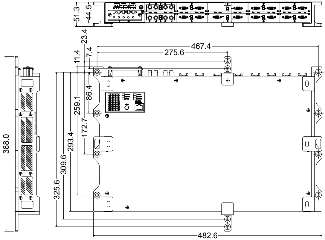
Figure 5.3 Panel Mount Dimensions
