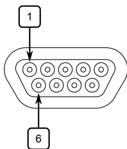
Figure 4.3 Micro-D 10/100/1000Base-TX Port Pin Configuration
