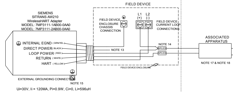
FIGURE # 2: LOOP POWER #2
