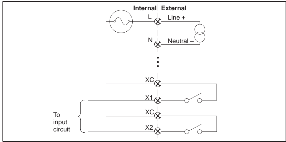
Figure 2-3 Input Wiring
