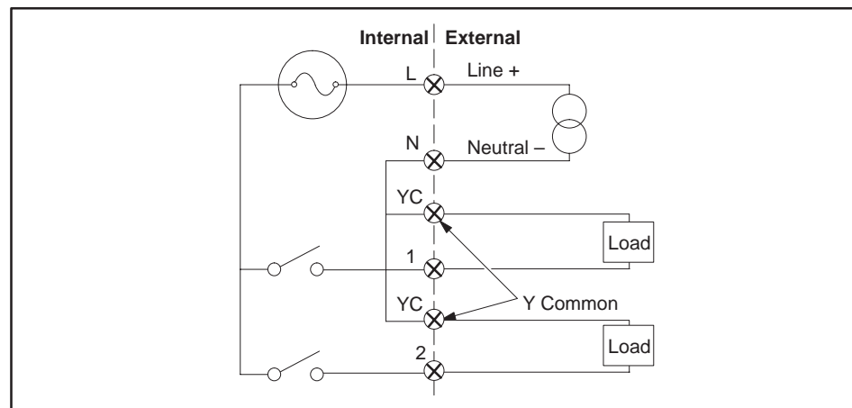
Figure 2-2 Output Wiring
