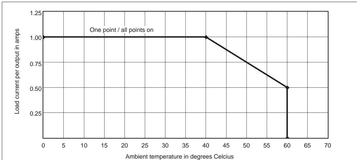
Figure A-1 Derating for Both Models
