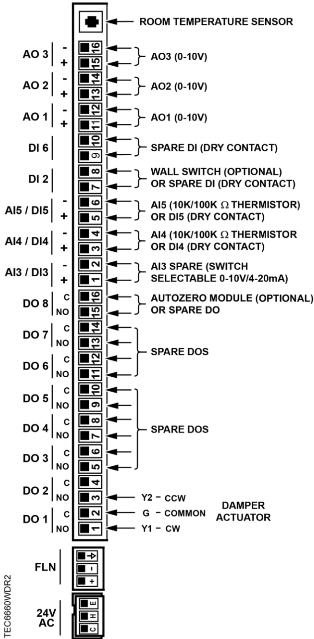
Application 6660 – Constant Volume Cooling Only.
