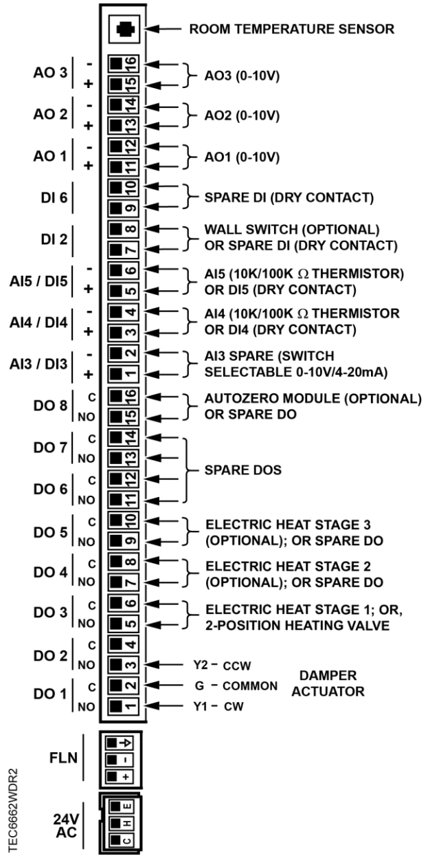
Application 6662 – Constant Volume with Electric Reheat.
