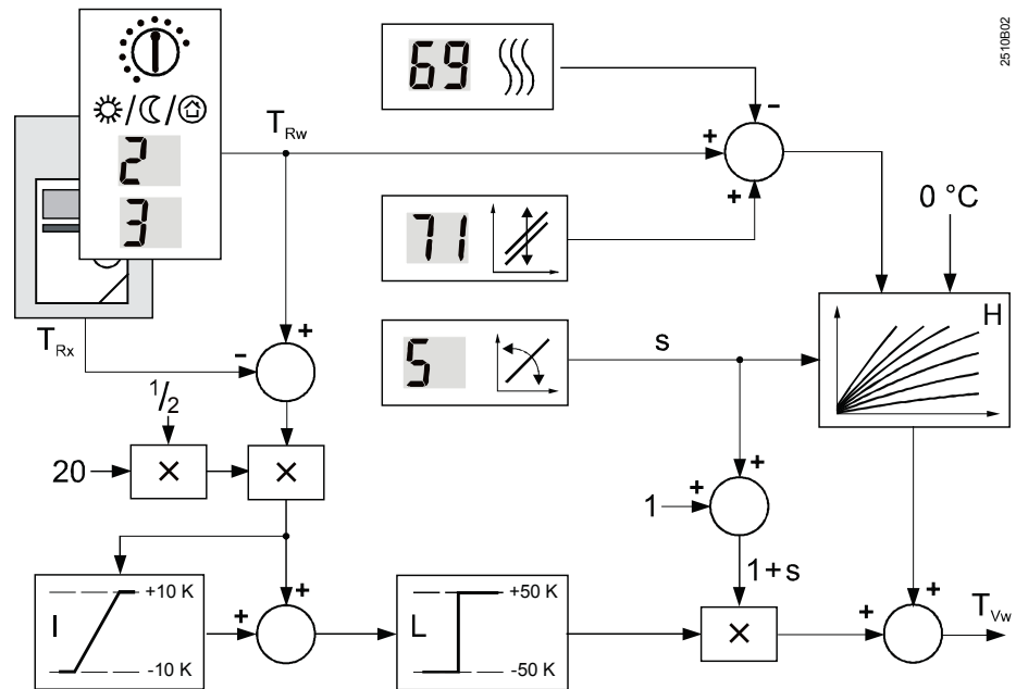
Generation of setpoint with room temperature-compensated control
