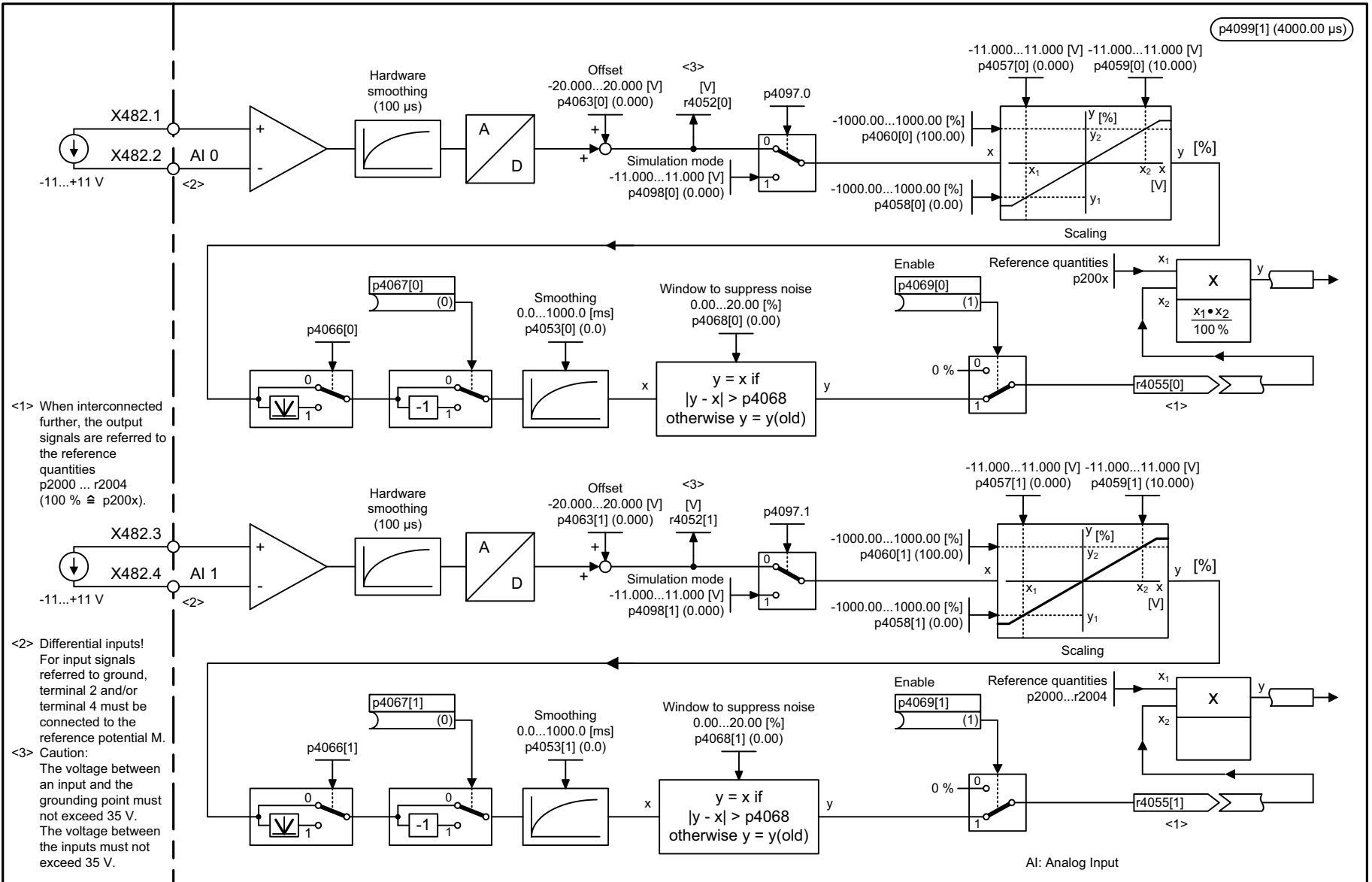
Fig. 3-359 9104 – Analog inputs (AI 0 ... AI 1)
