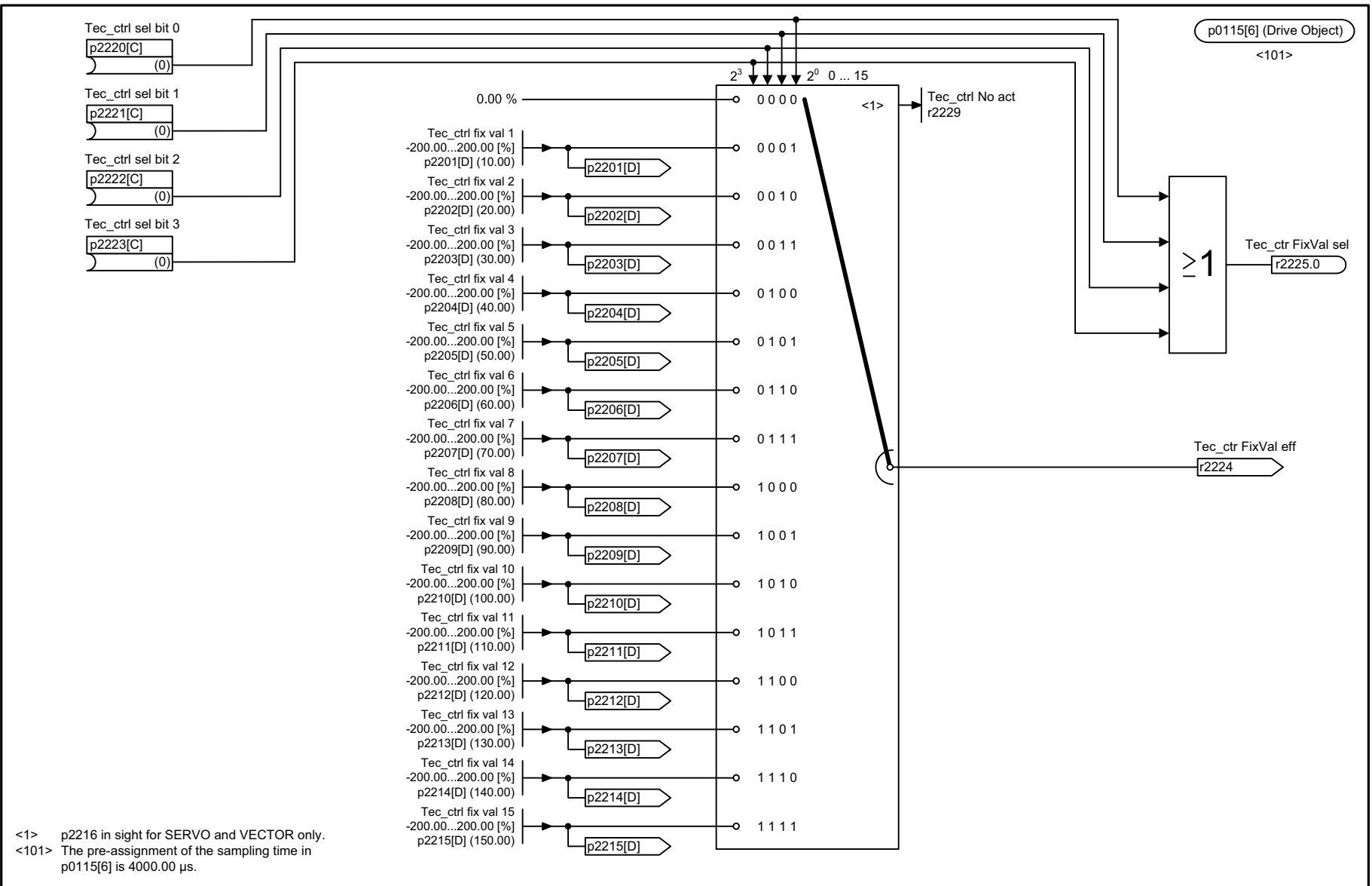
Fig. 3-277 7950 – Fixed values, binary selection (r0108.16 = 1 and p2216 = 2)
