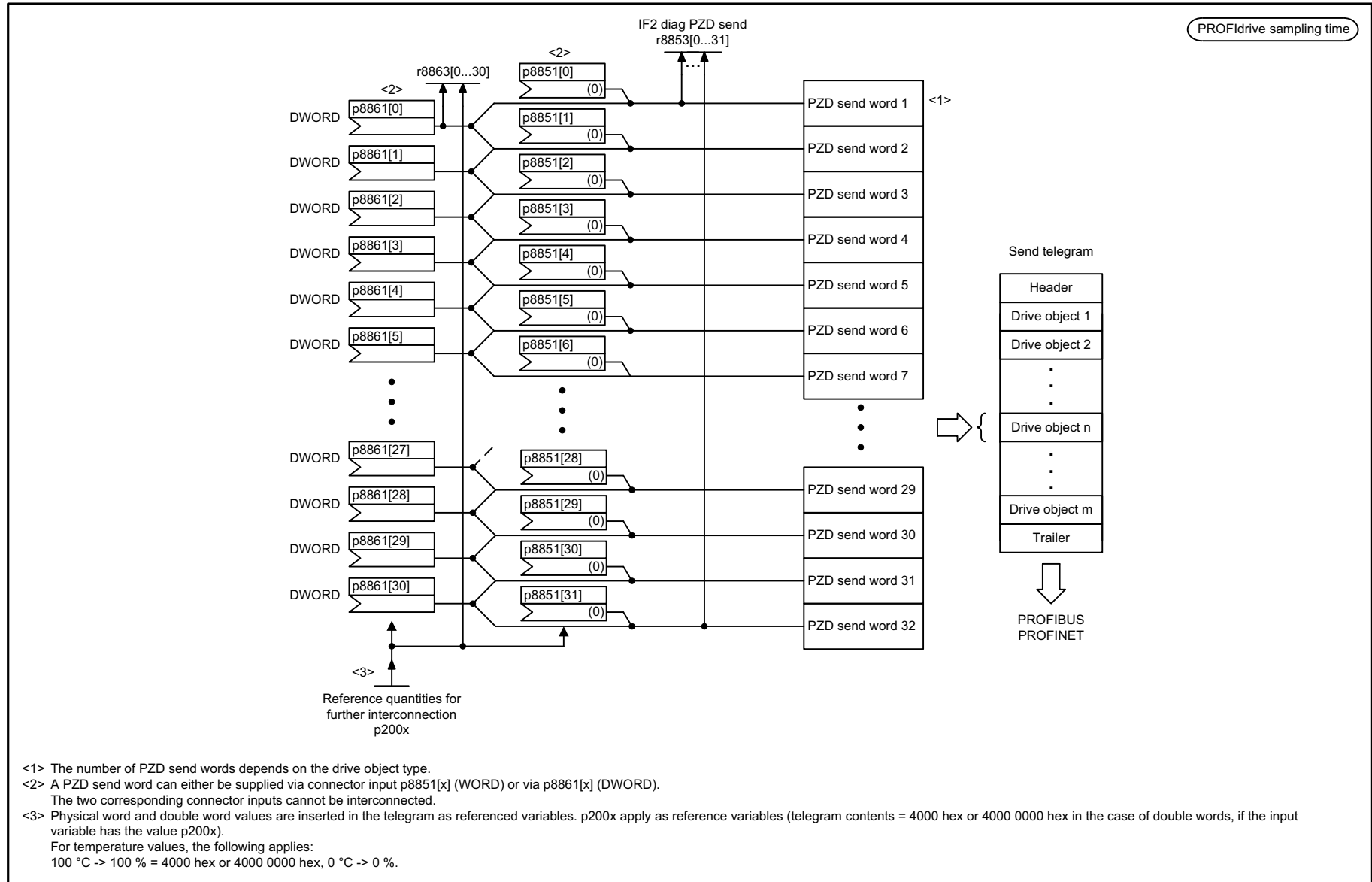
Fig. 3-85 2487 – IF2 send telegram free interconnection
