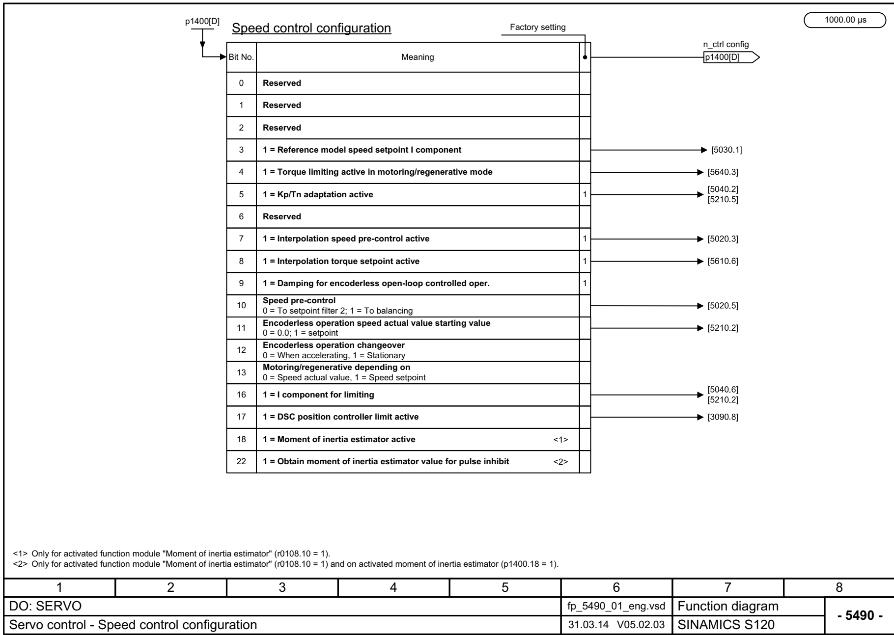
Fig. 3-220 5490 – Closed-loop speed control configuration
