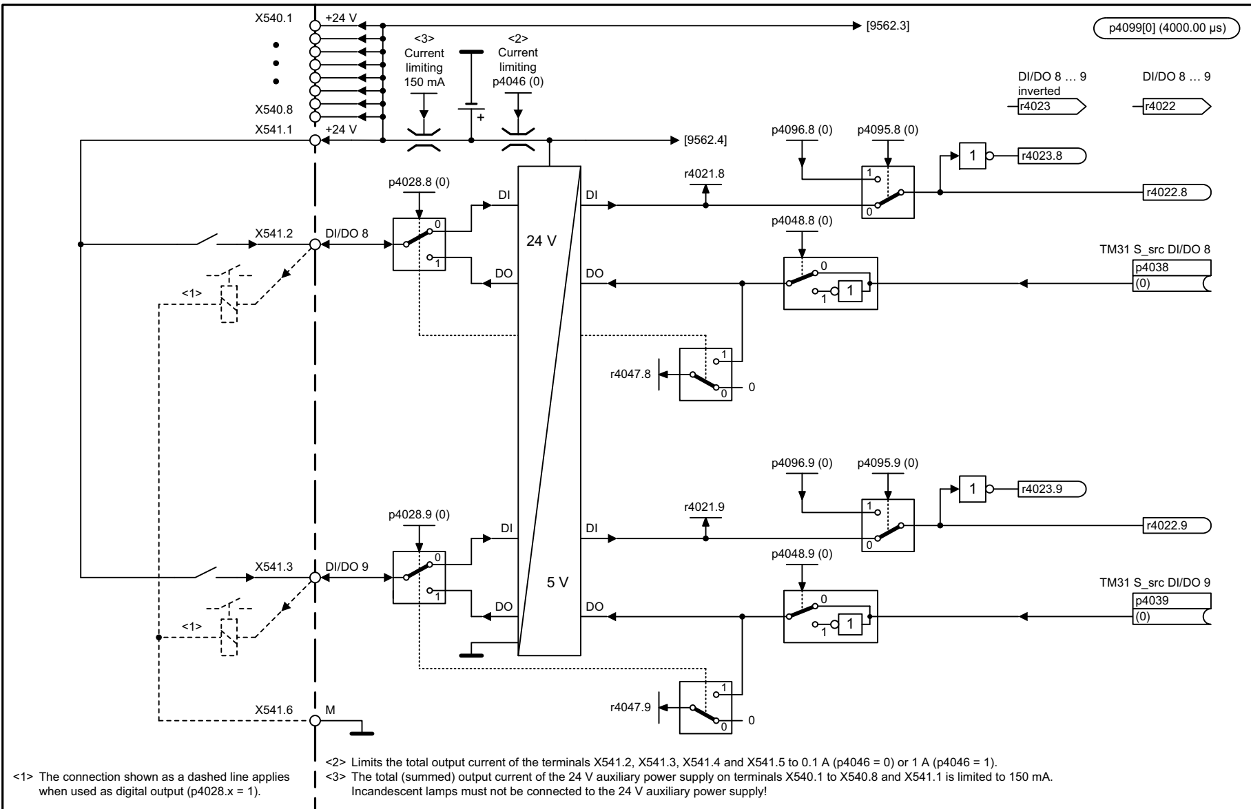
Fig. 3-377 9560 – Digital inputs/outputs bidirectional (DI/DO 8 ... DI/DO 9)
