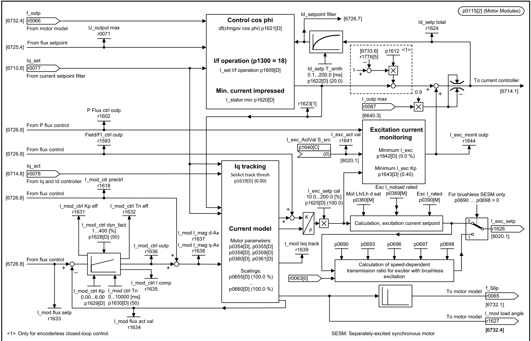
Fig. 3-259 6727 – Current model, excitation current monitoring, control cos phi (SESM, p0300 = 5)
