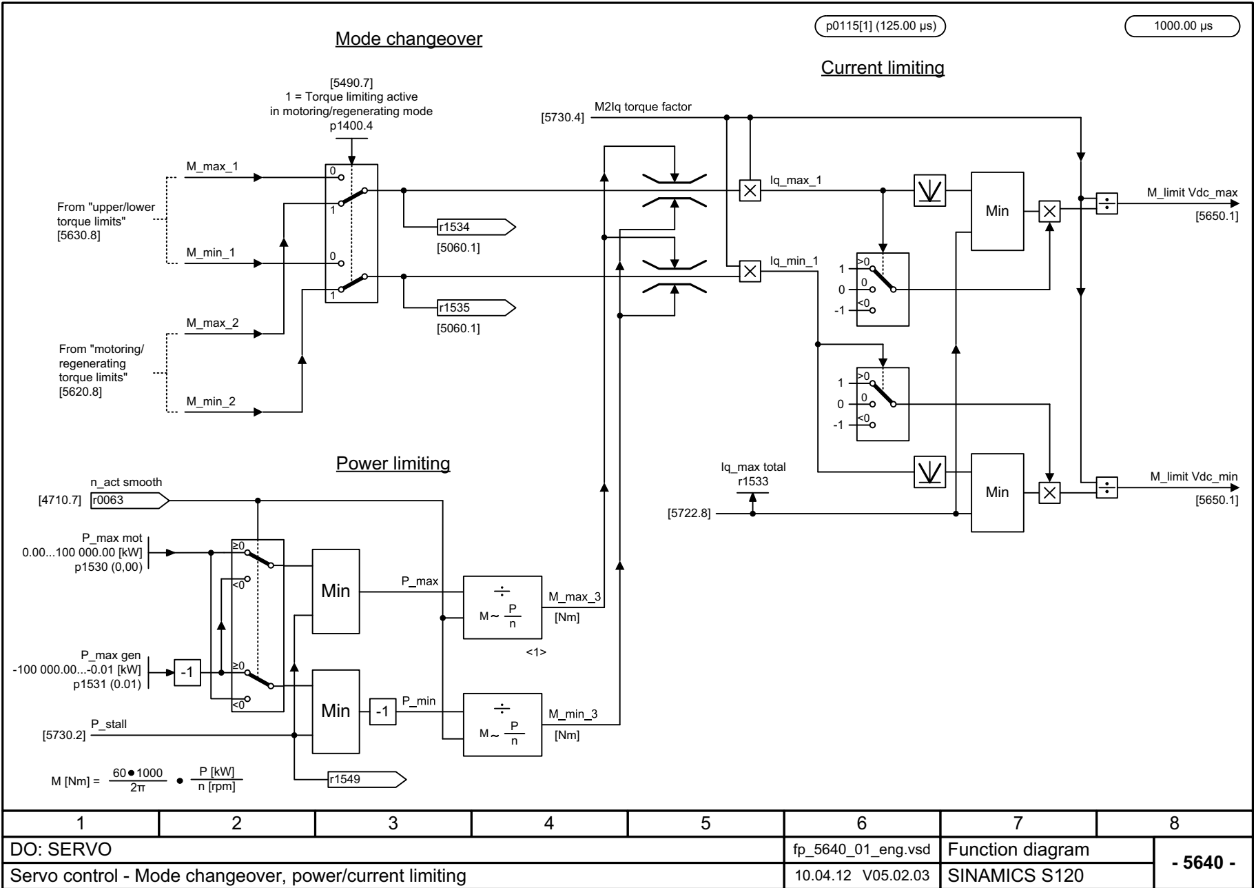
Fig. 3-225 5640 – Mode changeover, power/current limiting
