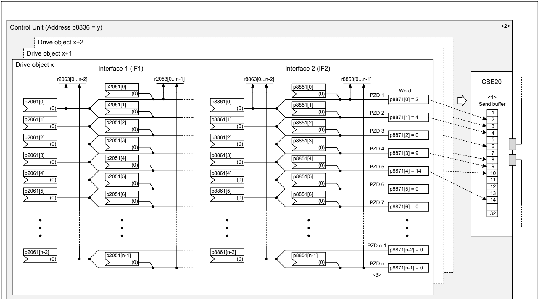
Fig. 3-30 2200 – SINAMICS link send data (r0108.31 = 1, p8835 = 3)
