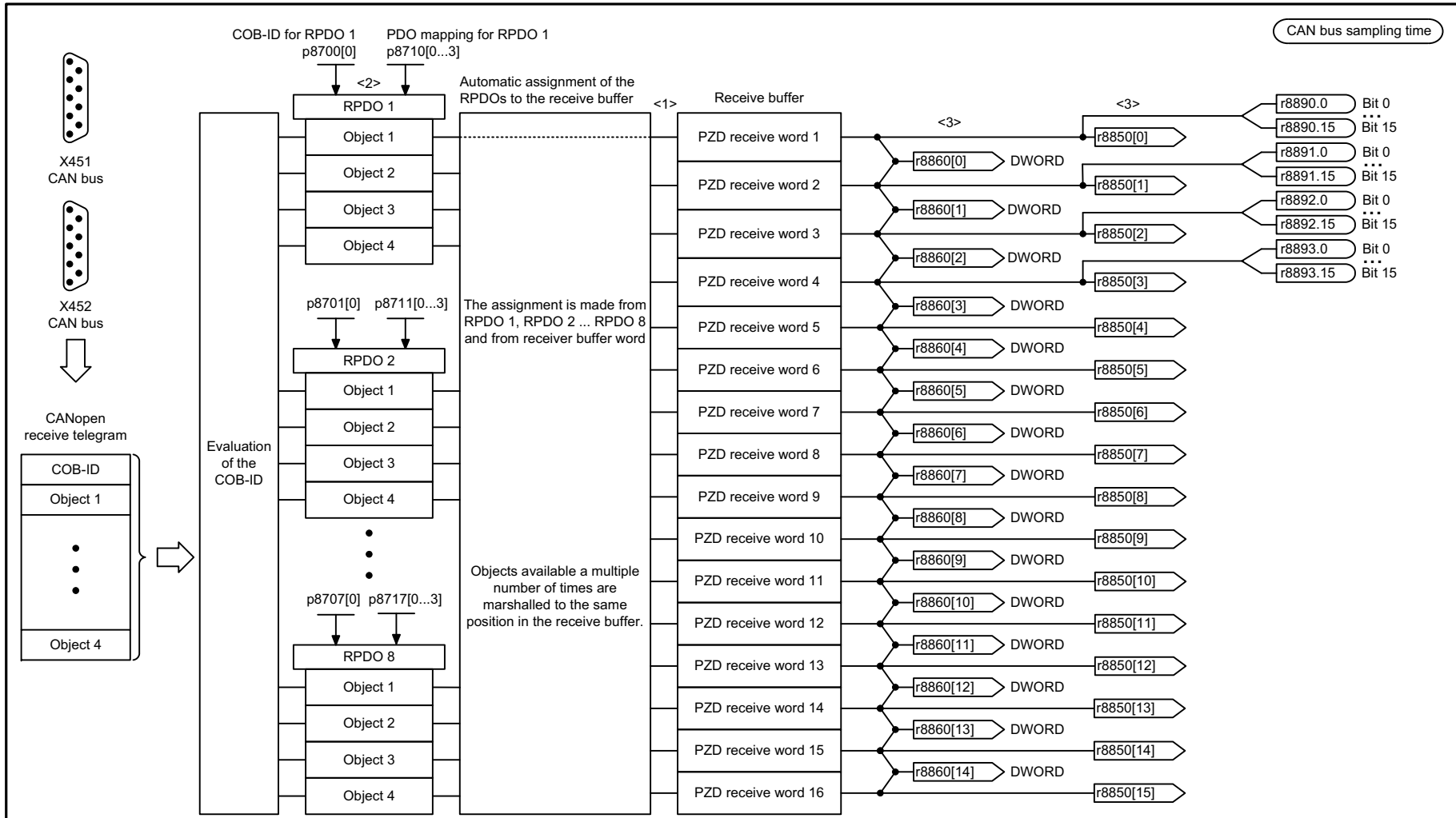
Fig. 3-361 9204 – Receive telegram free PDO mapping (p8744 = 2)
