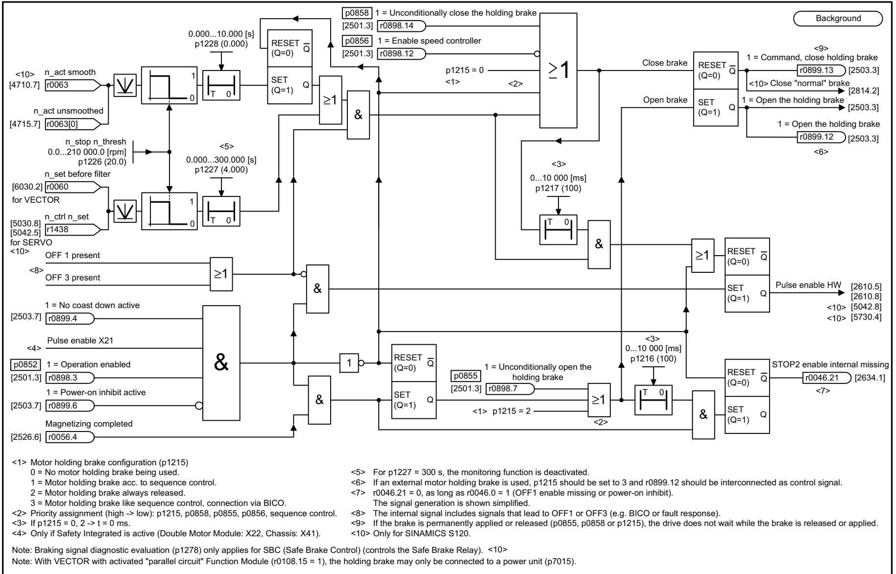
Fig. 3-109 2701 – Basic brake control (r0108.14 = 0)
