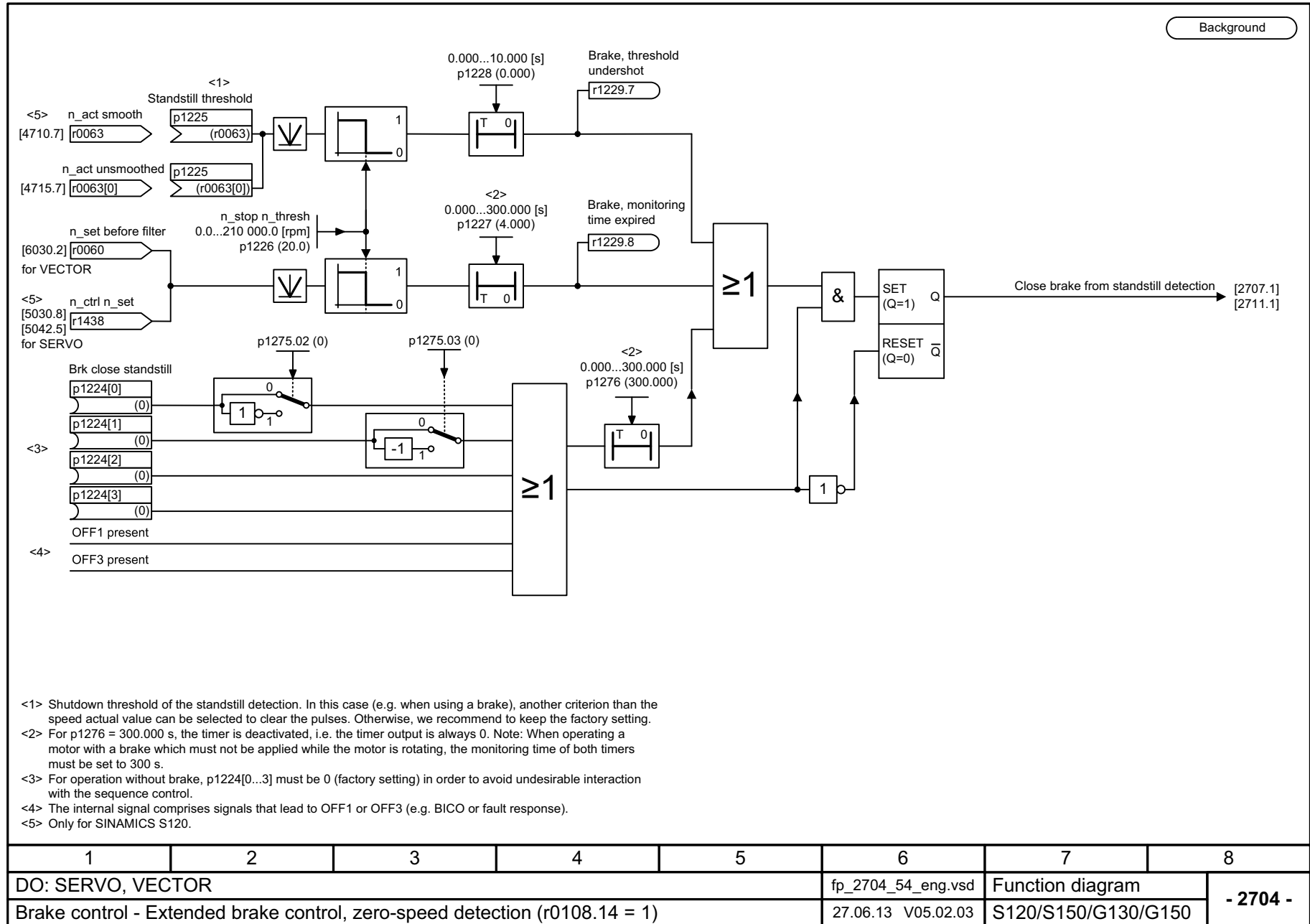
Fig. 3-110 2704 – Extended brake control, zero-speed detection (r0108.14 = 1)
