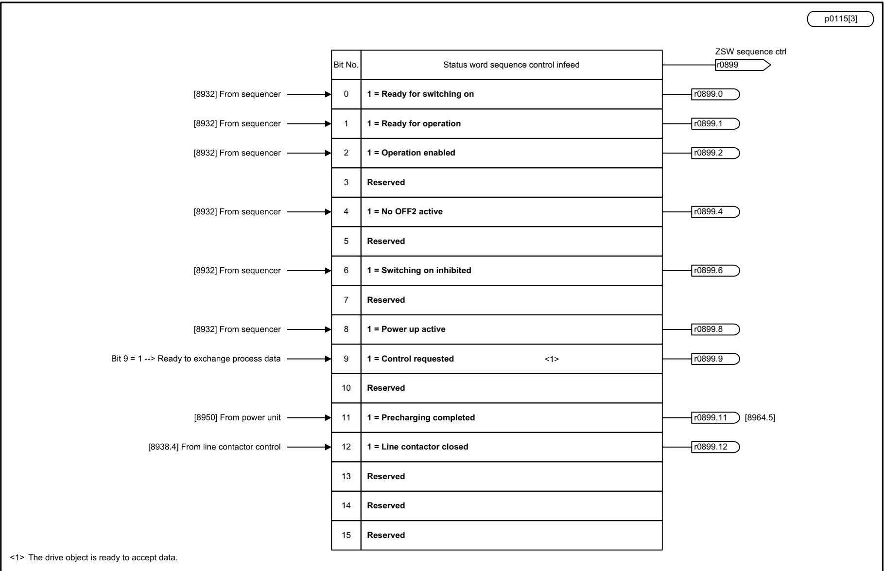
Fig. 3-344 8926 – Status word sequence control infeed
