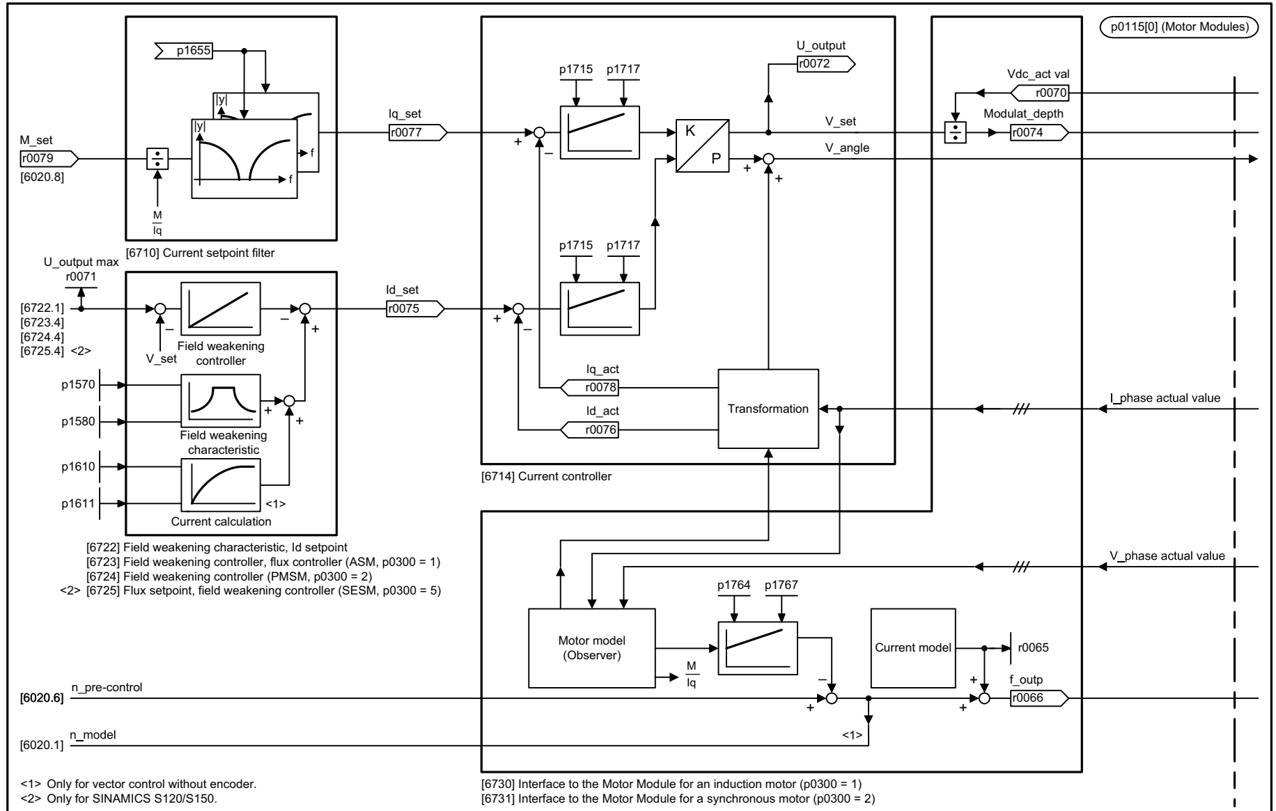
Fig. 3-250 6700 – Current control, overview
