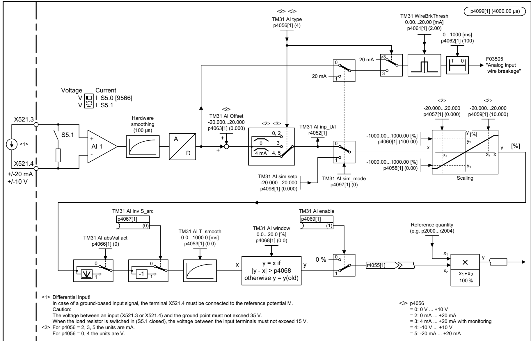
Fig. 3-380 9568 – Analog input 1 (AI 1)
