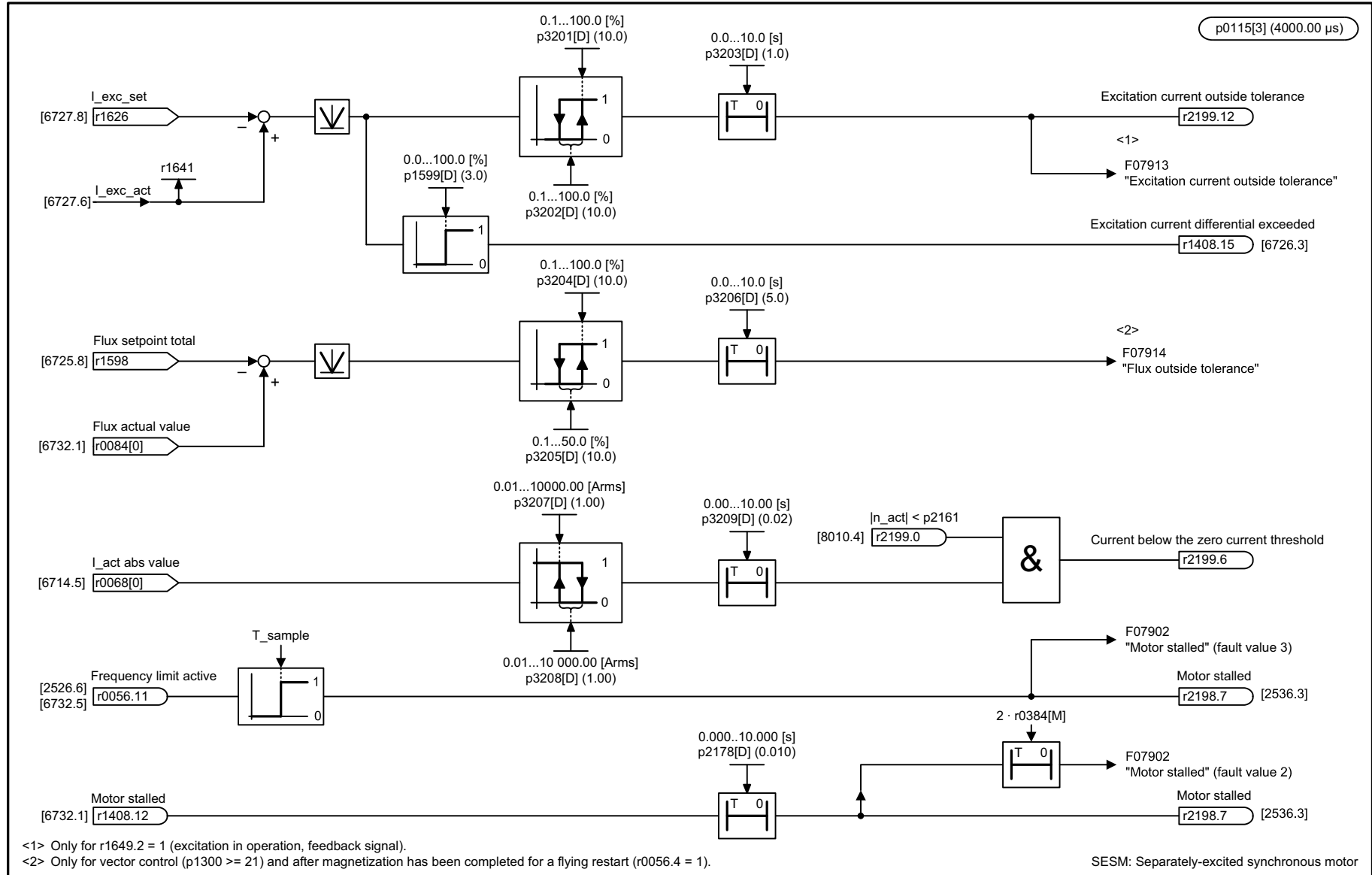
Fig. 3-310 8020 – Separately excited synchronous motor (SESM; p0300 = 5)
