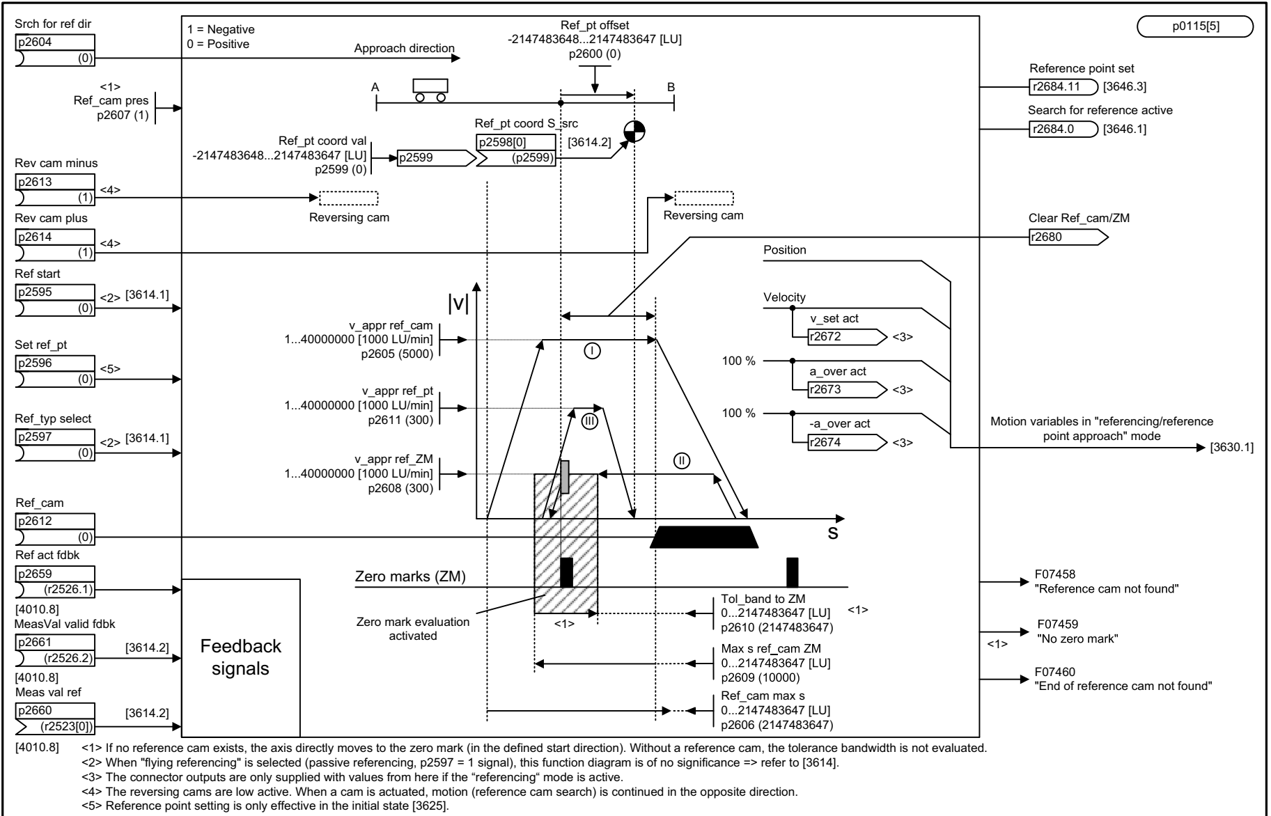
Fig. 3-169 3612 – Referencing/reference point approach mode (r0108.4 = 1) (p2597 = 0 signal)
