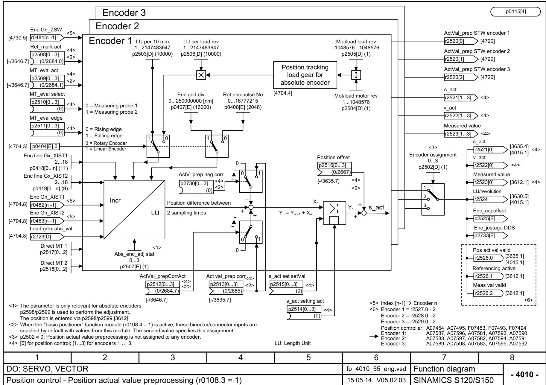
Fig. 3-183 4010 - Position actual value preprocessing (r0108.3 = 1)
