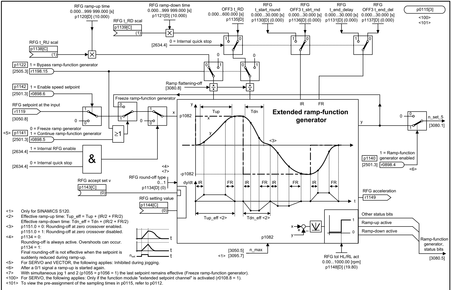
Fig. 3-163 3070 – Extended ramp-function generator
