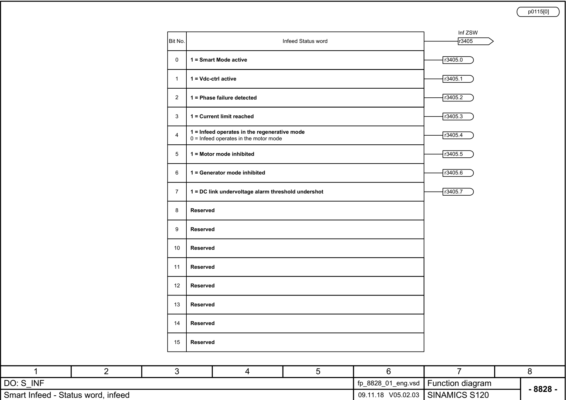
Fig. 3-336 8828 – Status word infeed
