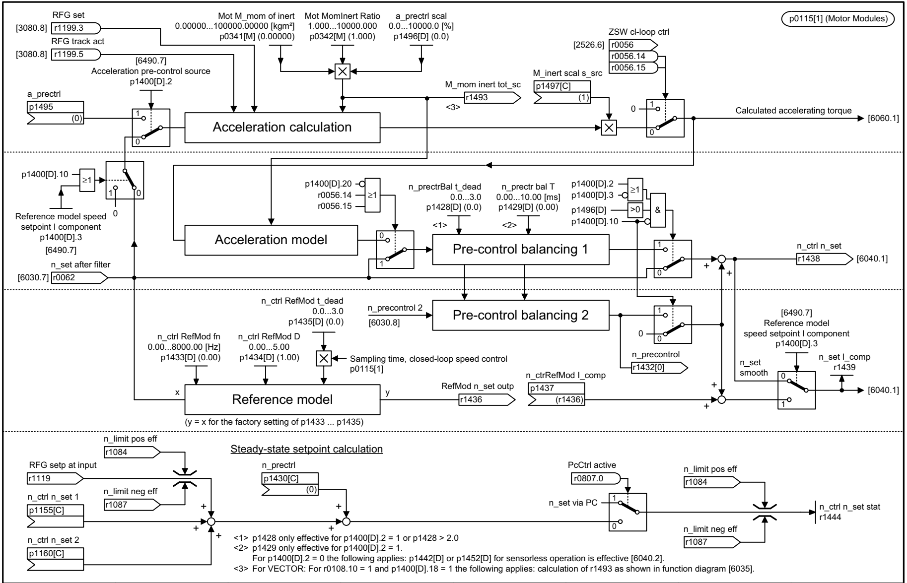
Fig. 3-235 6031 – Precontrol symmetrization, reference/acceleration model
