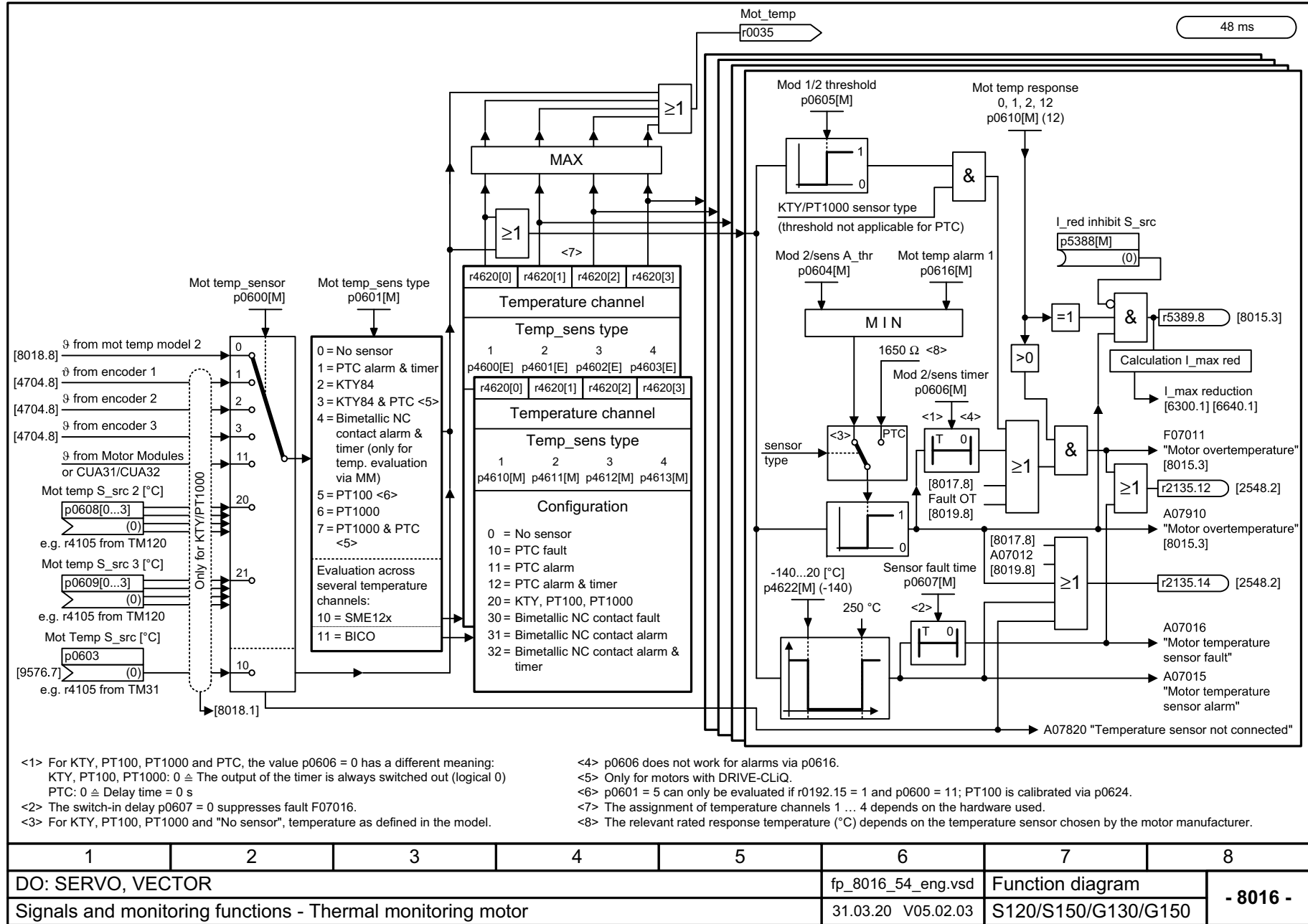
Fig. 3-306 8016 – Thermal motor monitoring
