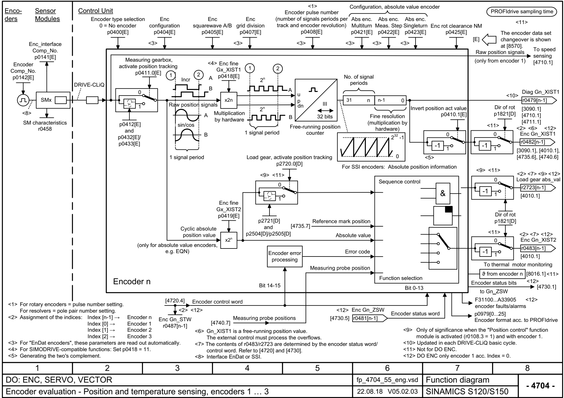
Fig. 3-189 4704 – Position and temperature sensing encoders 1 ... 3
