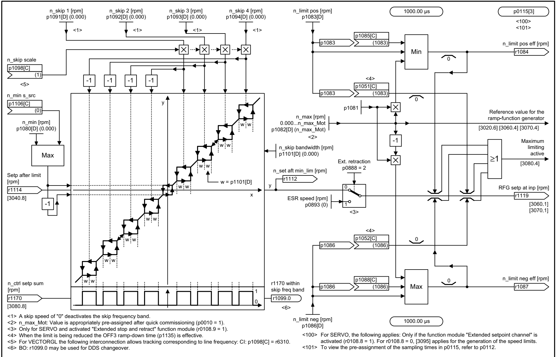
Fig. 3-161 3050 – Skip frequency bands and speed limitations
