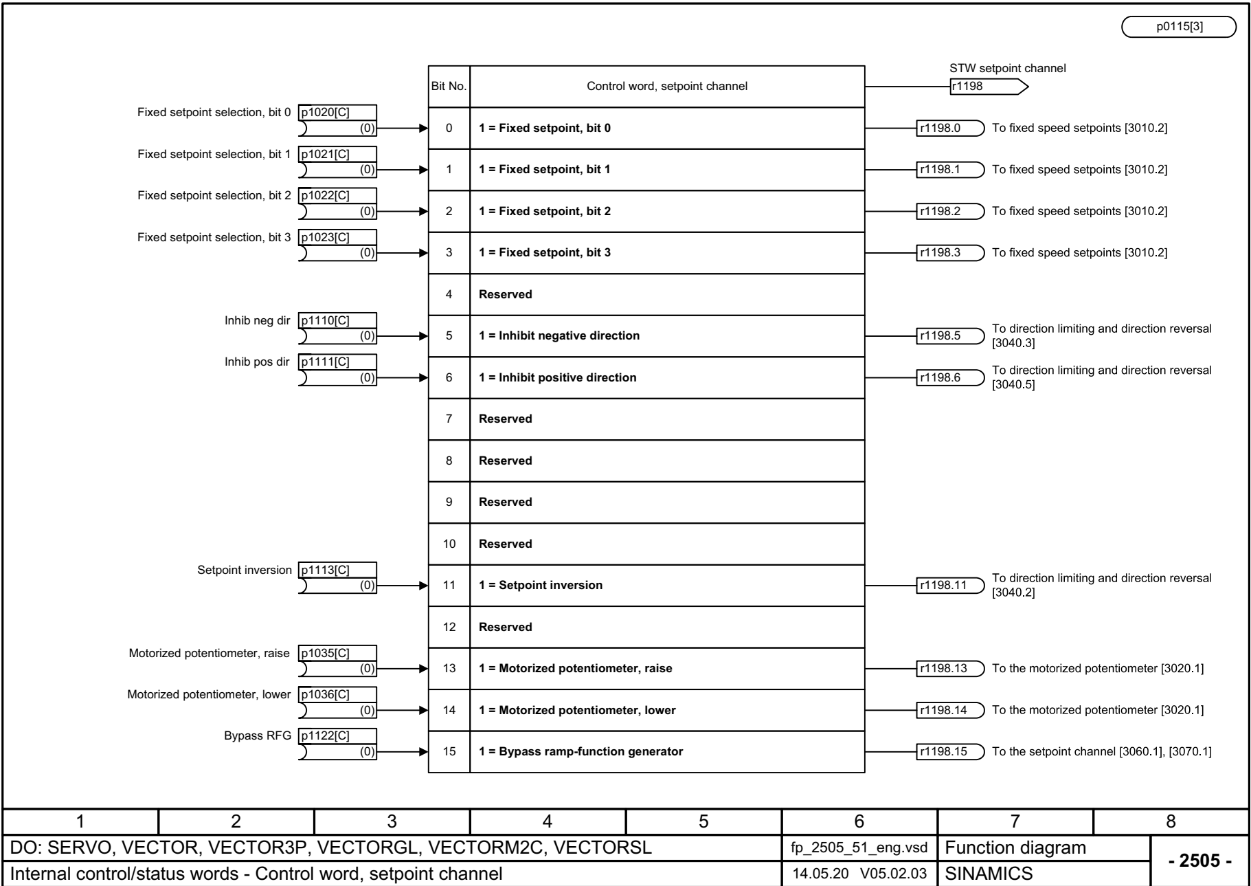
Fig. 3-97 2505 - Control word setpoint channel
