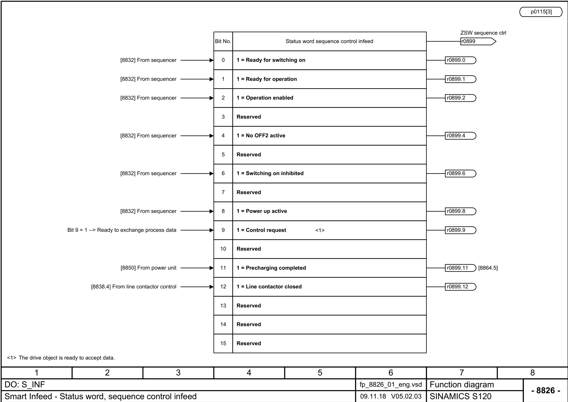
Fig. 3-335 8826 – Status word sequence control infeed
