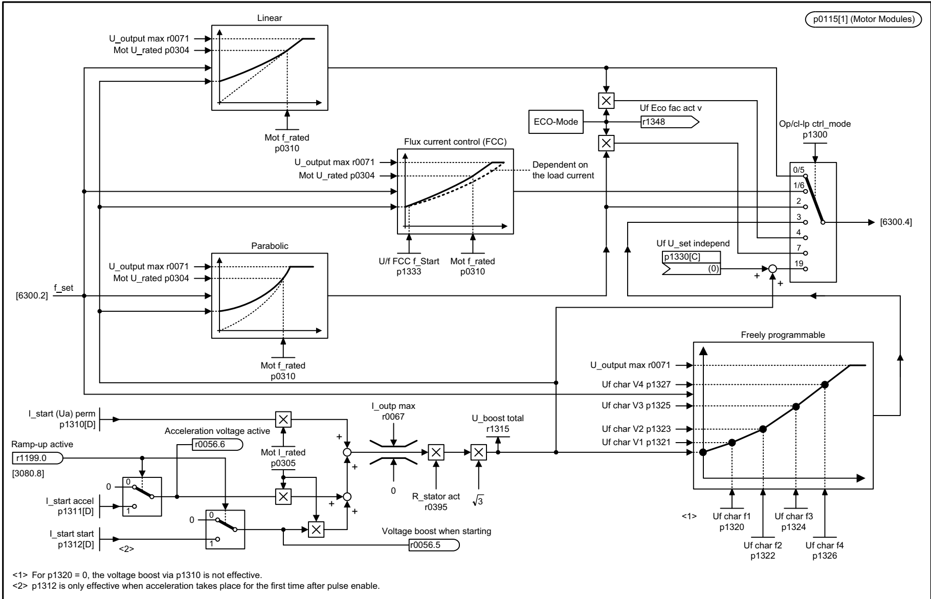
Fig. 3-242 6301 – U/f characteristic and voltage boost
