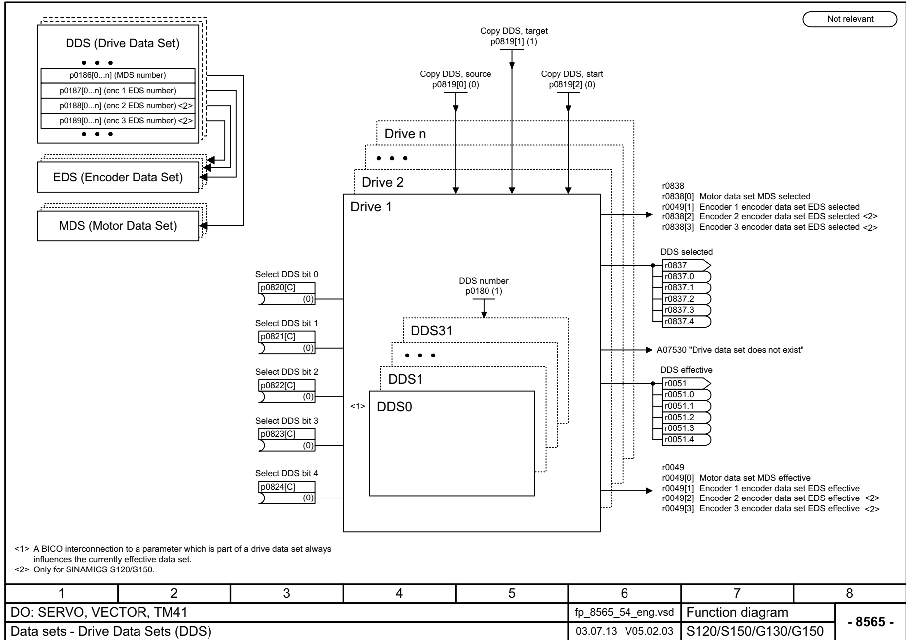
Fig. 3-322 8565 – Drive Data Sets (DDS)
