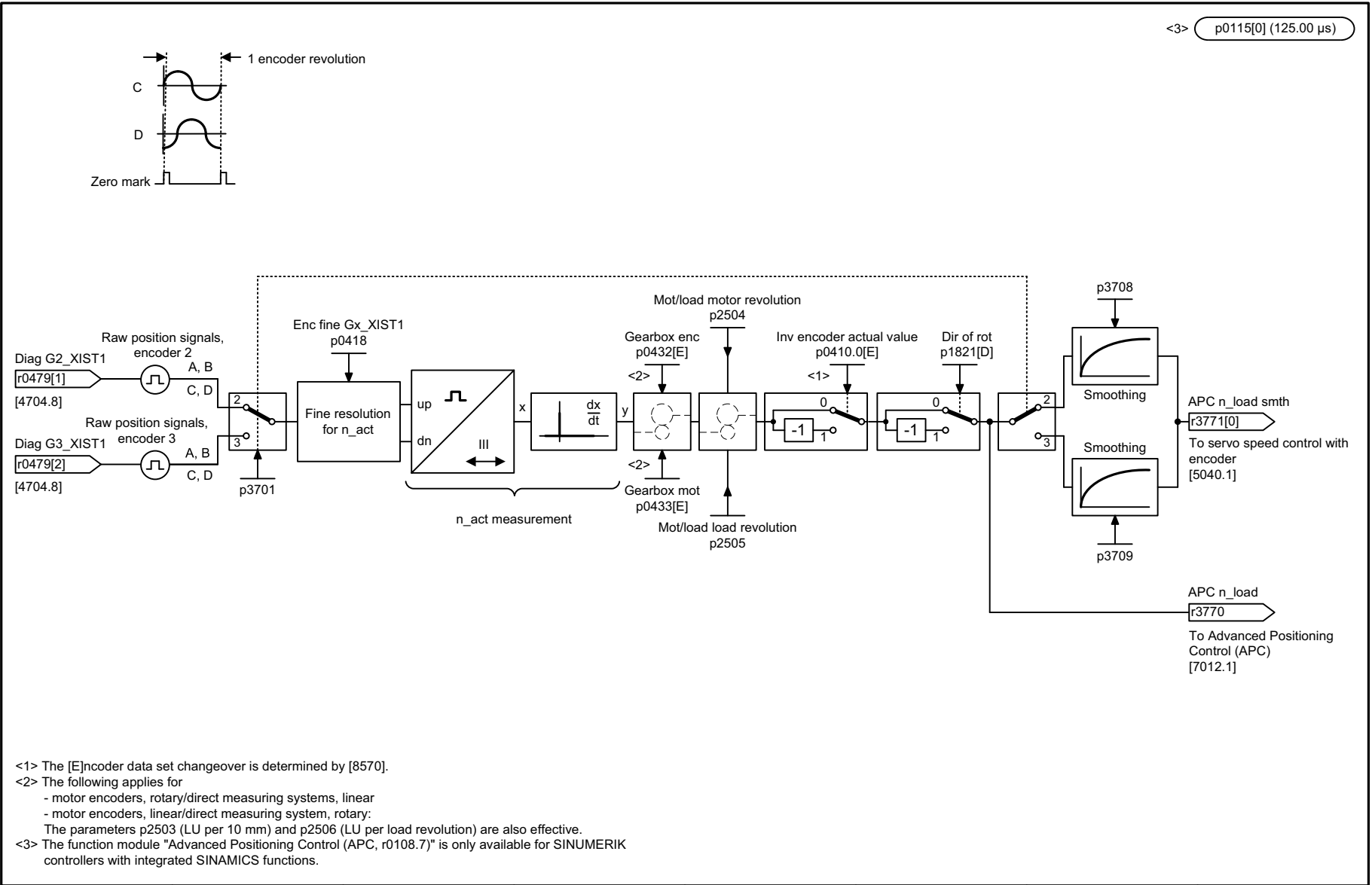
Fig. 3-191 4711 – Speed actual value sensing encoders 2, 3 (r0108.7 = 1, APC activated)
