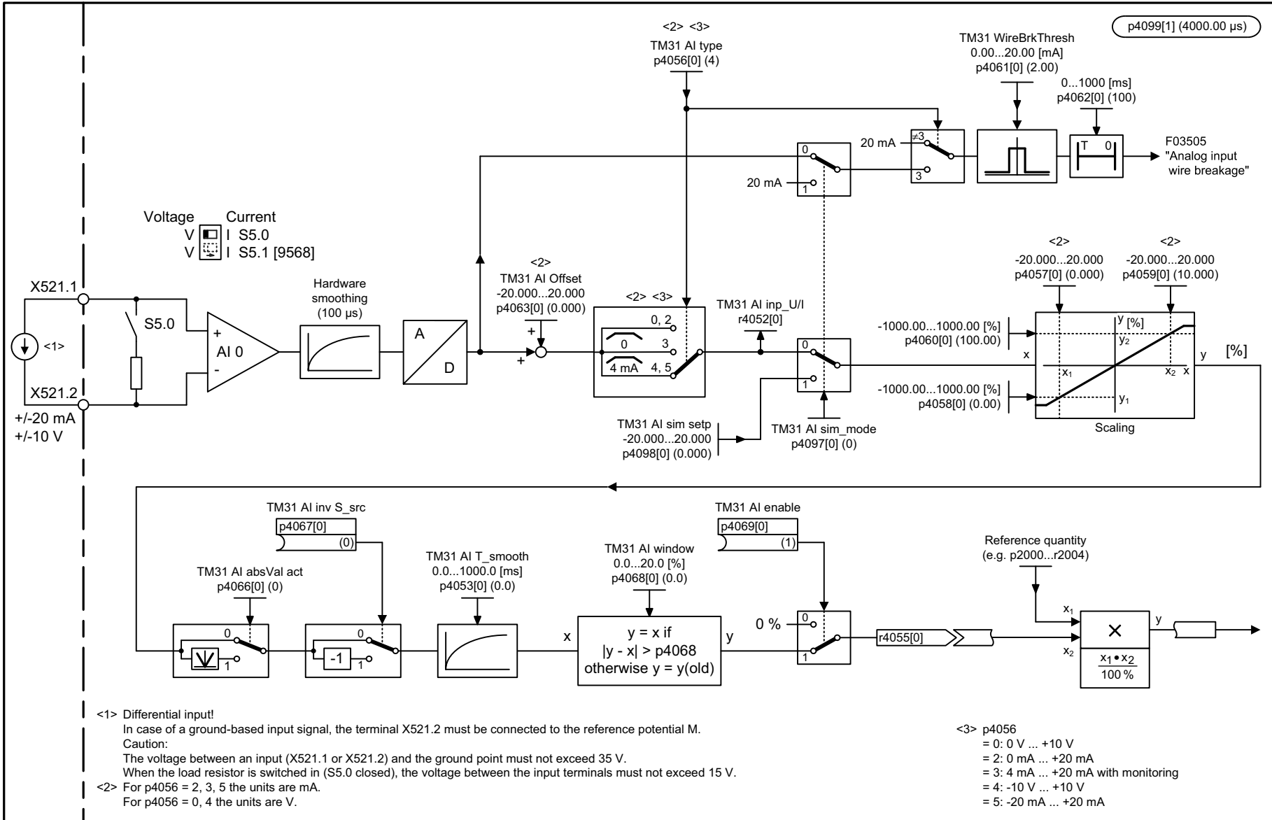
Fig. 3-379 9566 – Analog input 0 (AI 0)
