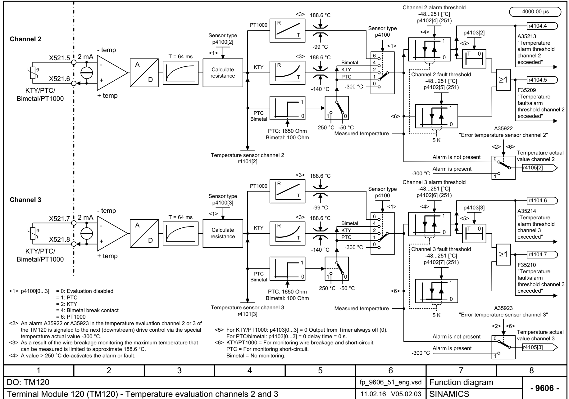
Fig. 3-385 9606 – Temperature evaluation channels 2 and 3
