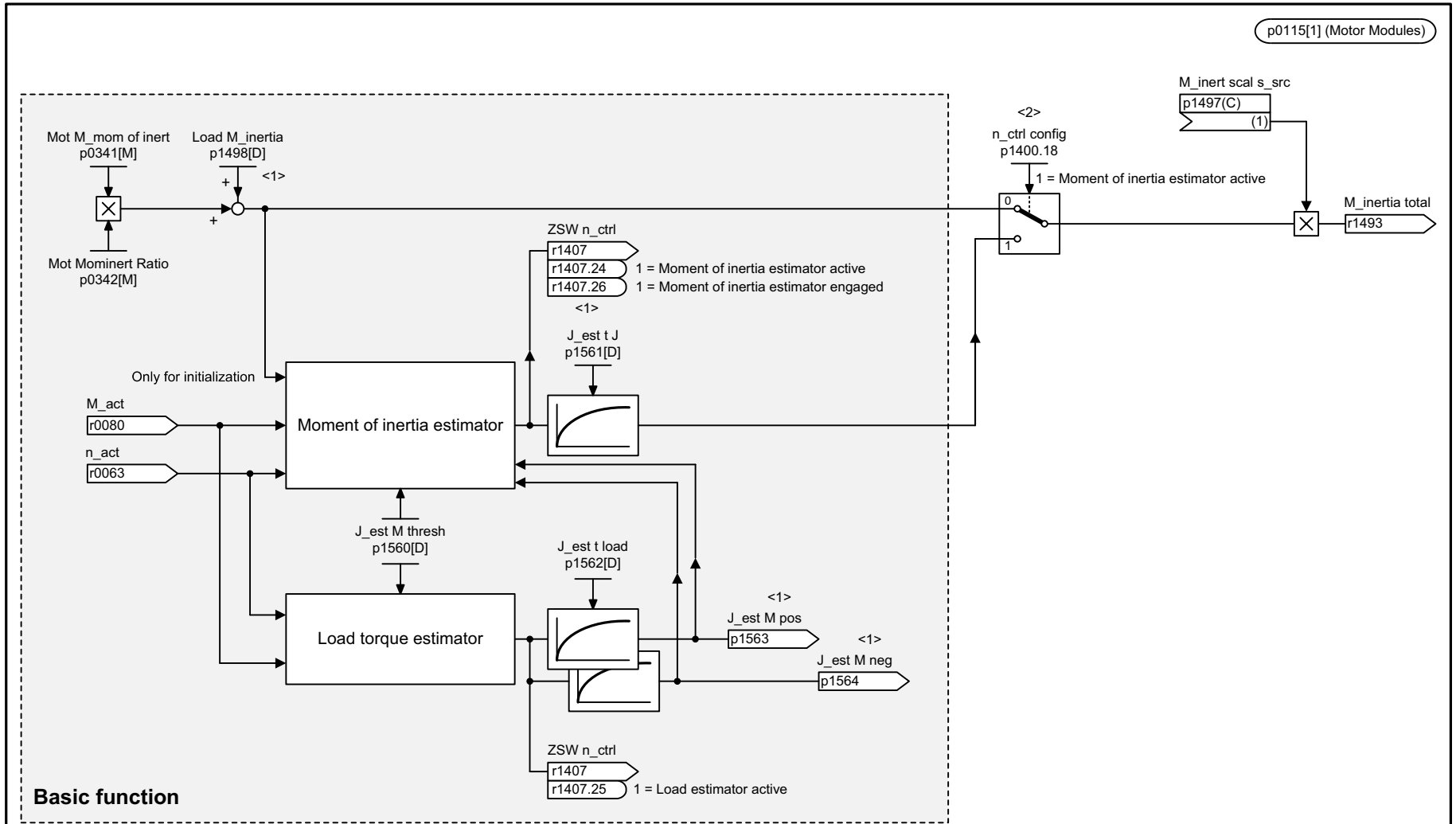
Fig. 3-210 5035 – Moment of inertia estimator (r0108.10 = 1, r0108.30 = 1)
