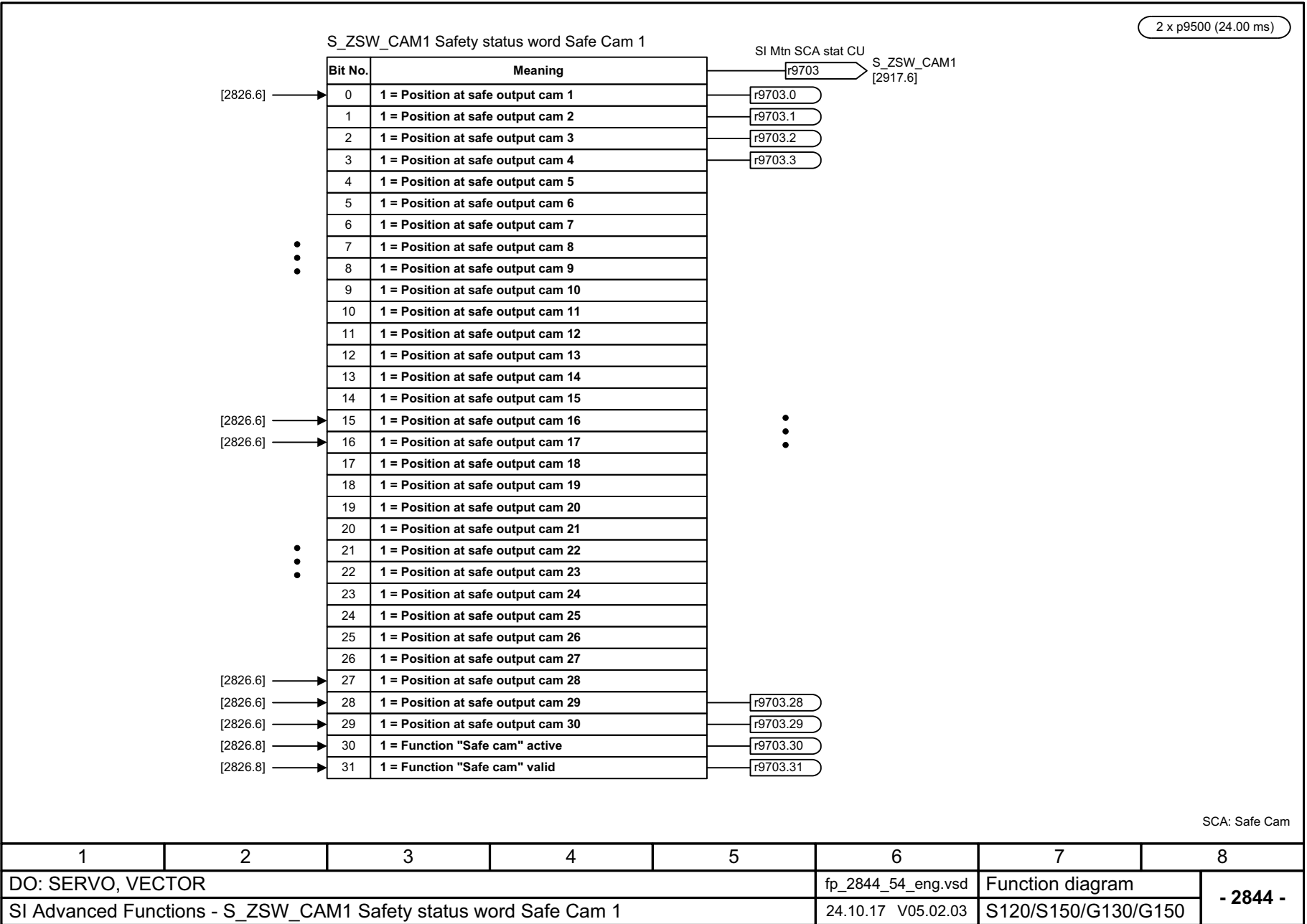
Fig. 3-141 2844 – S_ZSW_CAM1 Safety status word Safe Cam 1
