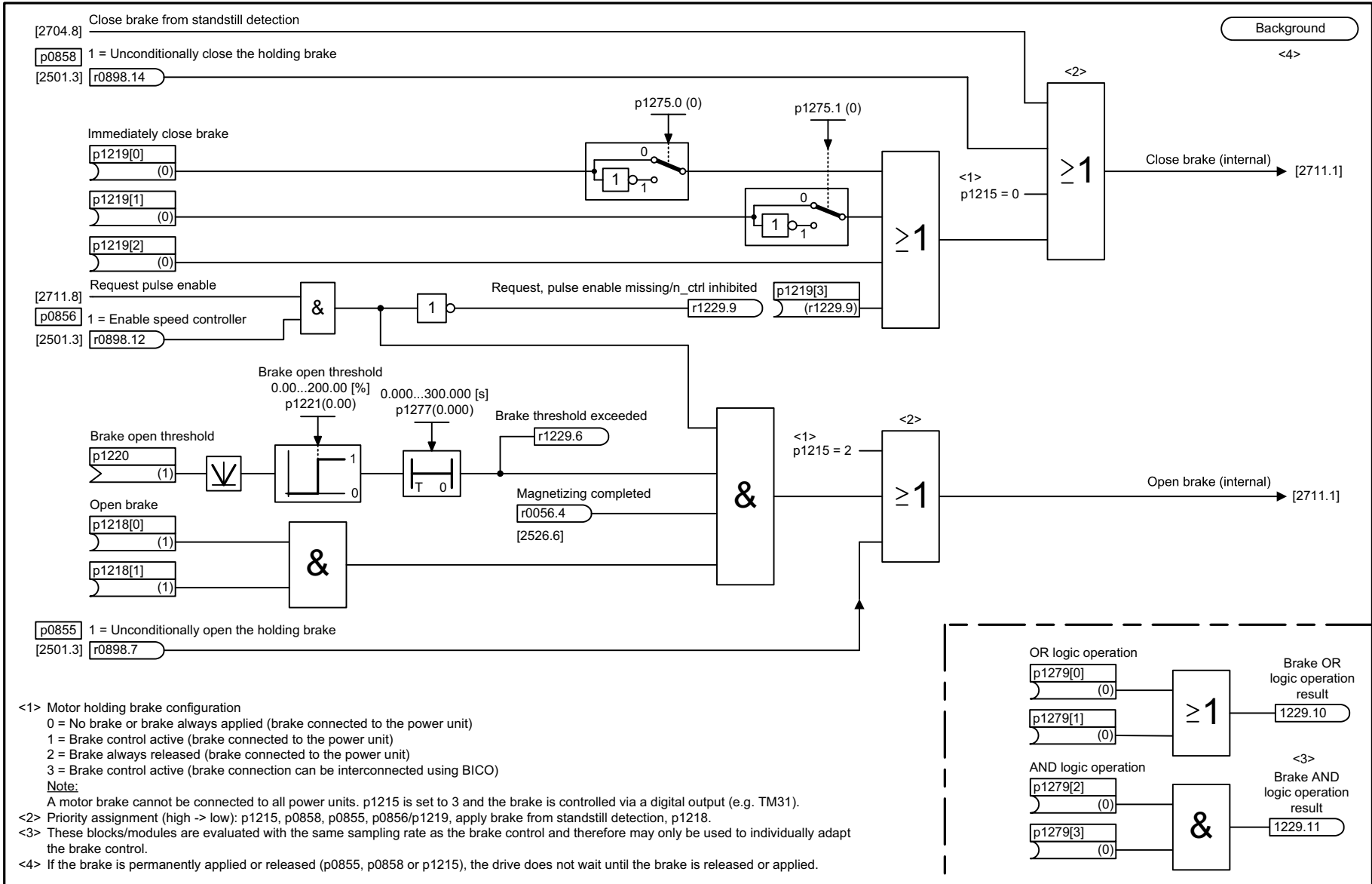
Fig. 3-111 2707 – Extended brake control, open/close brake (r0108.14 = 1)
