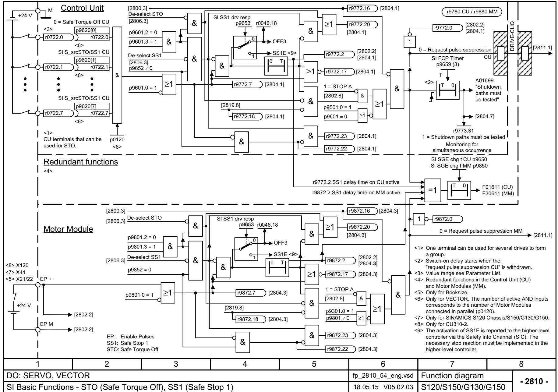
Fig. 3-117 2810 - STO (Safe Torque Off), SS1 (Safe Stop 1)
