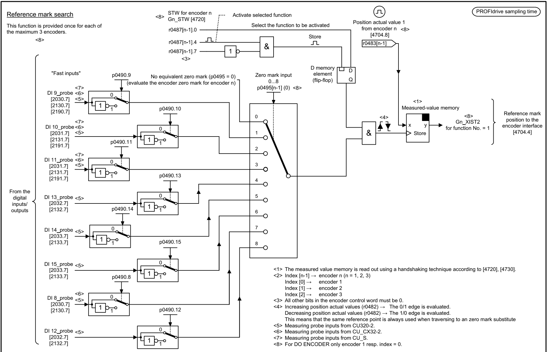
Fig. 3-195 4735 – Reference mark search with external zero mark; encoders 1 ... 3
