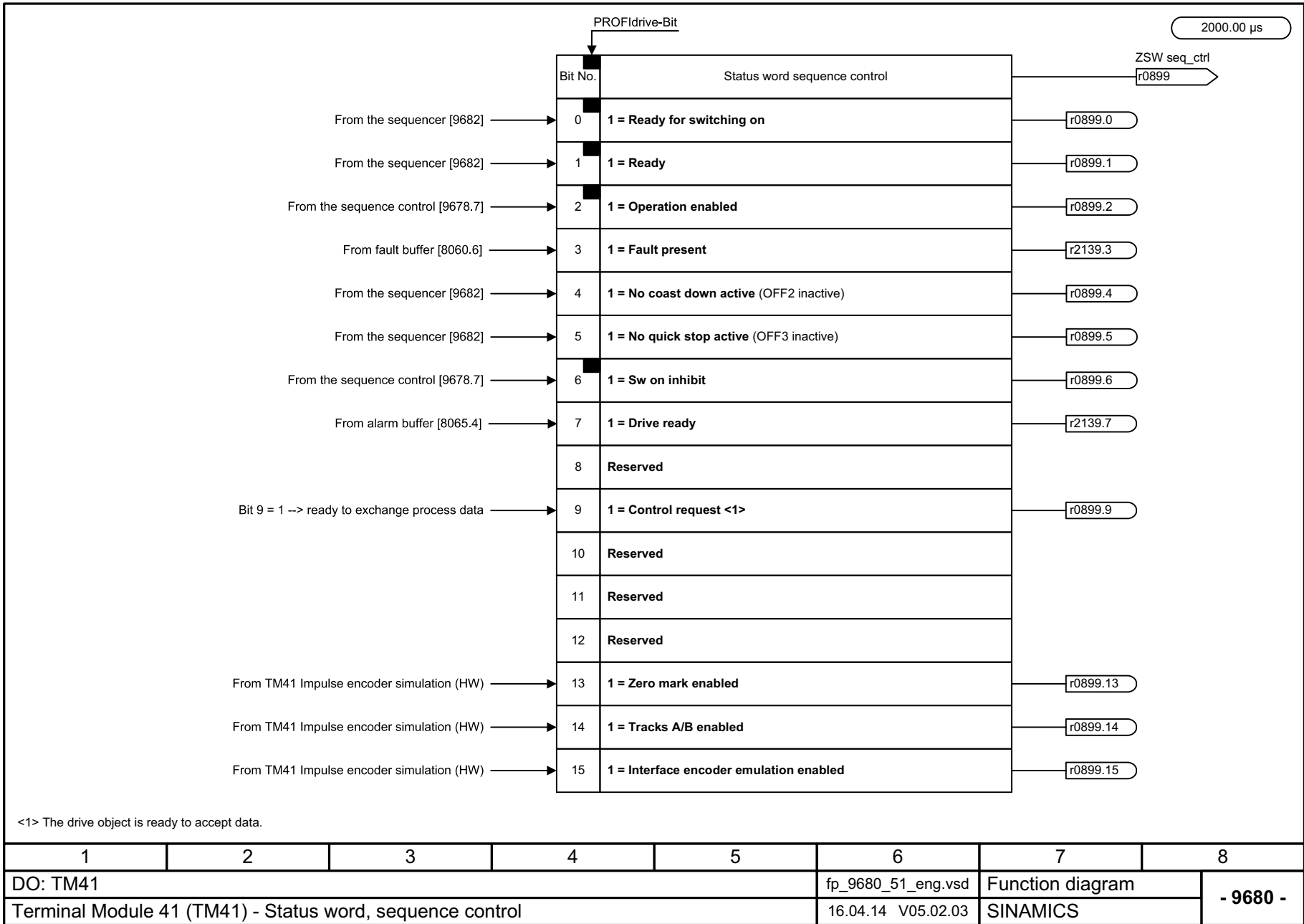
Fig. 3-399 9680 – Status word sequence control
