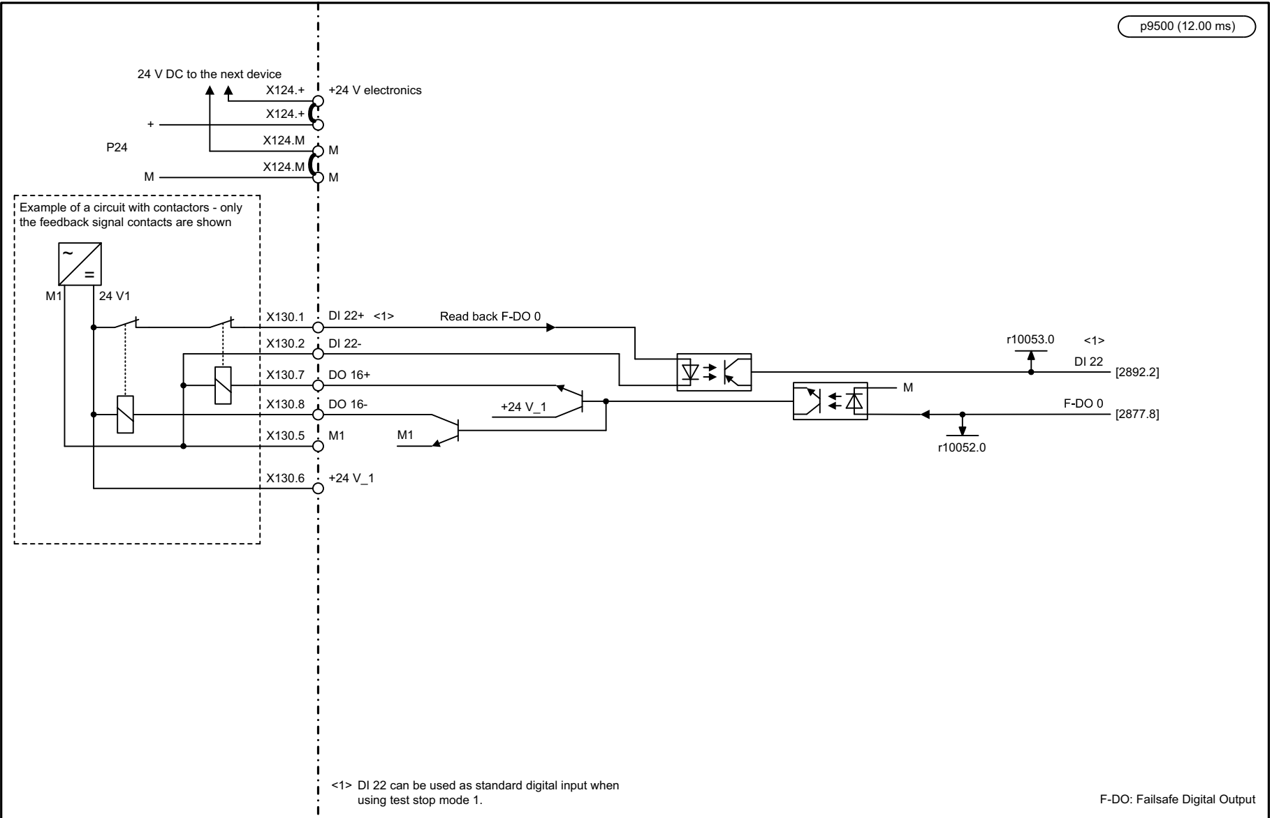
Fig. 3-135 2873 – CU310-2 Failsafe Digital Output (F-DO 0)
