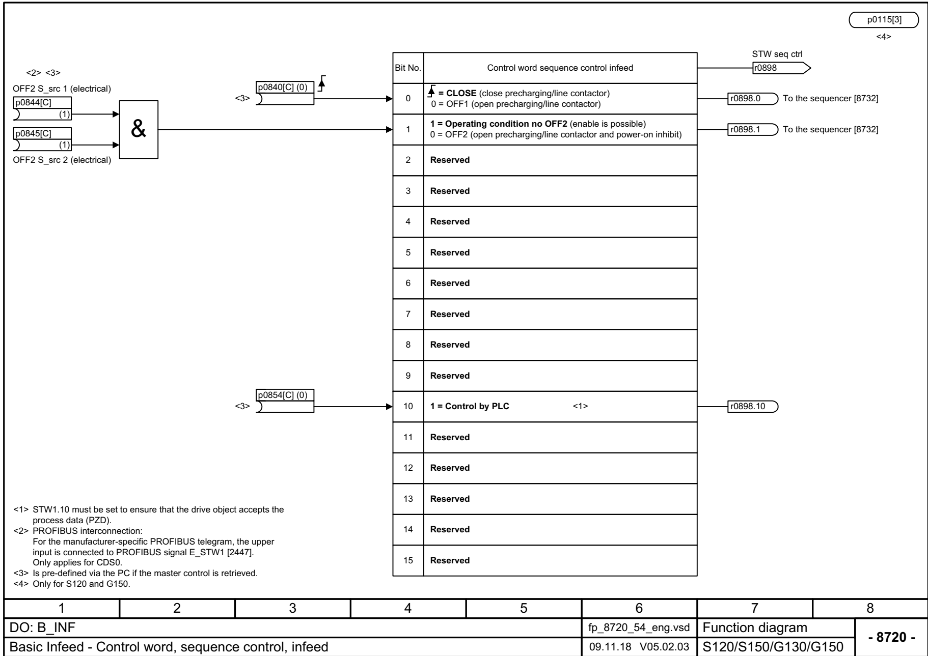
Fig. 3-327 8720 – Control word sequence control infeed
