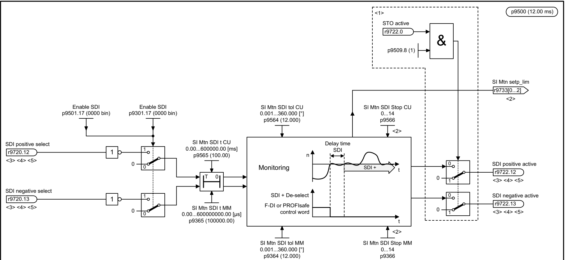
Fig. 3-125 2824 – SDI (Safe Direction)
