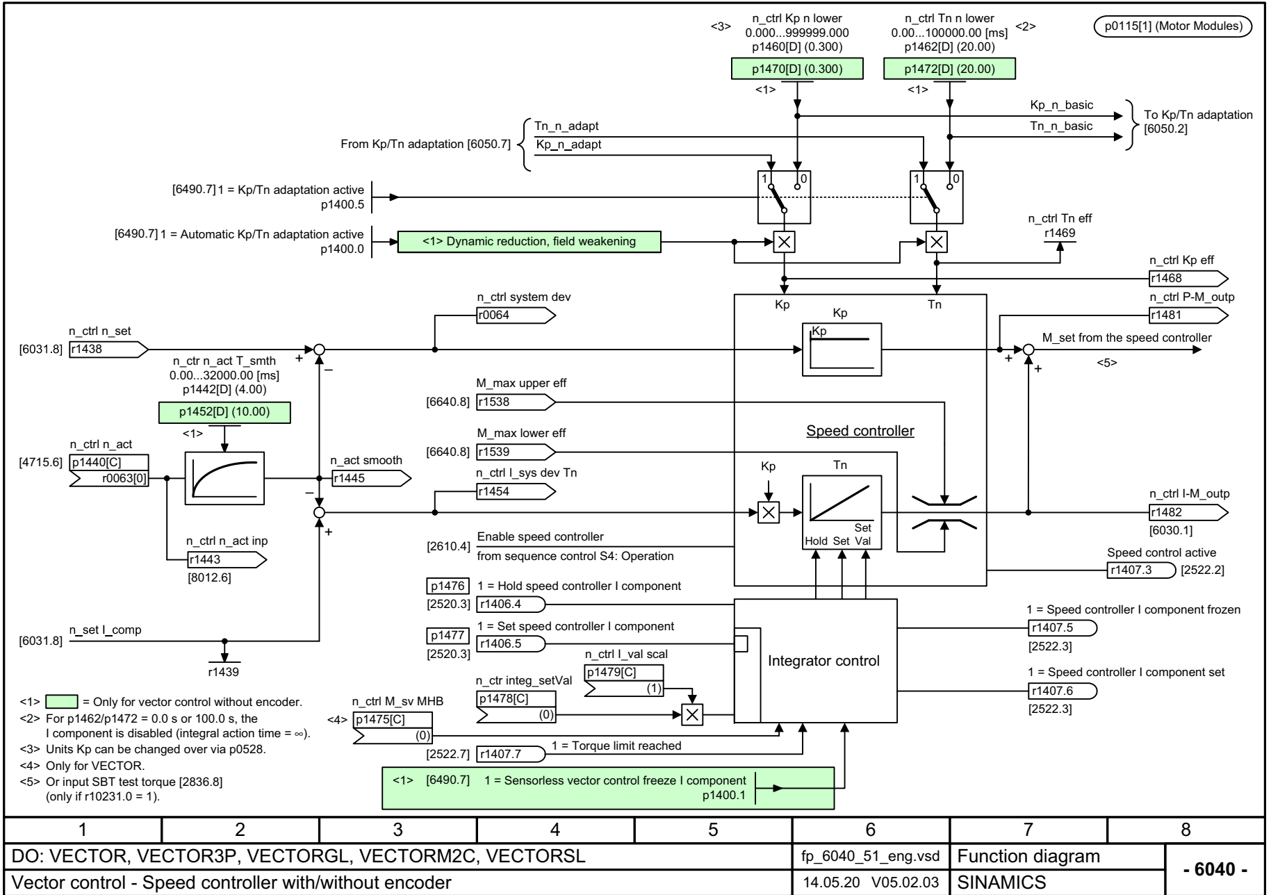
Fig. 3-237 6040 – Speed controller with/without encoder
