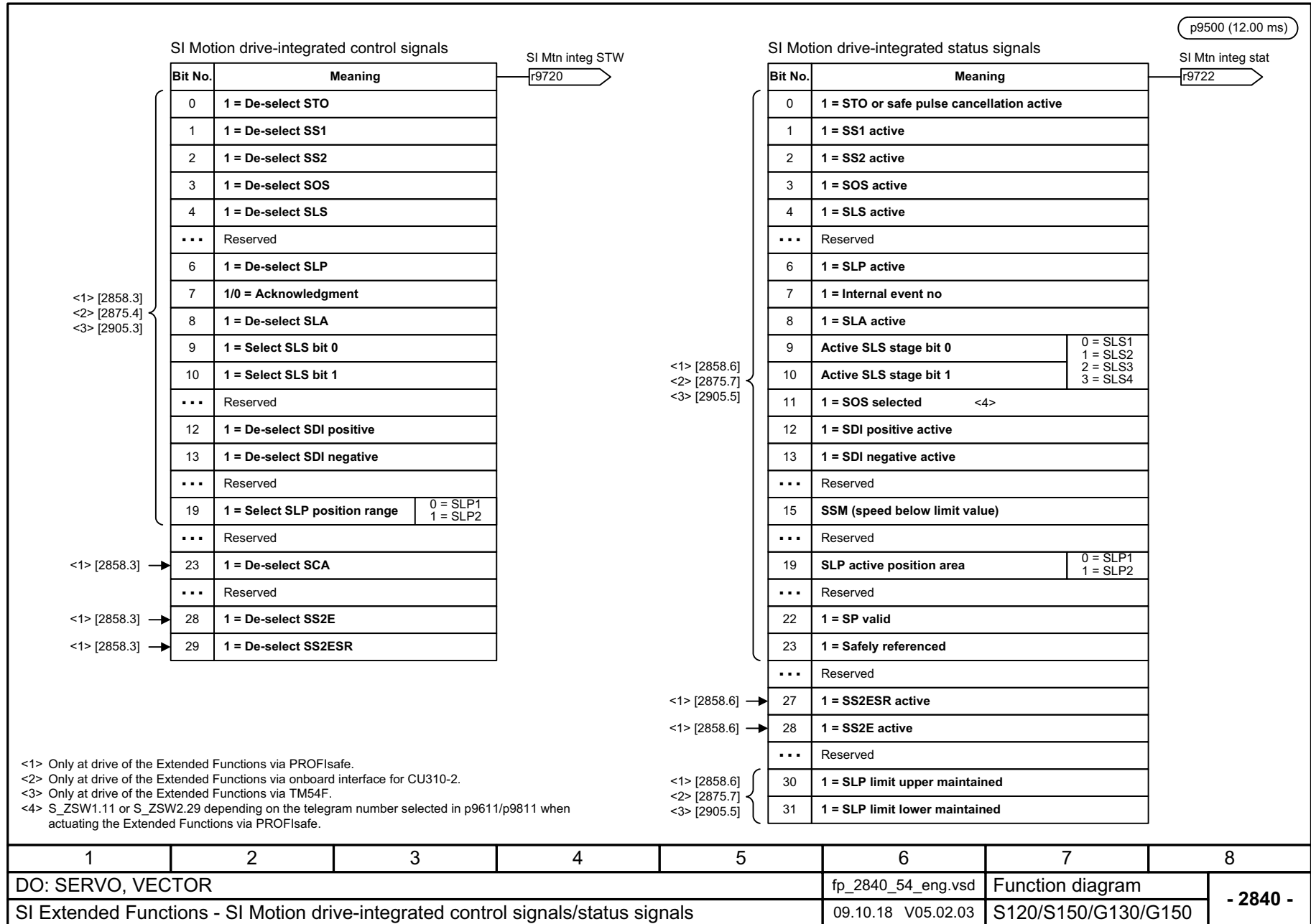
Fig. 3-130 2840 – SI Motion drive-integrated control signals / status signals
