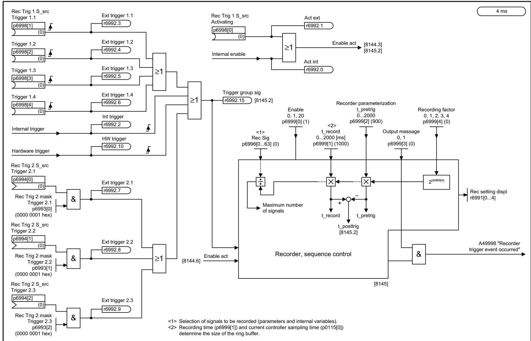
Fig. 3-319 8144 – Recorder overview (r0108.5 = 1)
