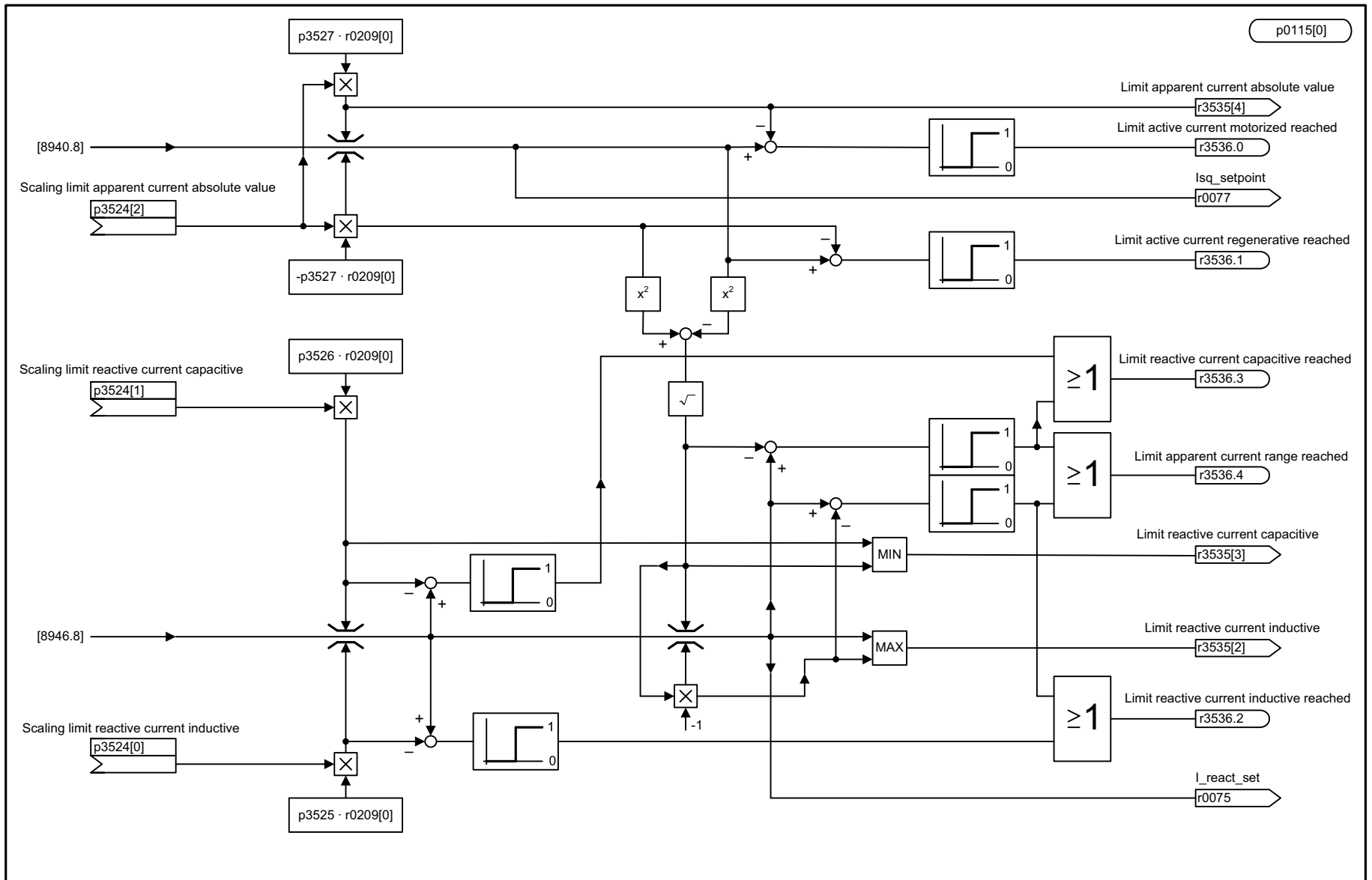
Fig. 3-349 8945 - Reactive current/apparent current limits (r0108.3 = 1)
