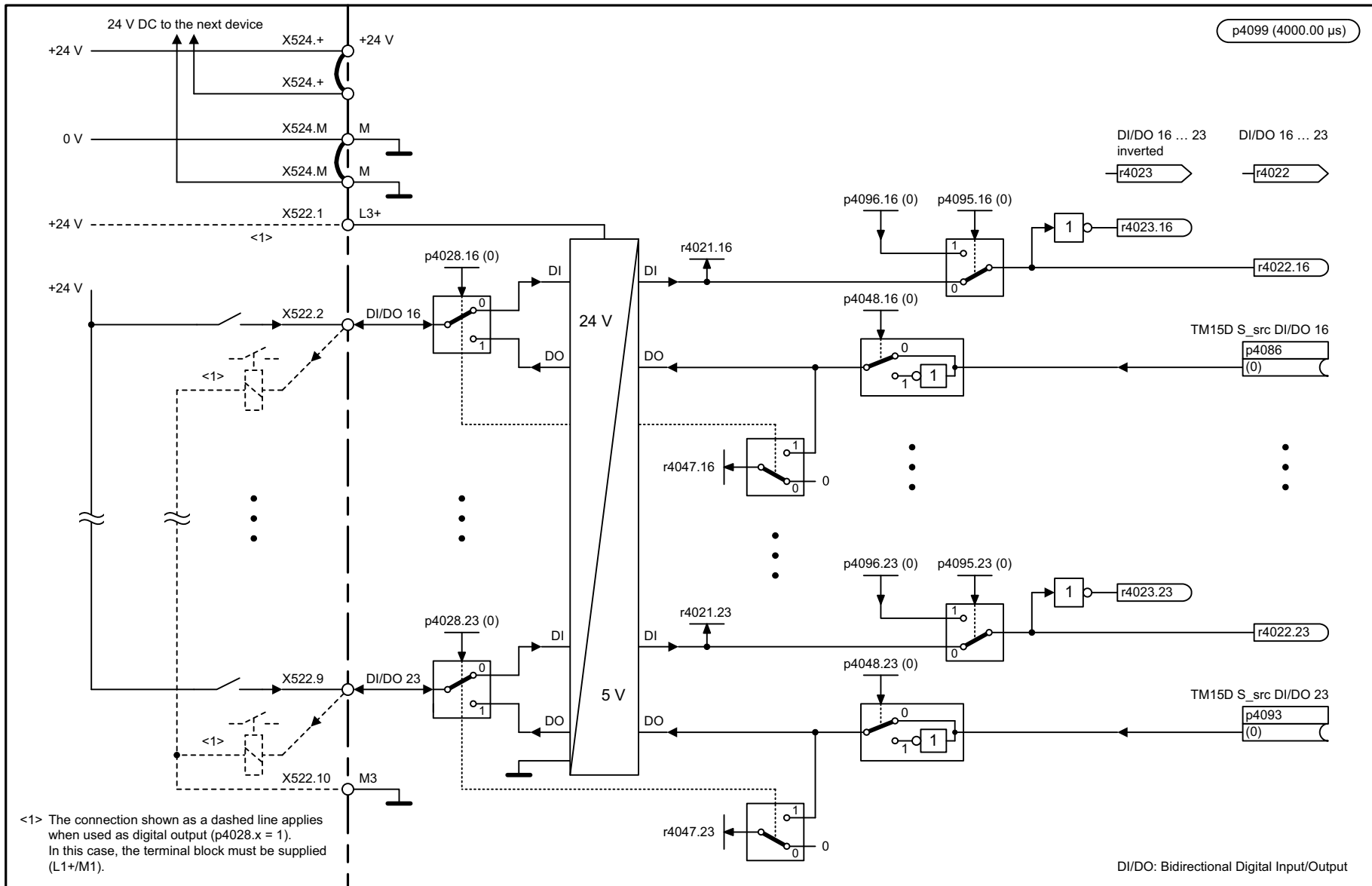
Fig. 3-371 9402 – Digital inputs/outputs bidirectional (DI/DO 16 ... DI/DO 23)
