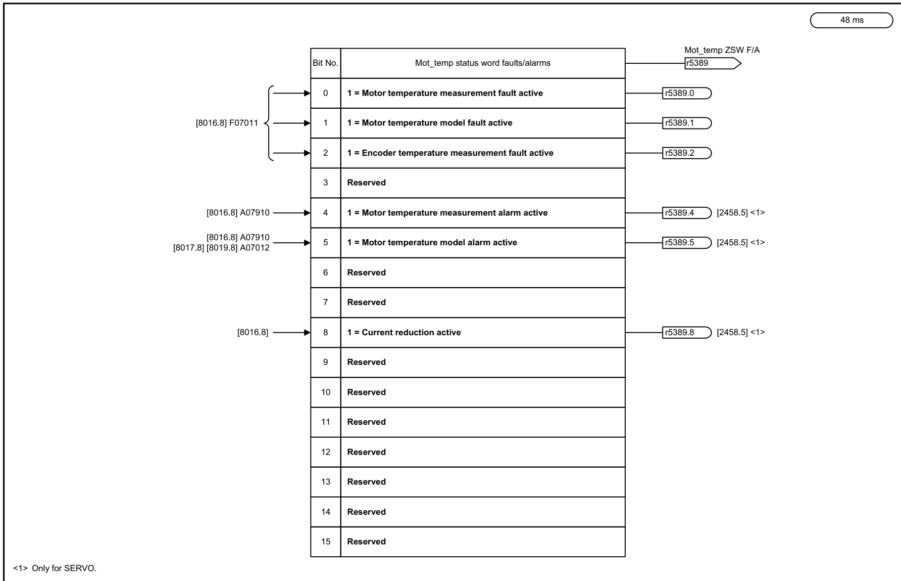
Fig. 3-305 8015 – Motor temperature status word faults/alarms
