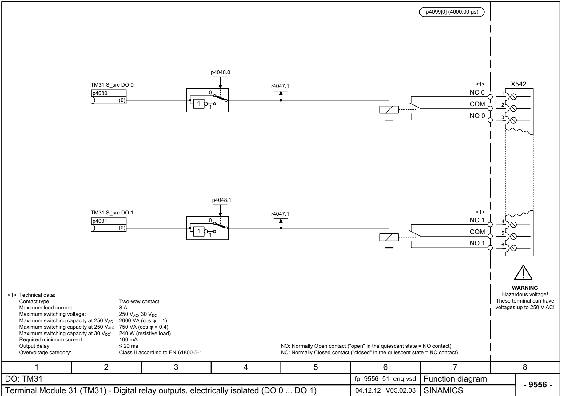
Fig. 3-376 9556 – Digital relay outputs electrically isolated (DO 0 ... DO 1)
