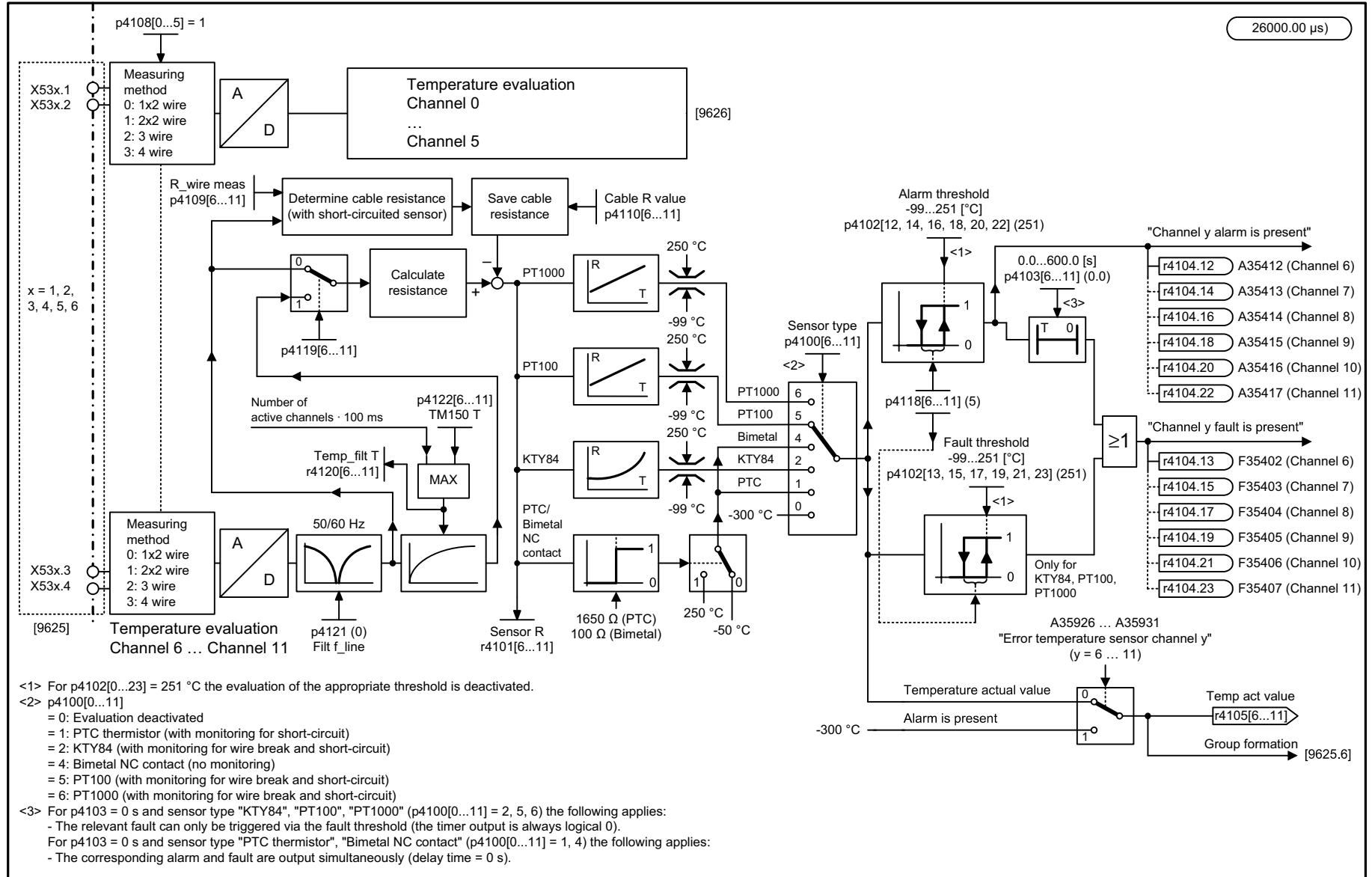
Fig. 3-388 9627 – Temperature evaluation 2x2 wire (channels 0 ... 11)
