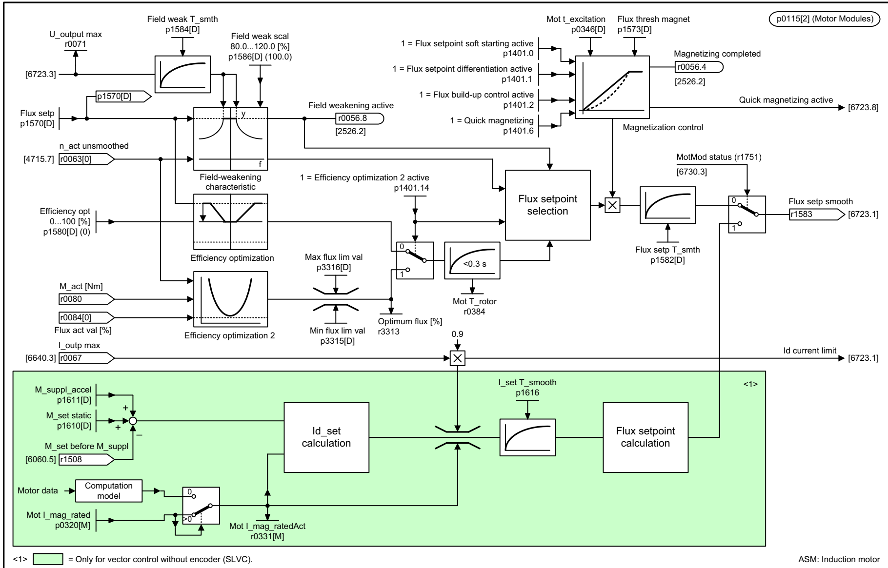
Fig. 3-254 6722 – Field weakening characteristic, Id setpoint (ASM, p0300 = 1)
