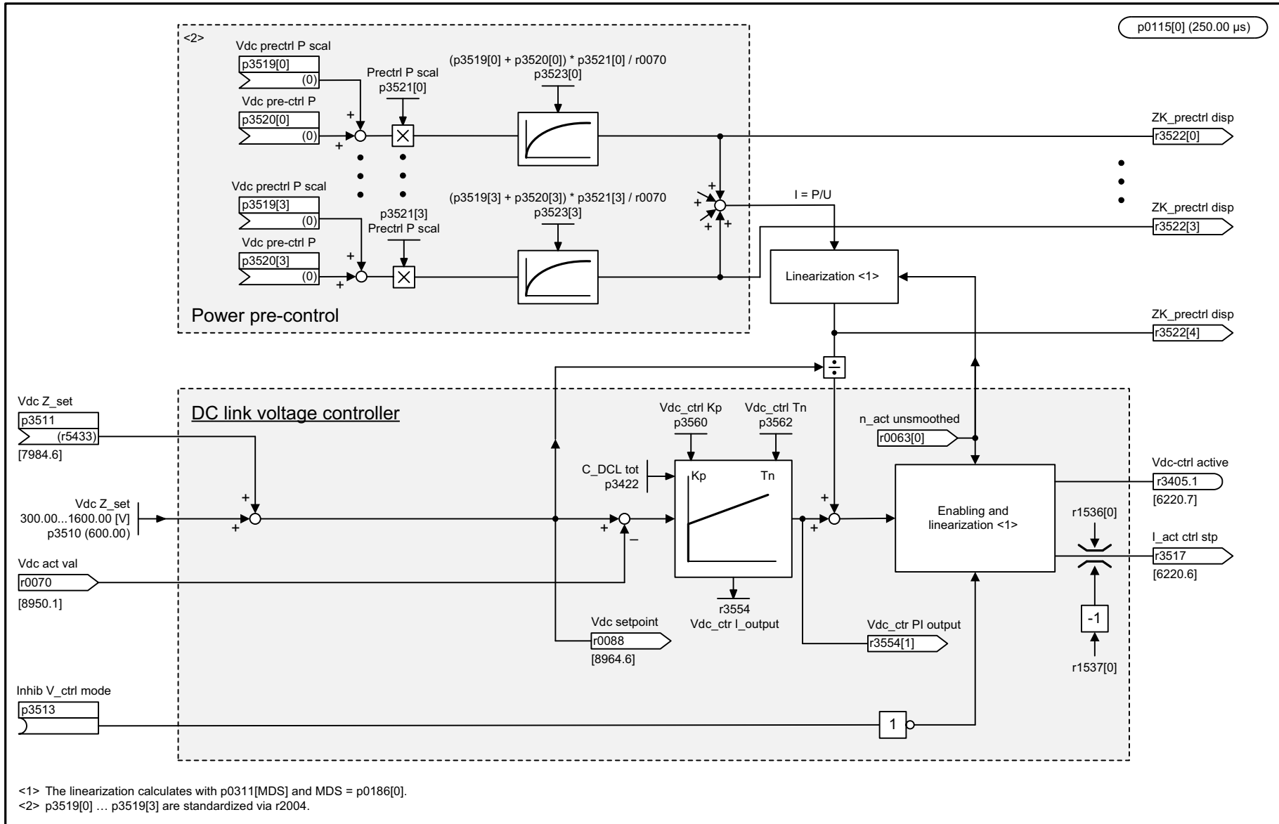
Fig. 3-282 7960 – DC-link voltage controller (r0108;16 = 1)
