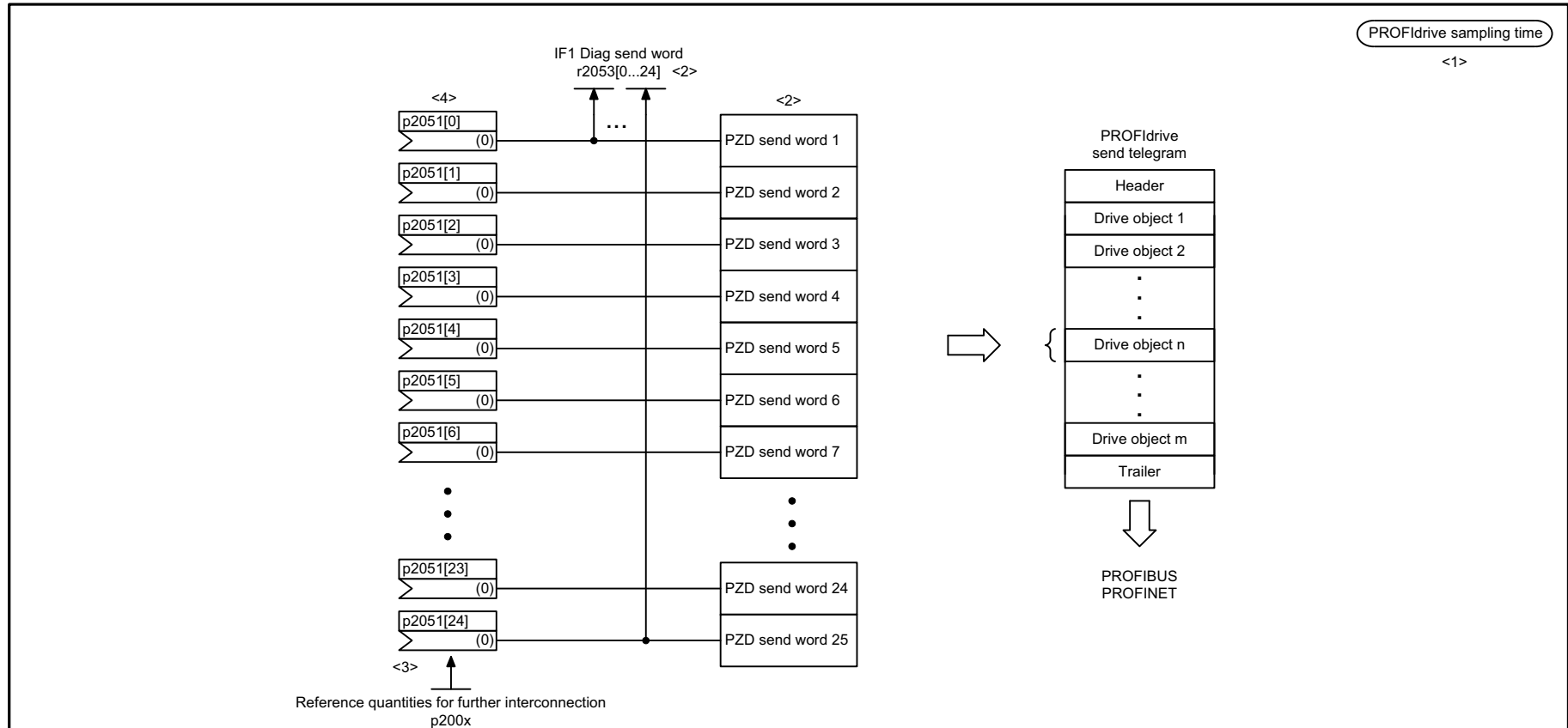
Fig. 3-83 2483 – IF1 send telegram free interconnection via BICO (p0922 = 999)
