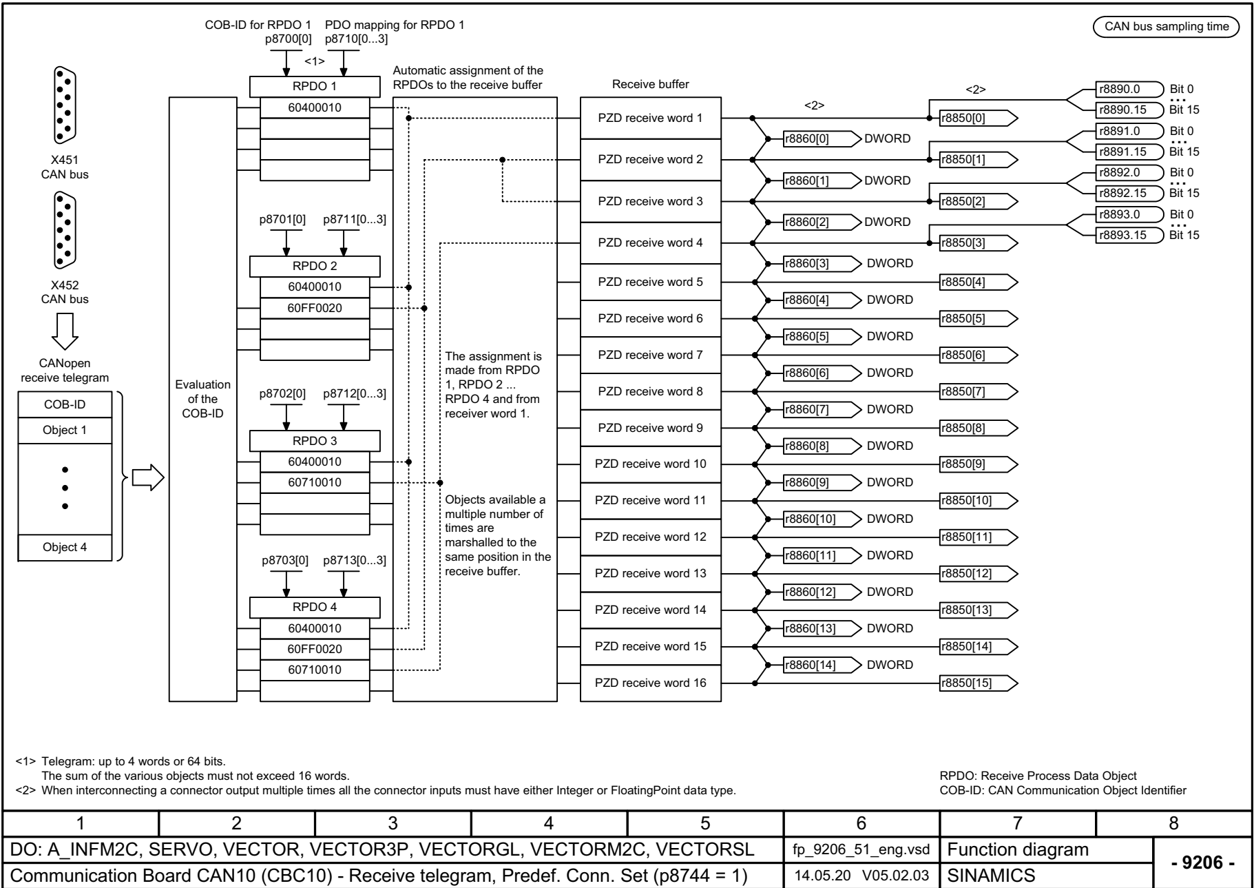
Fig. 3-362 9206 – Receive telegram Predefined Connection Set (p8744 = 1)
