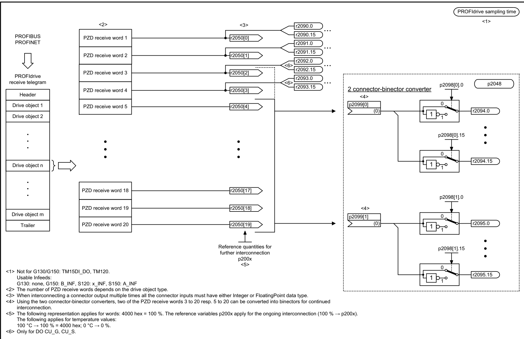
Fig. 3-82 2481 – IF1 receive telegram free interconnection via BICO (p0922 = 999)
