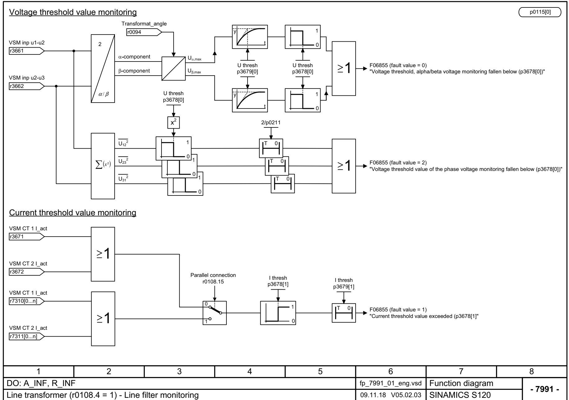
Fig. 3-292 7991 – Line filter monitoring
