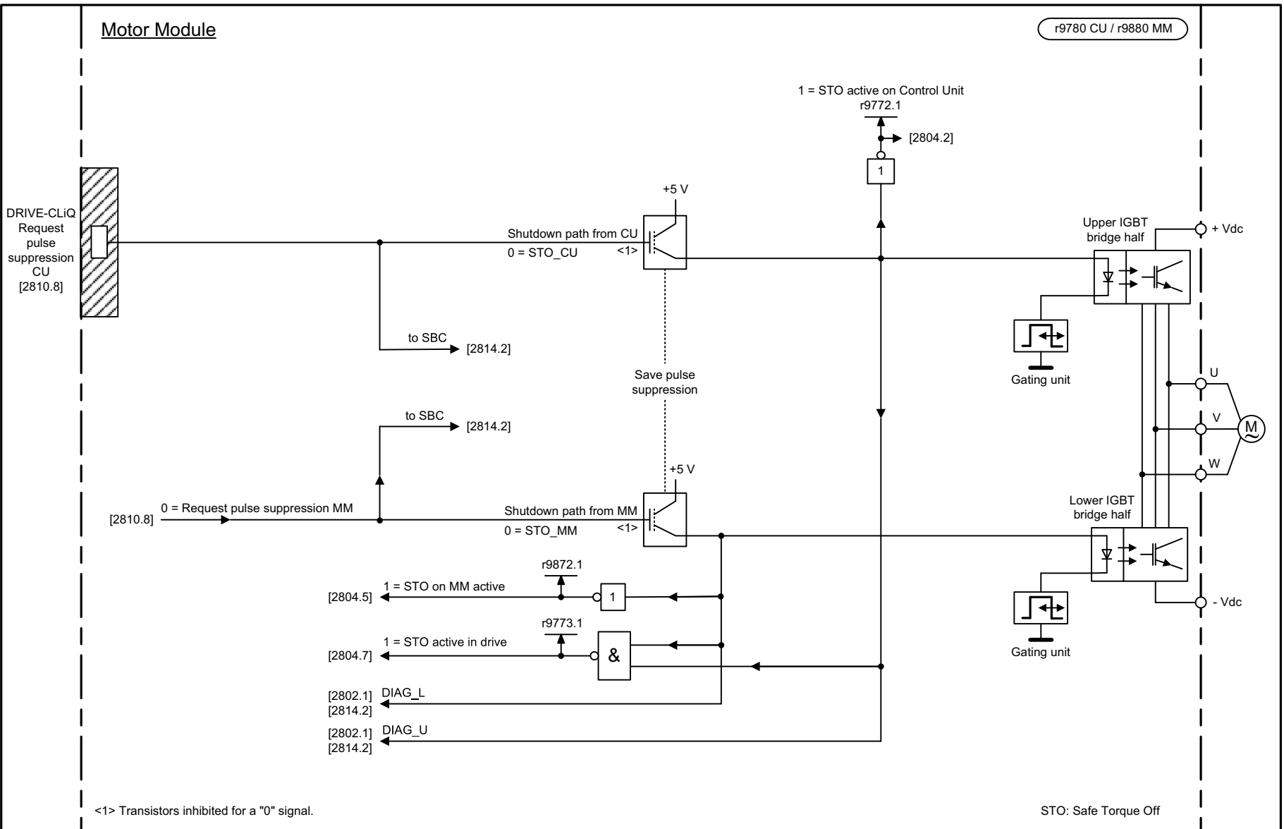
Fig. 3-118 2811 – STO (Safe Torque Off), safe pulse suppression
