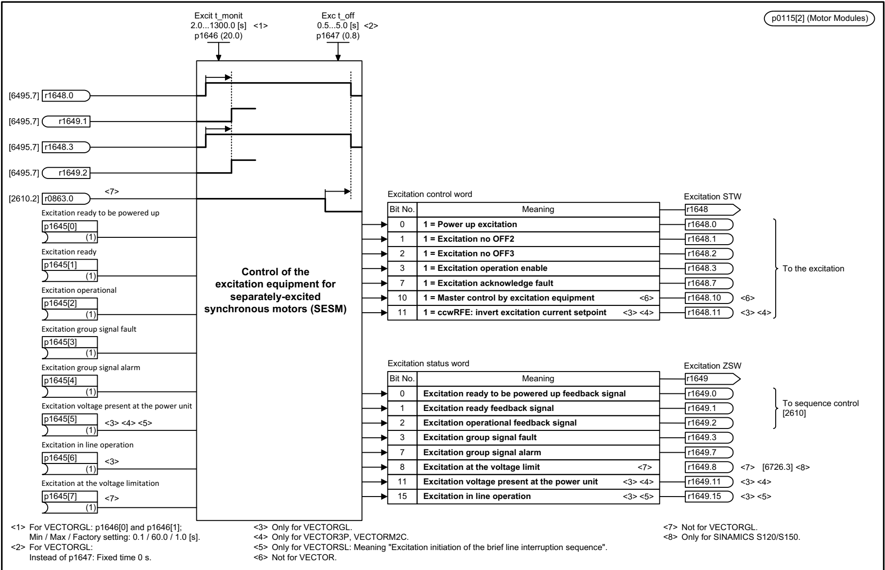
Fig. 3-247 6495 – Excitation (SESM, p0300 = 5)
