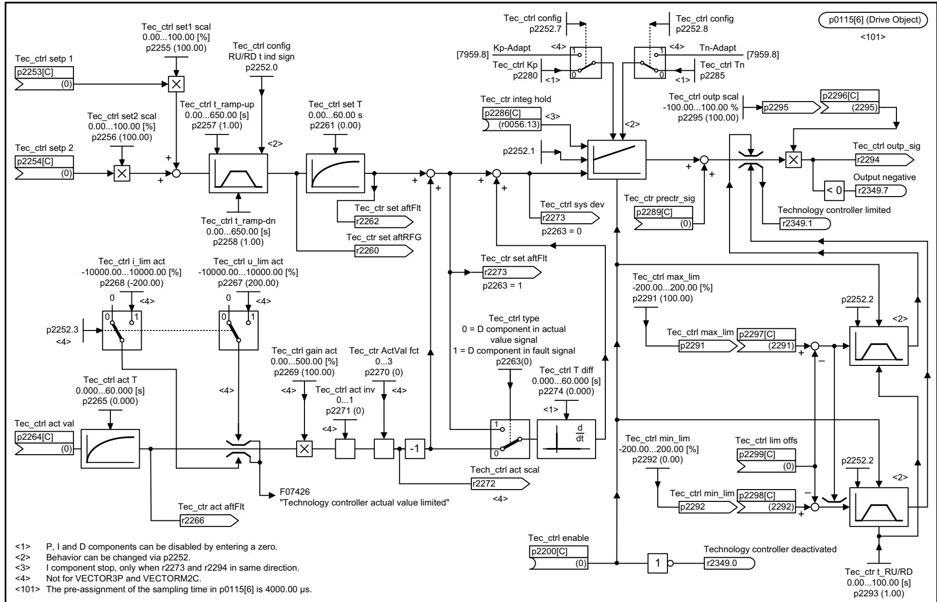
Fig. 3-280 7958 – Closed-loop control (r0108.16 = 1)
