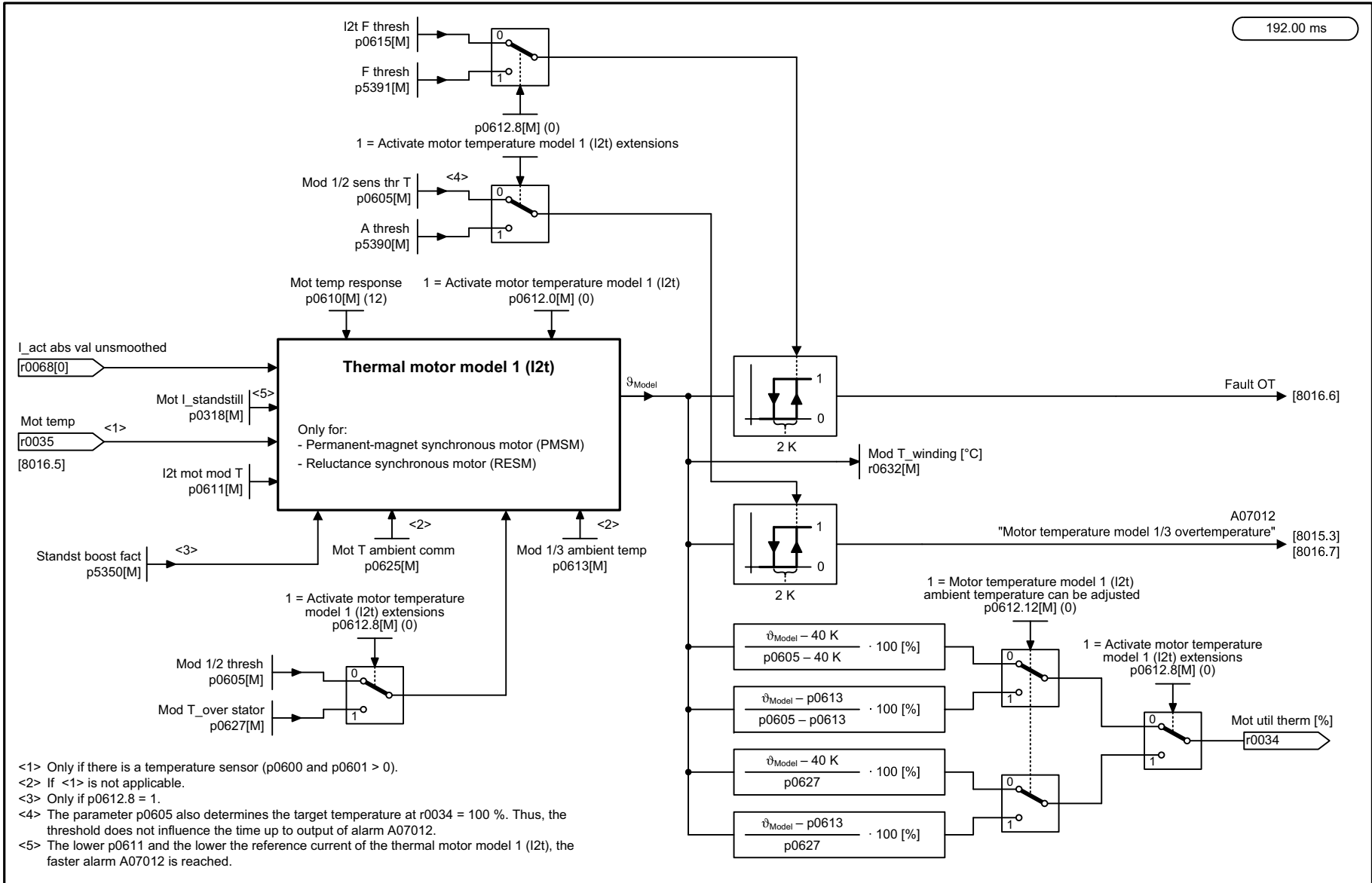
Fig. 3-307 8017 – Motor temperature model 1 (I2t)
