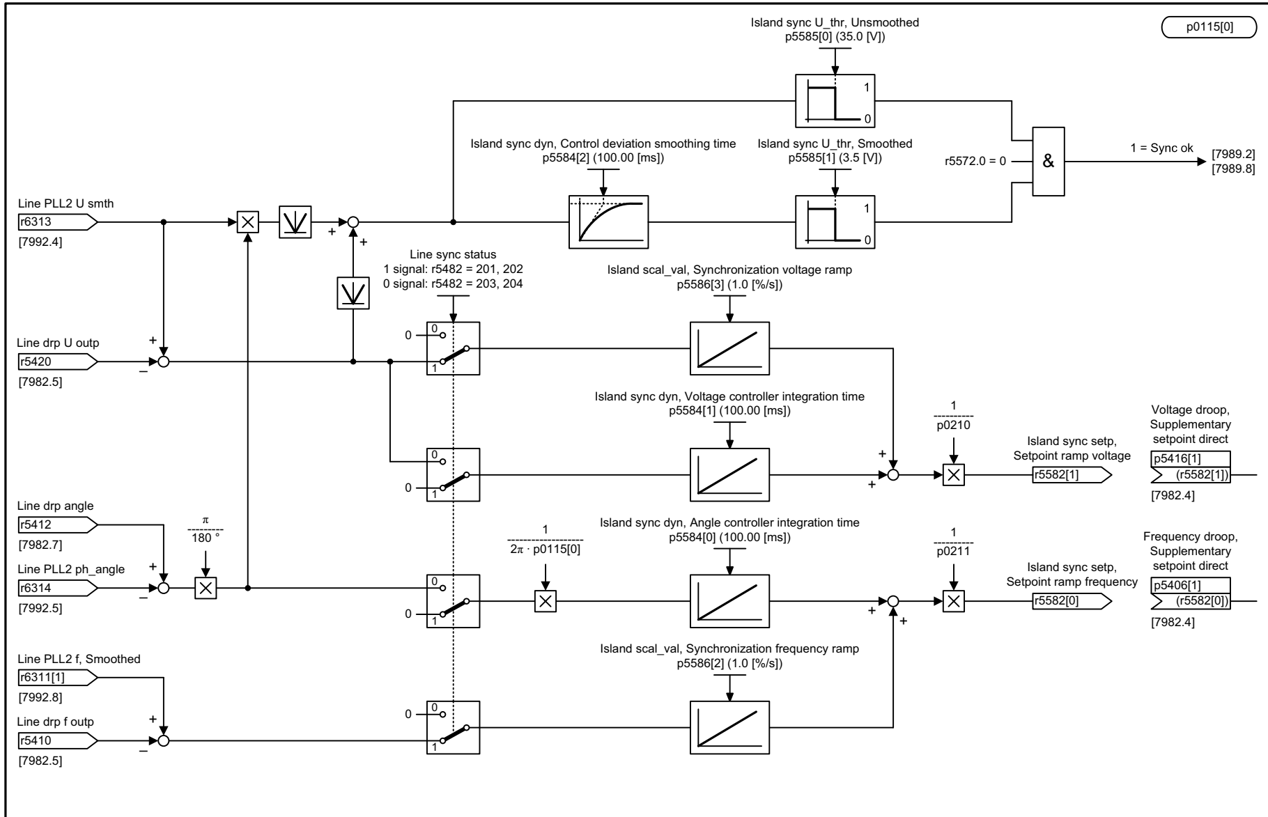
Fig. 3-290 7995 – Island grid synchronization, voltage threshold
