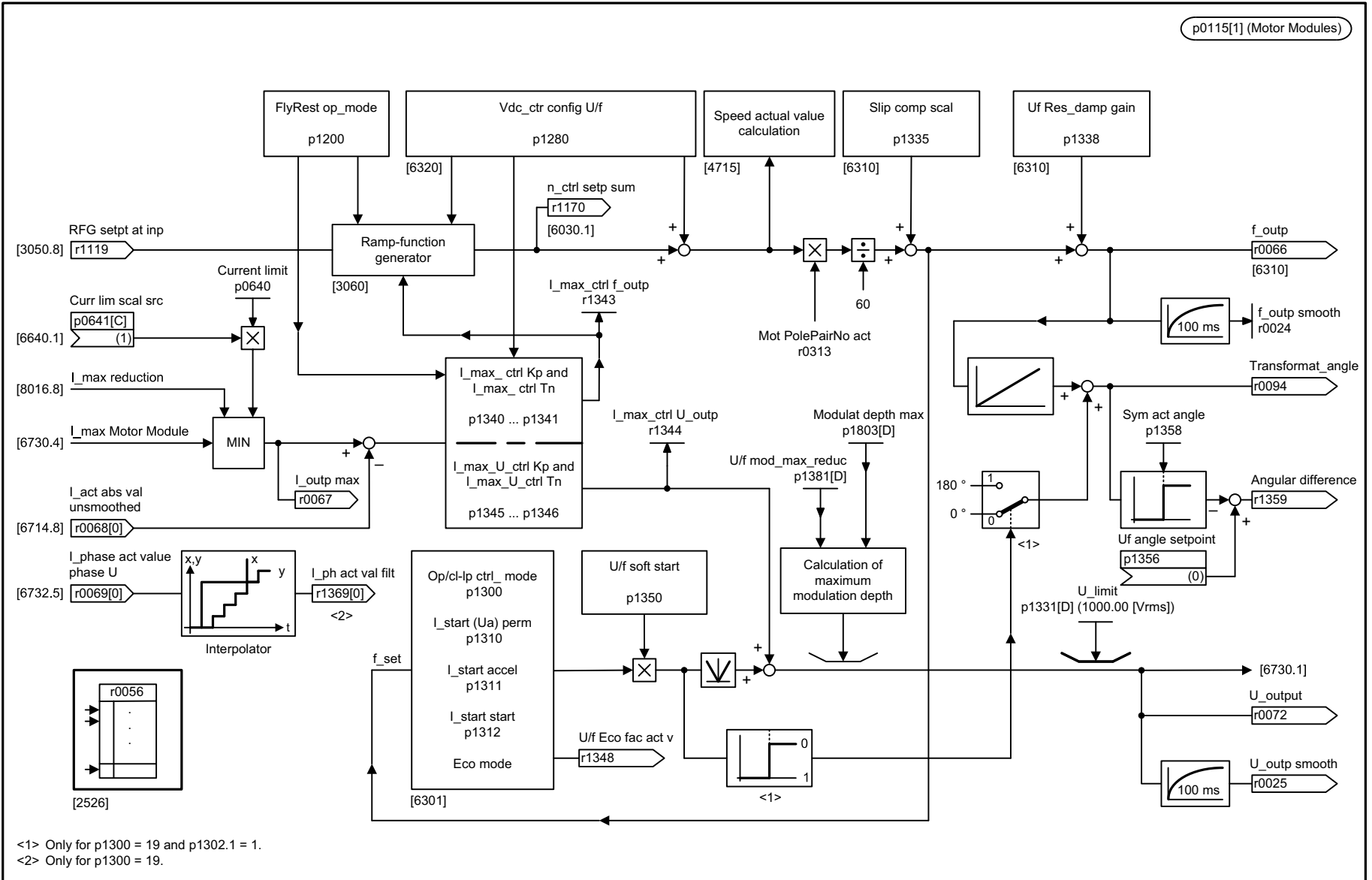
Fig. 3-241 6300 – U/f control, overview
