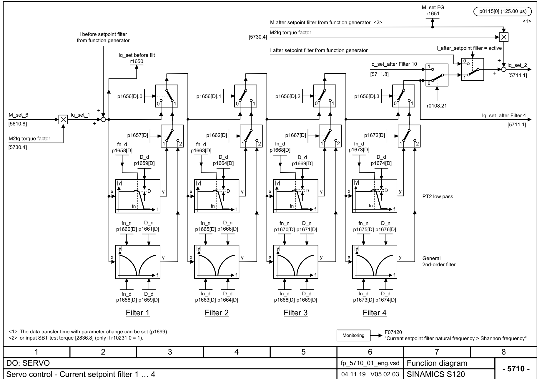
Fig. 3-228 5710 – Current setpoint filter 1 ... 4
