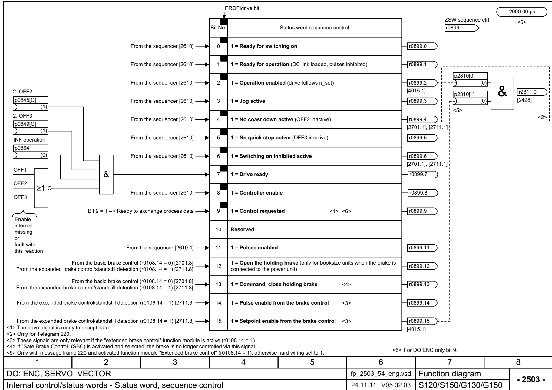
Fig. 3-96 2503 – Status word sequence control
