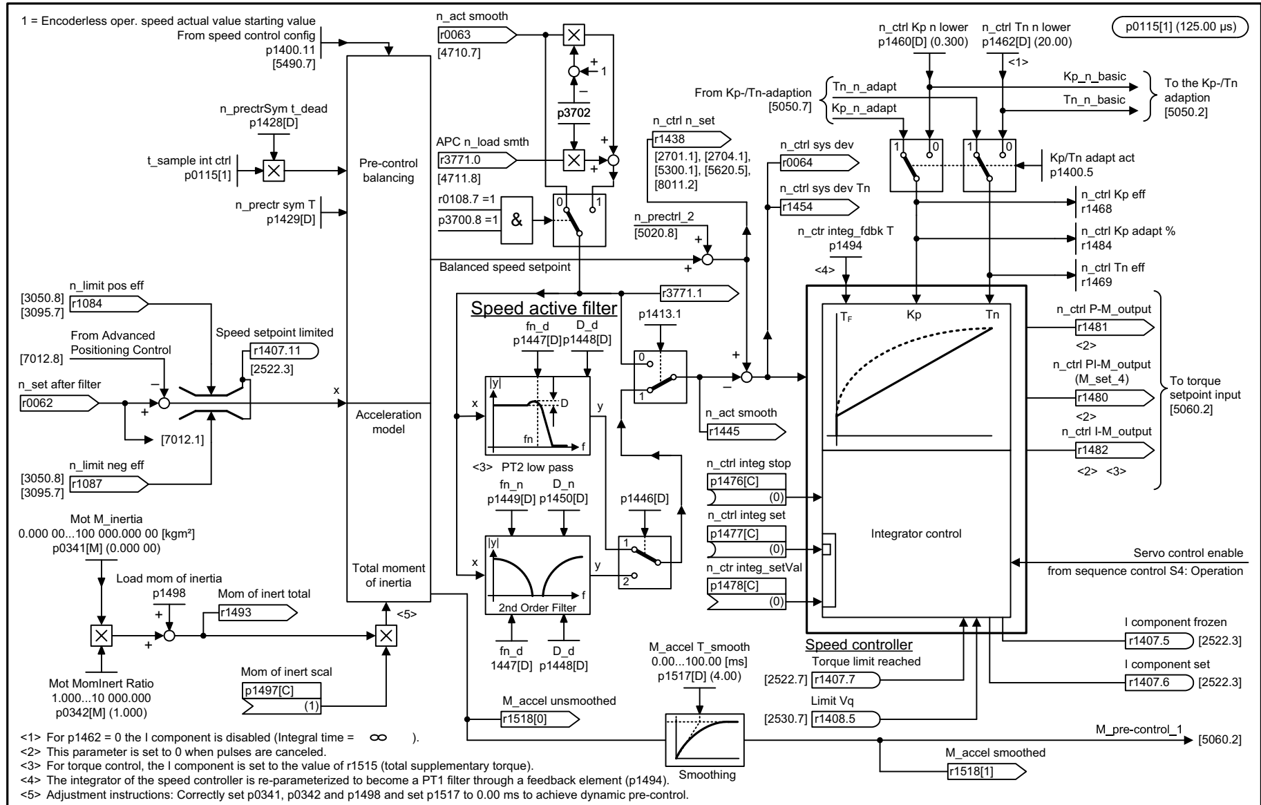
Fig. 3-212 5042 – Speed controller, torque/speed precontrol with encoder (p1402.4 = 1)
