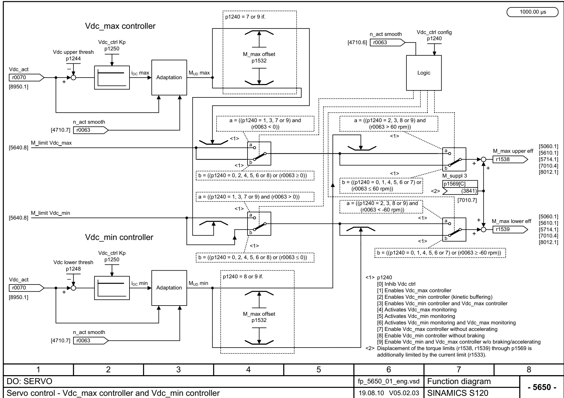
Fig. 3-226 5650 – Vdc_max controller and Vdc_min controller
