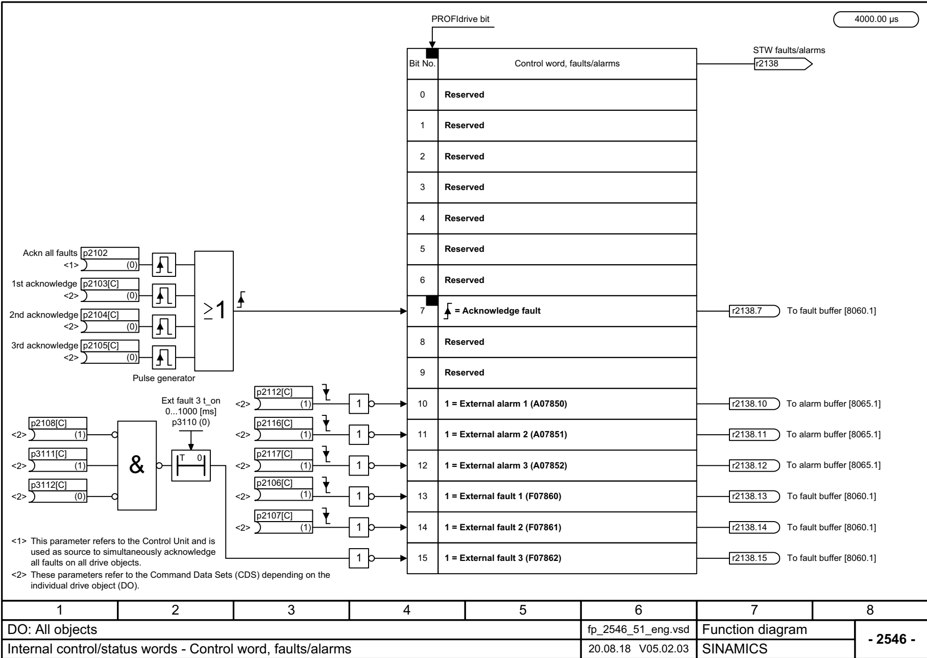
Fig. 3-105 2546 – Control word faults/alarms
