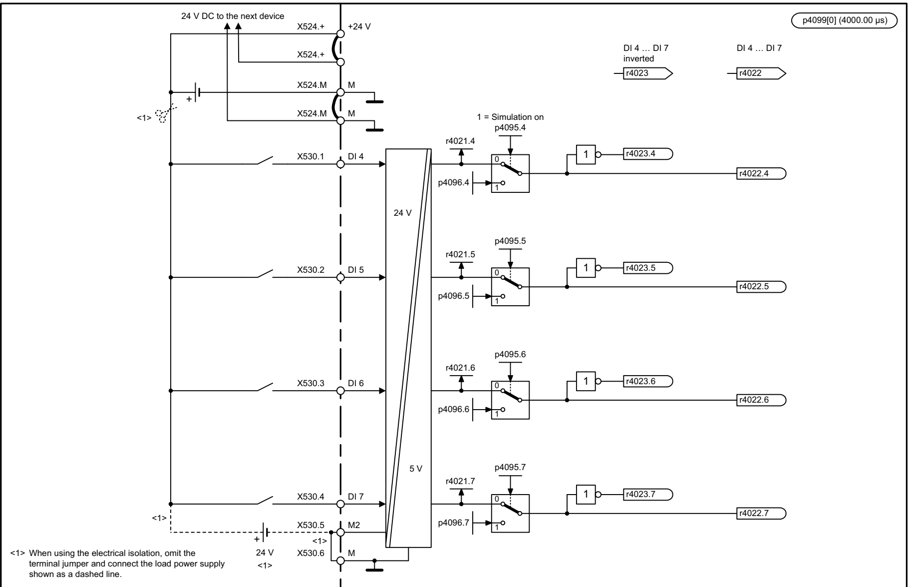
Fig. 3-375 9552 – Digital inputs electrically isolated (DI 4 ... DI 7)
