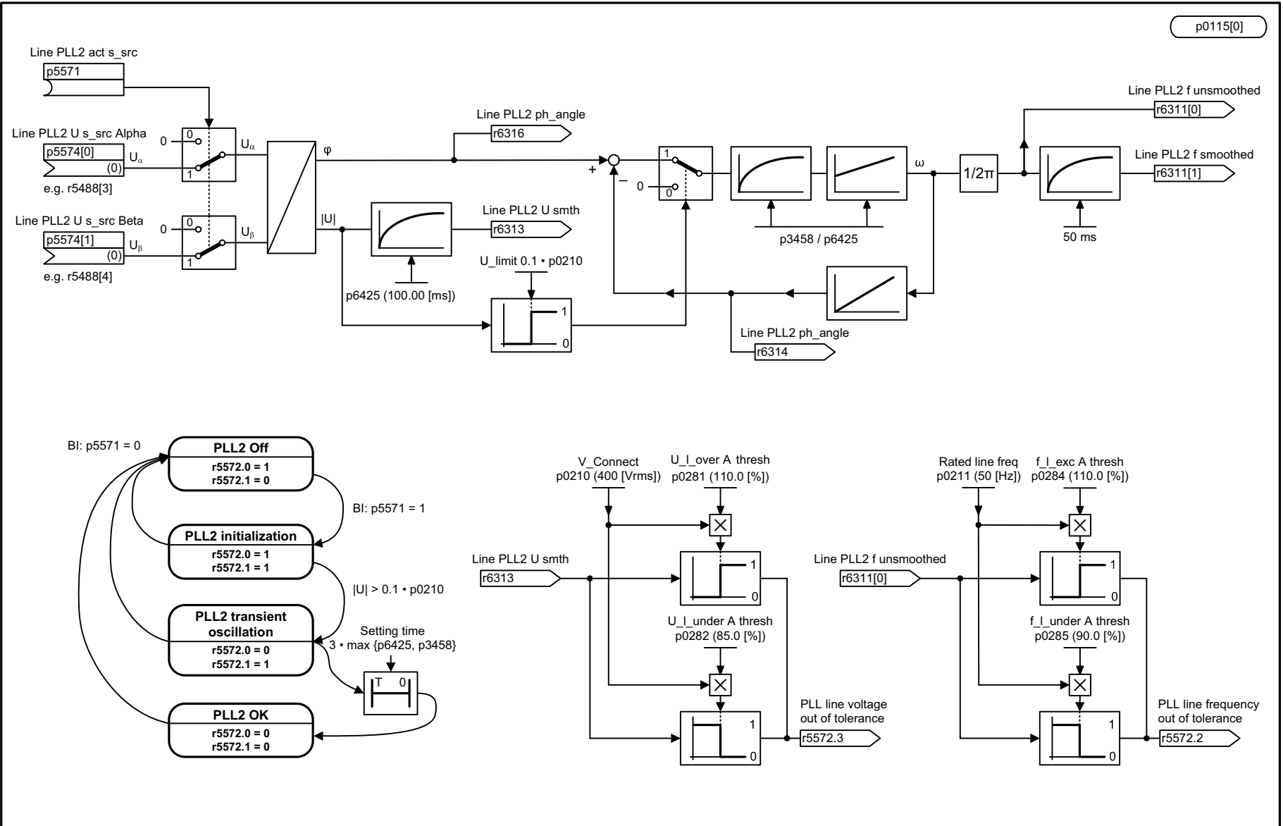
Fig. 3-293 7992 - PLL2 (phase locked loop 2)
