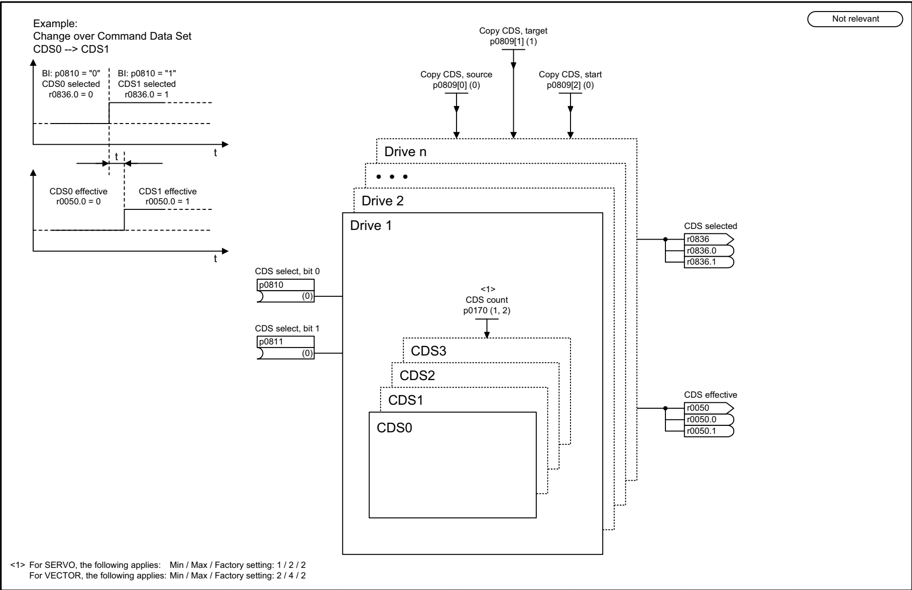
Fig. 3-321 8560 – Command Data Sets (CDS)
