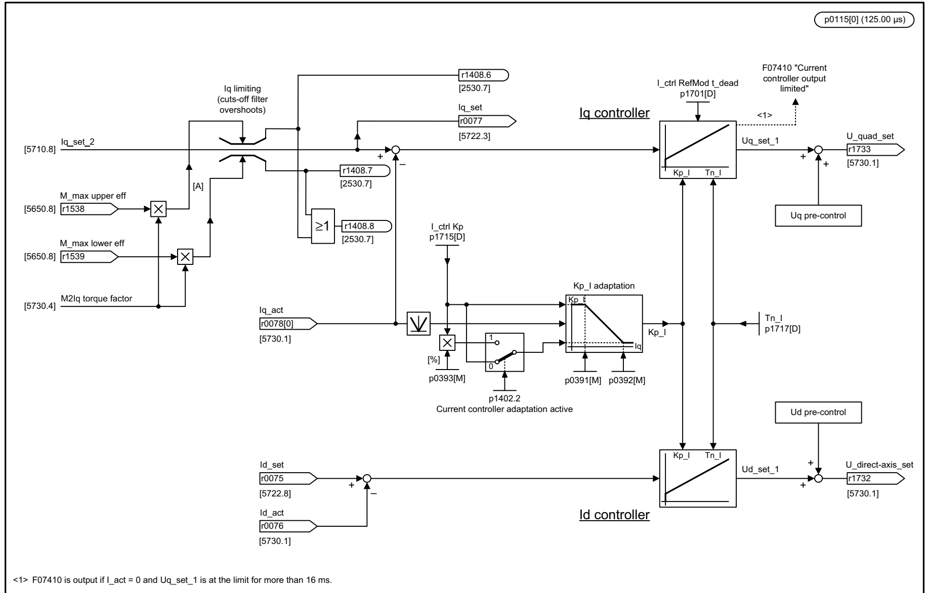
Fig. 3-230 5714 – Iq and Id controllers
