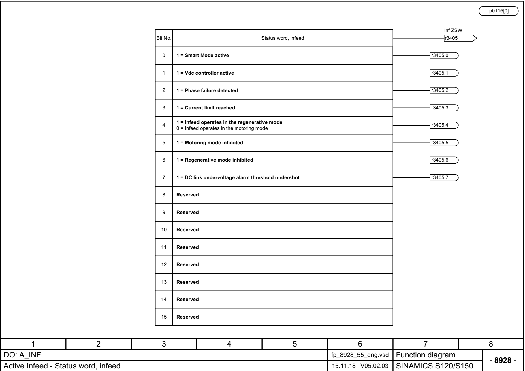
Fig. 3-345 8928 – Status word infeed
