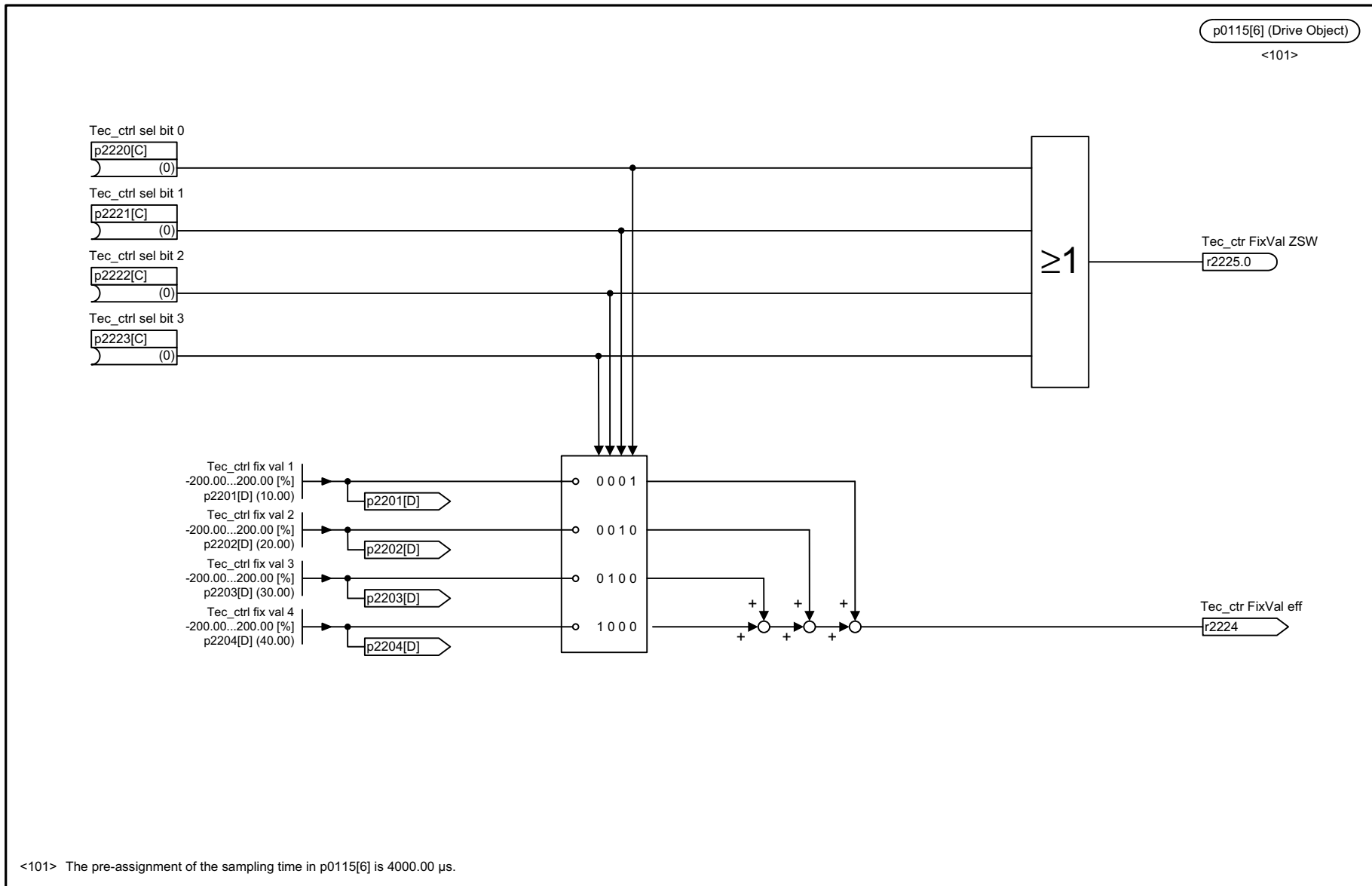
Fig. 3-278 7951 – Fixed values, direct selection (r0108.16 = 1 and p2216 = 1)
