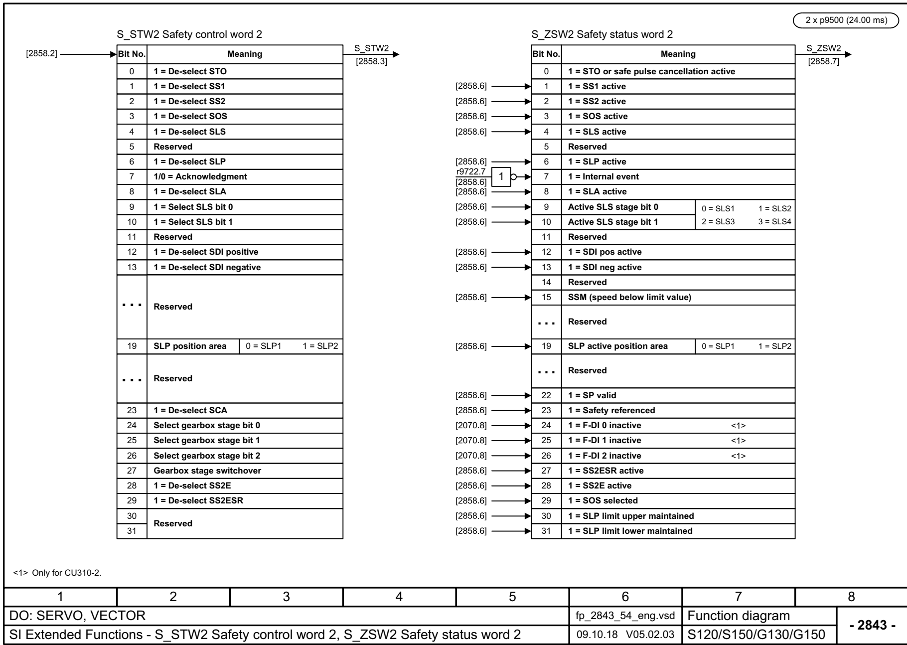
Fig. 3-132 2843 – S_STW2 Safety control word 2, S_ZSW2 Safety status word 2
