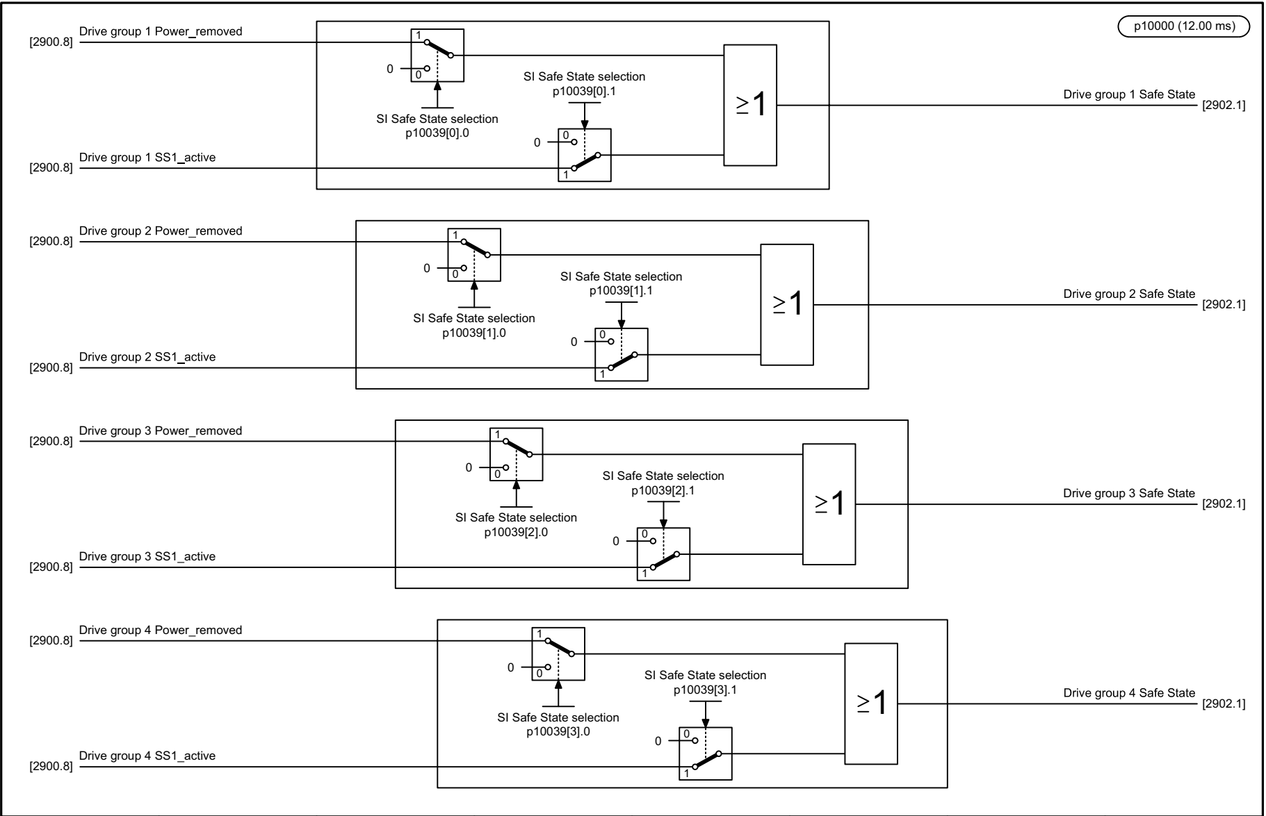
Fig. 3-149 2901 – Basic Functions safe state selection
