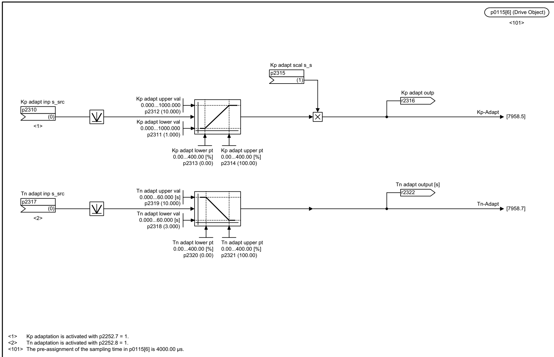
Fig. 3-281 7959 – Kp/Tn adaptation (r0108.16 = 1)
