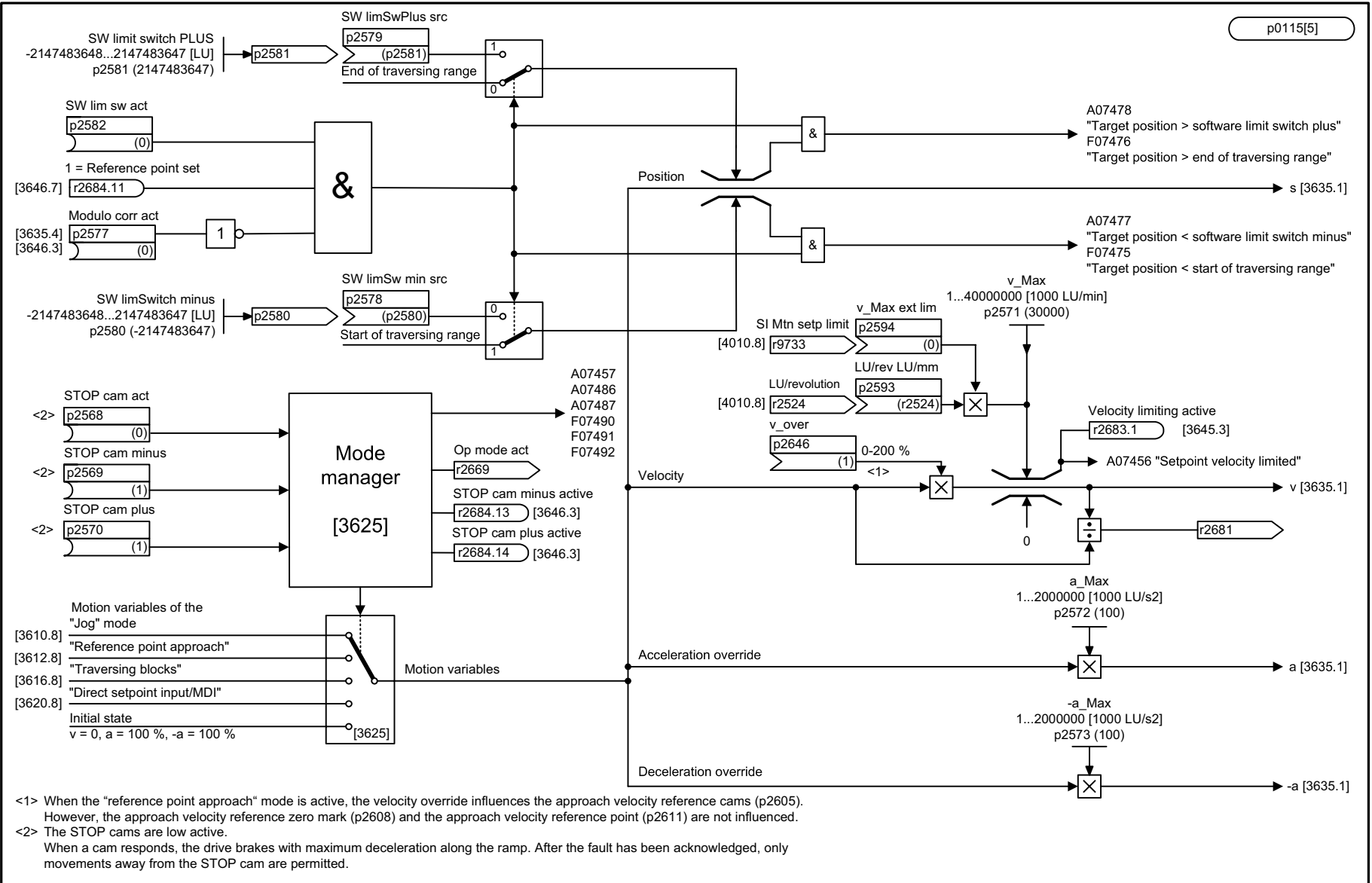
Fig. 3-177 3630 - Traversing range limits (r0108.4 = 1)
