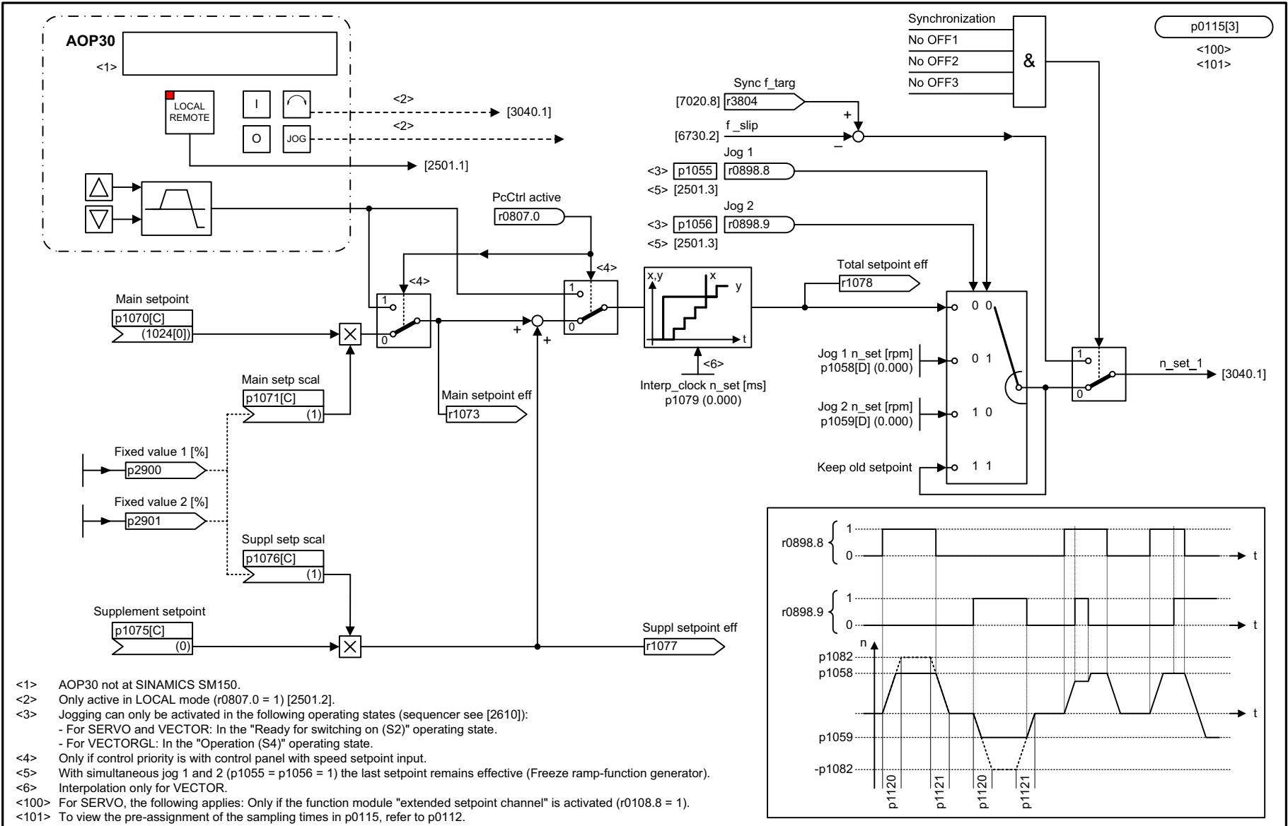
Fig. 3-159 3030 – Main/supplementary setpoint, setpoint scaling, jogging
