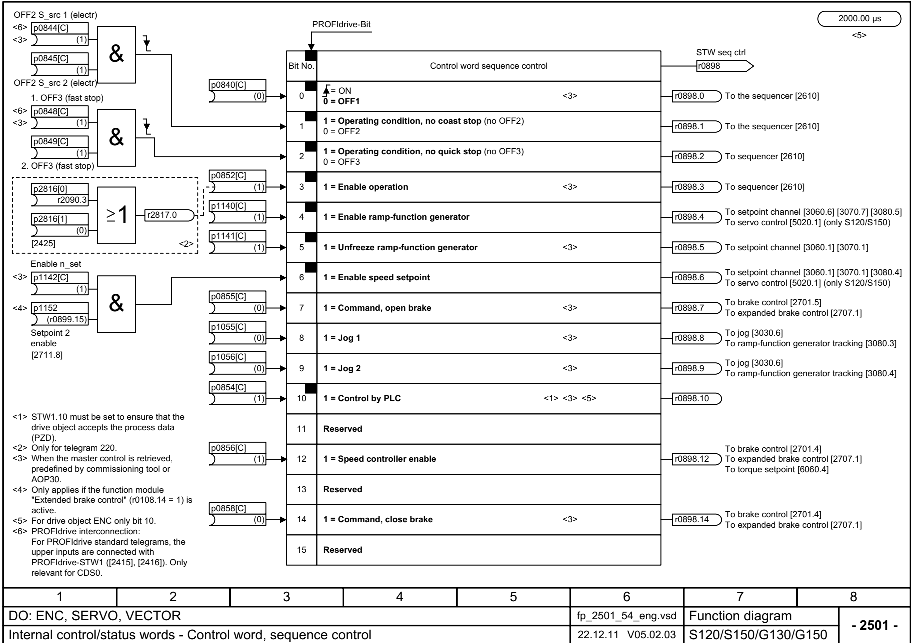
Fig. 3-95 2501 – Control word sequence control
