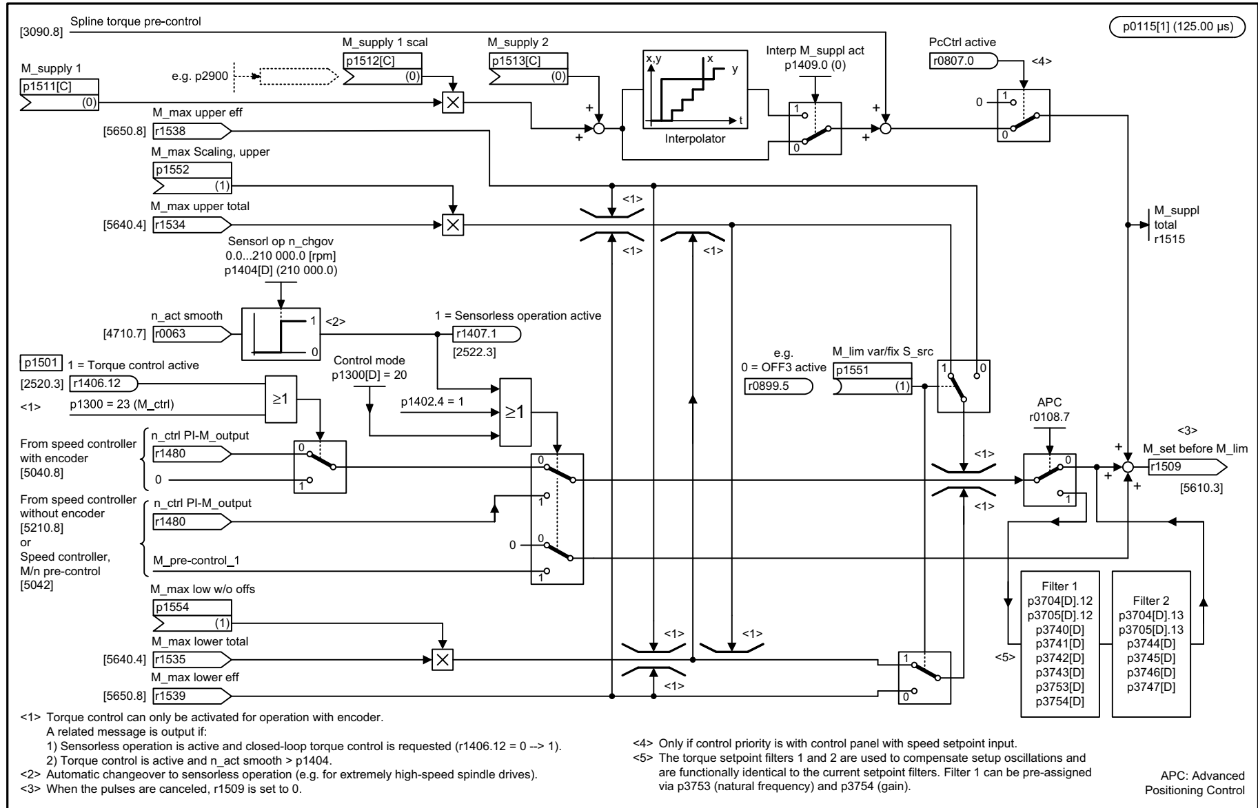
Fig. 3-216 5060 – Torque setpoint, switchover control mode
