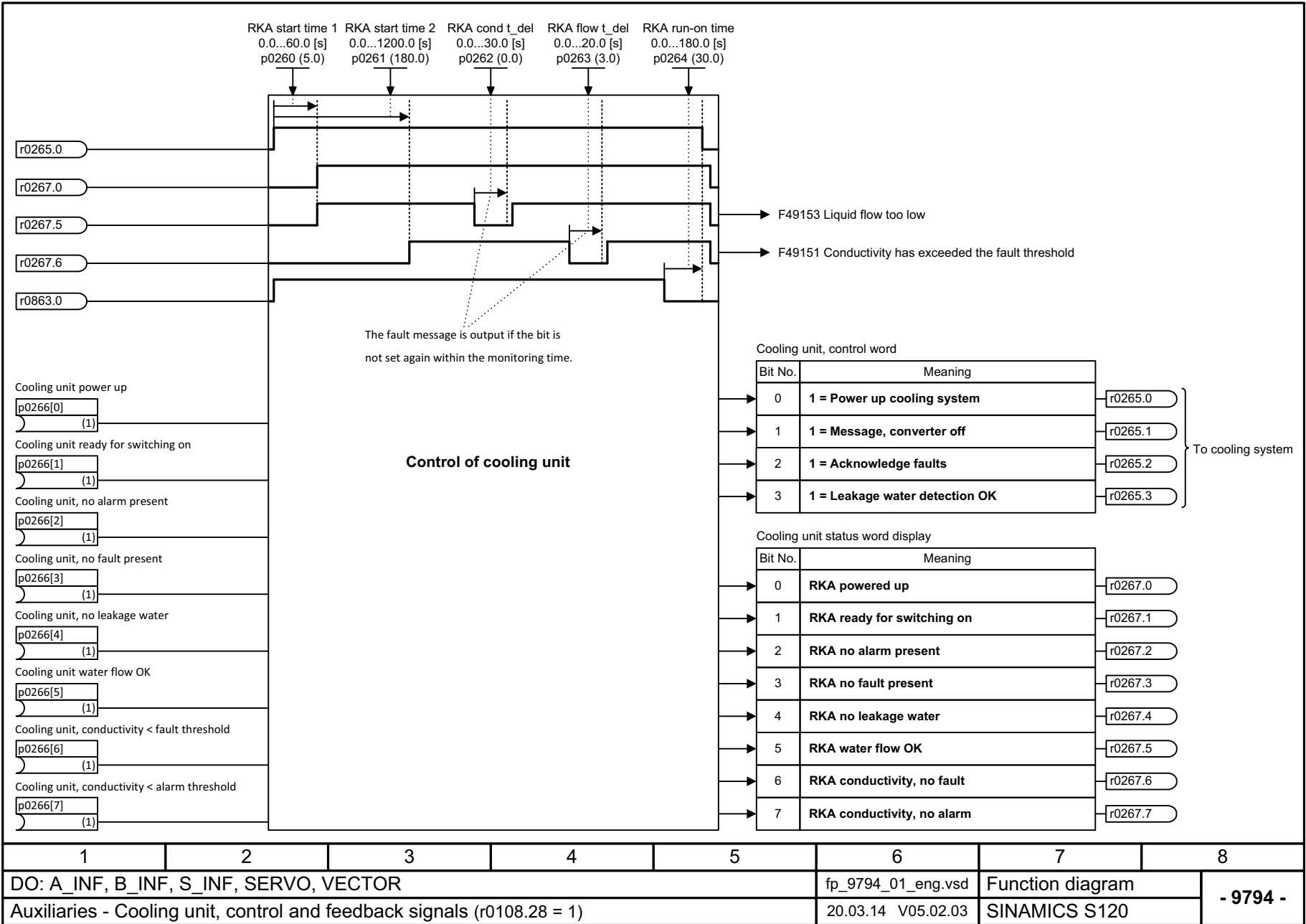
Fig. 3-403 9794 – Cooling unit, control and feedback signals (r0108.28 = 1)
