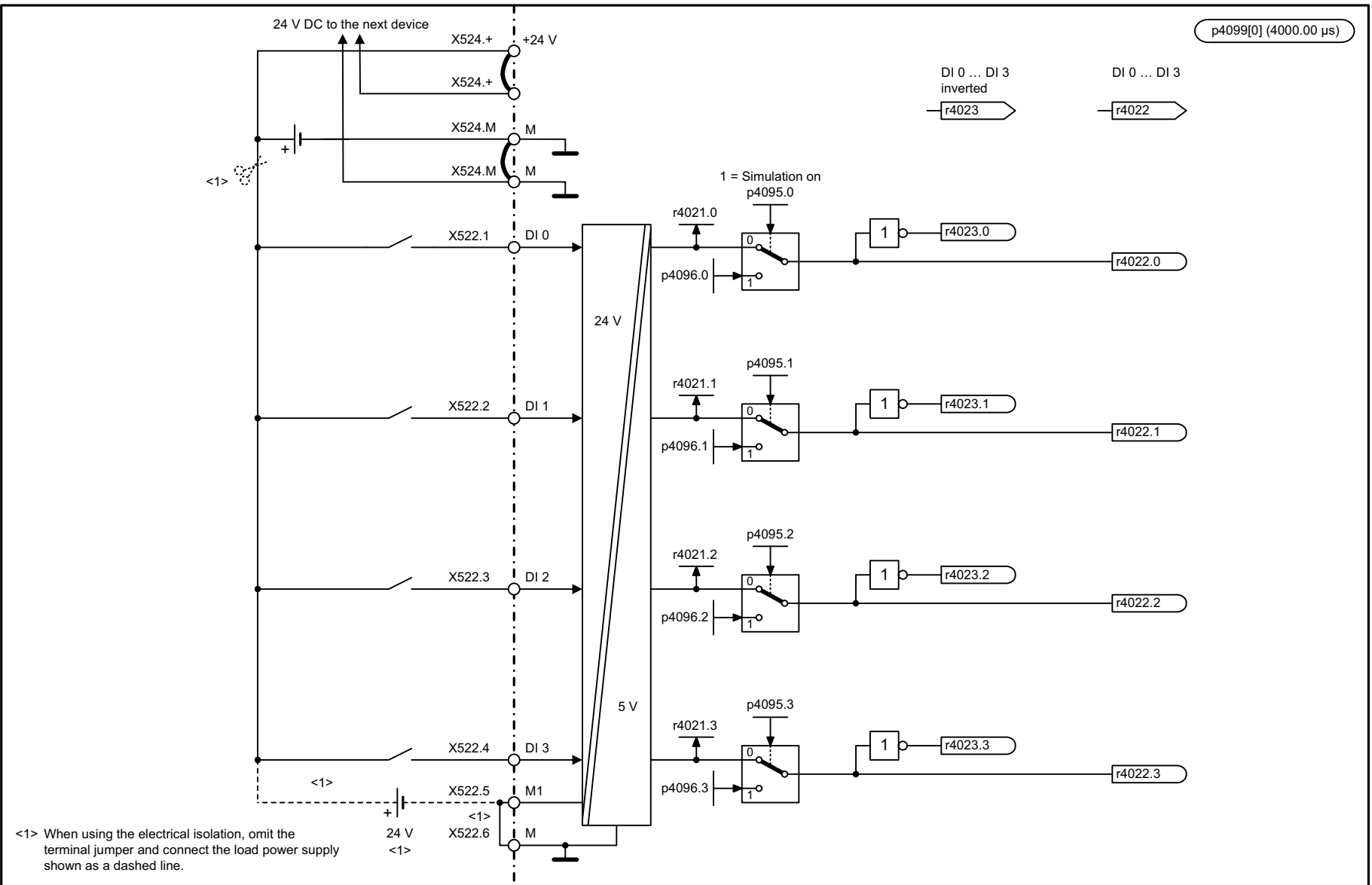
Fig. 3-390 9660 – Digital inputs electrically isolated (DI 0 ... DI 3)
