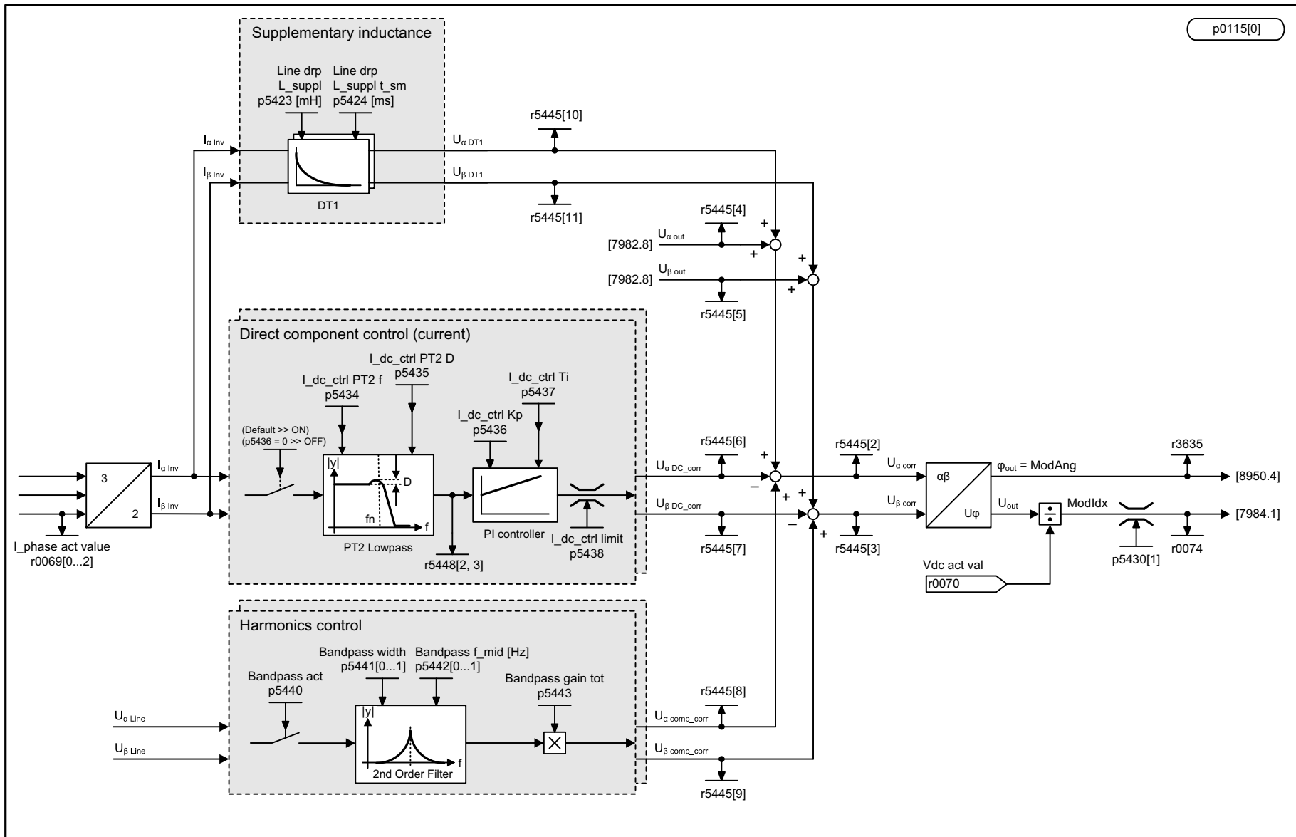
Fig. 3-284 7983 – Direct component control, harmonics control
