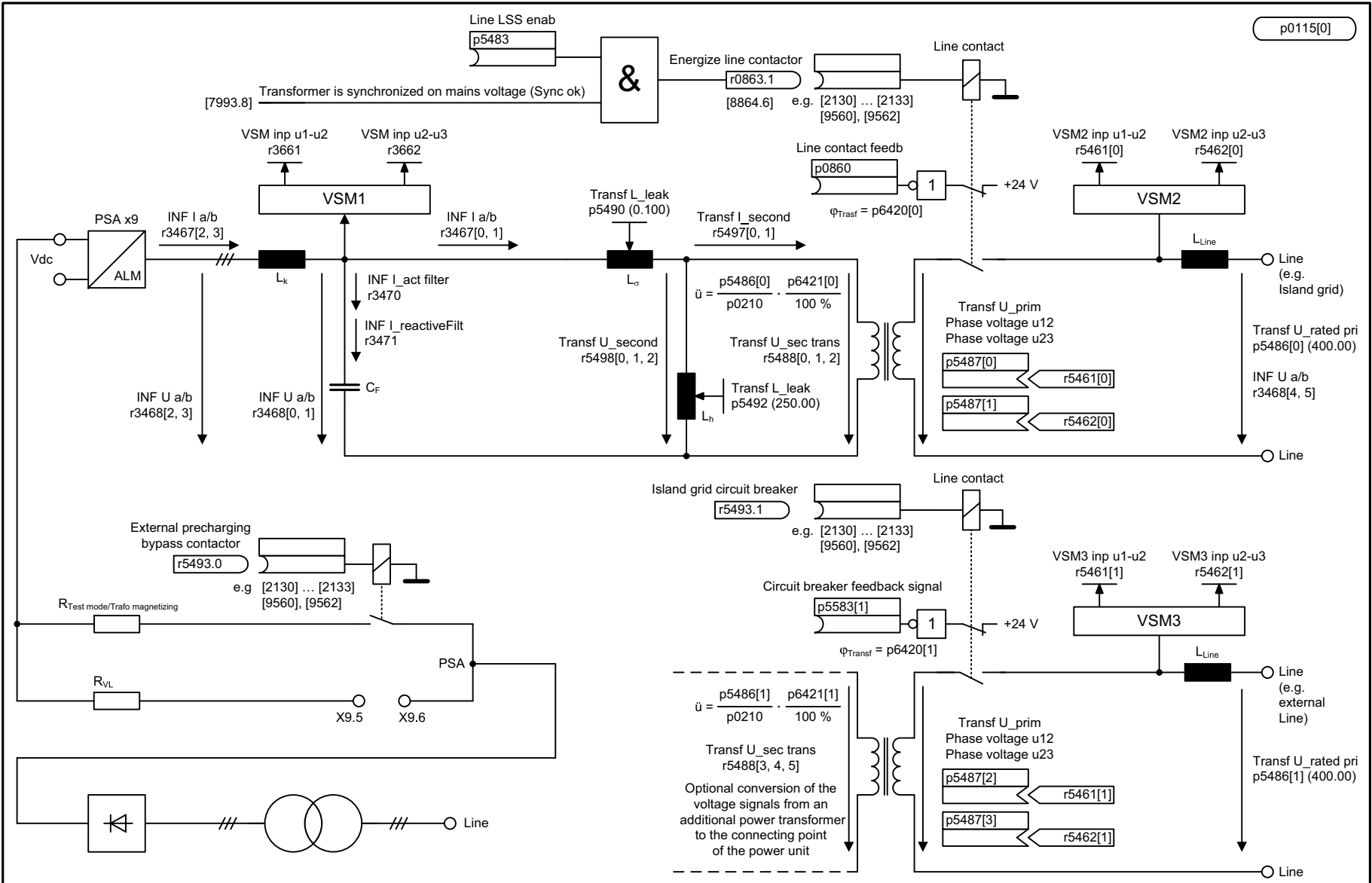
Fig. 3-291 7990 – Transformer model (p5480 = 1)
