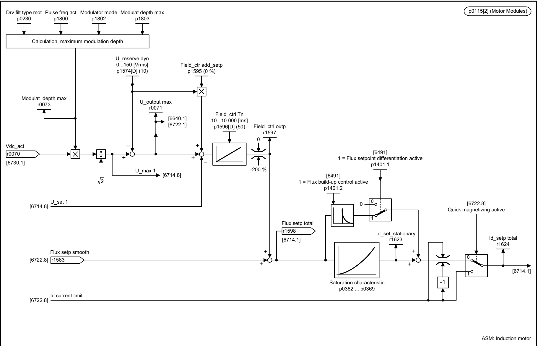
Fig. 3-255 6723 - Field weakening controller, flux controller (ASM, p0300 = 1)
