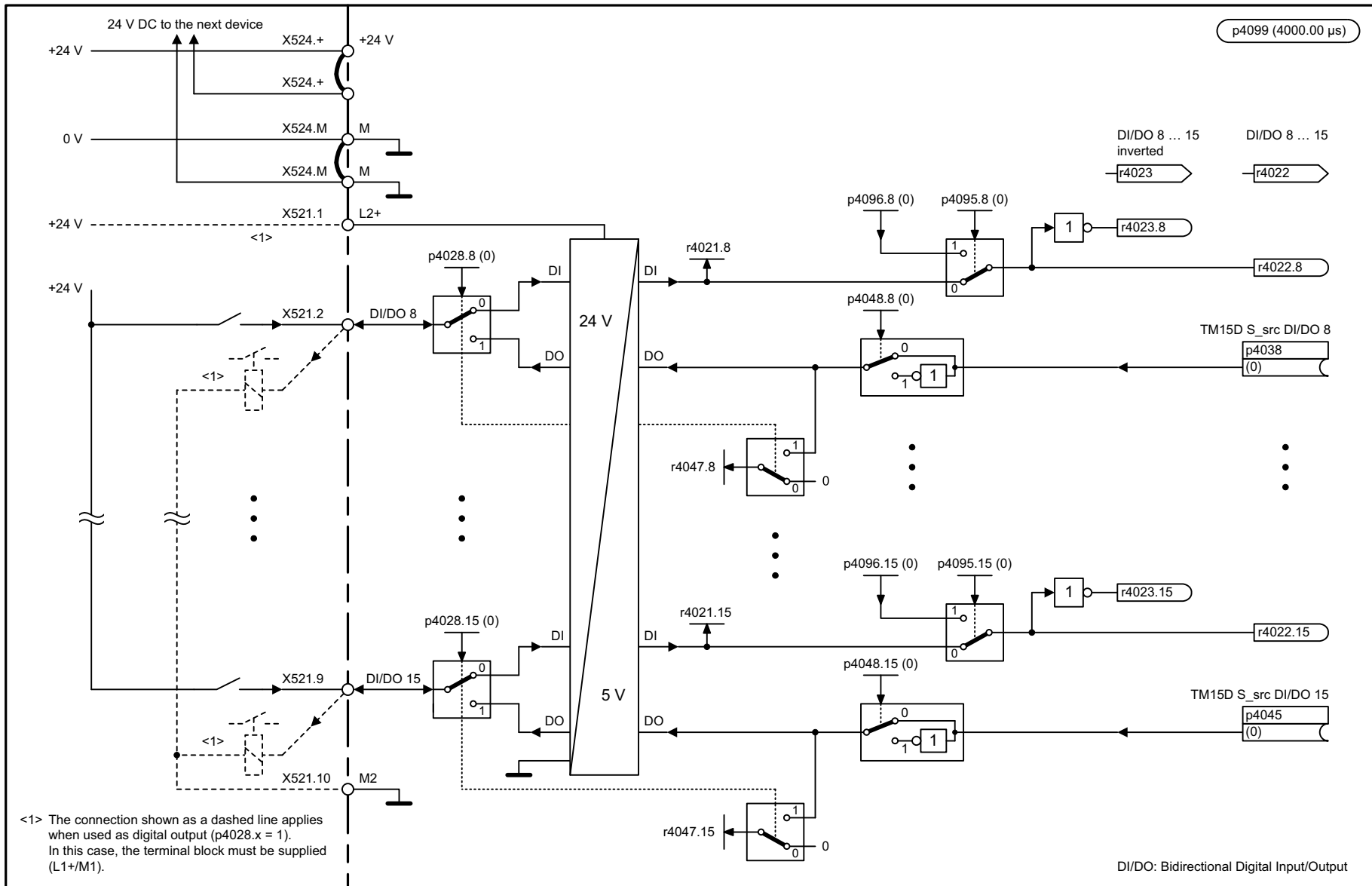
Fig. 3-370 9401 – Digital inputs/outputs bidirectional (DI/DO 8 ... DI/DO 15)
