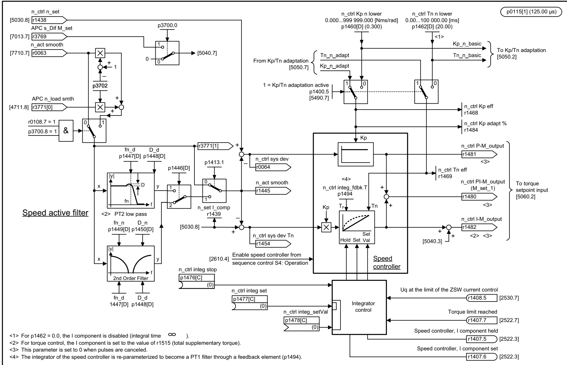
Fig. 3-211 5040 – Speed controller with encoder
