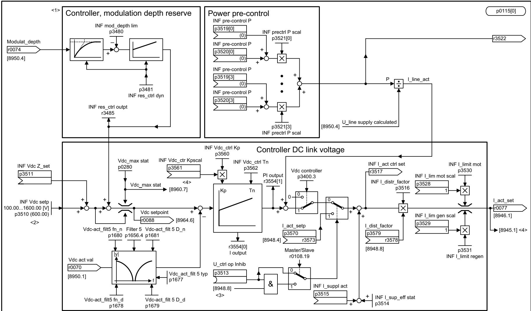
Fig. 3-348 8940 – Controller modulation depth reserve/controller DC link voltage (p3400.0 = 0)
