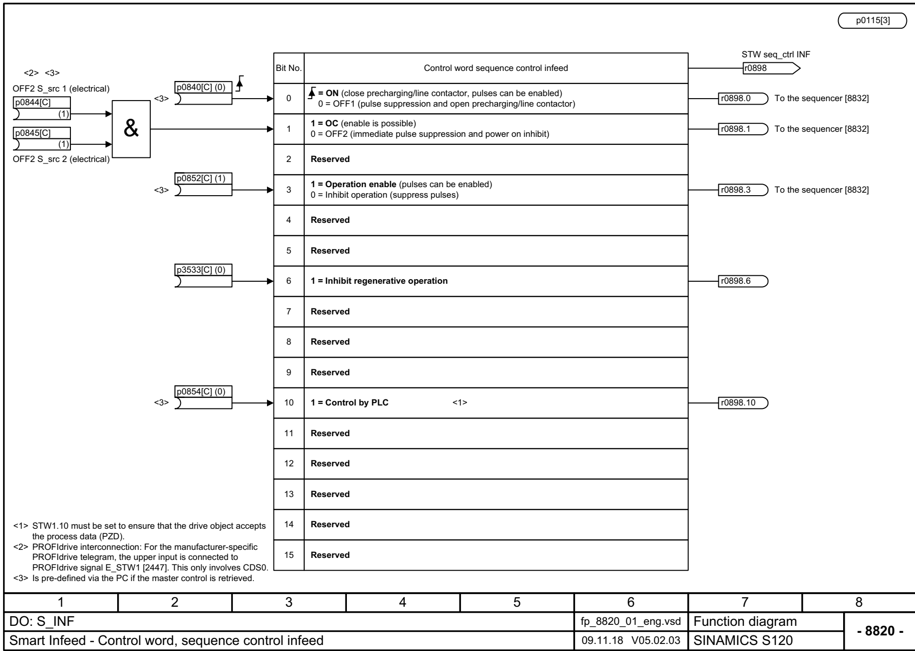
Fig. 3-334 8820 – Control word sequence control infeed
