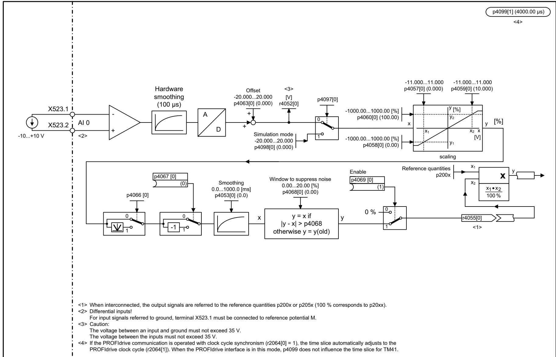
Fig. 3-393 9663 – Analog input 0 (AI 0)
