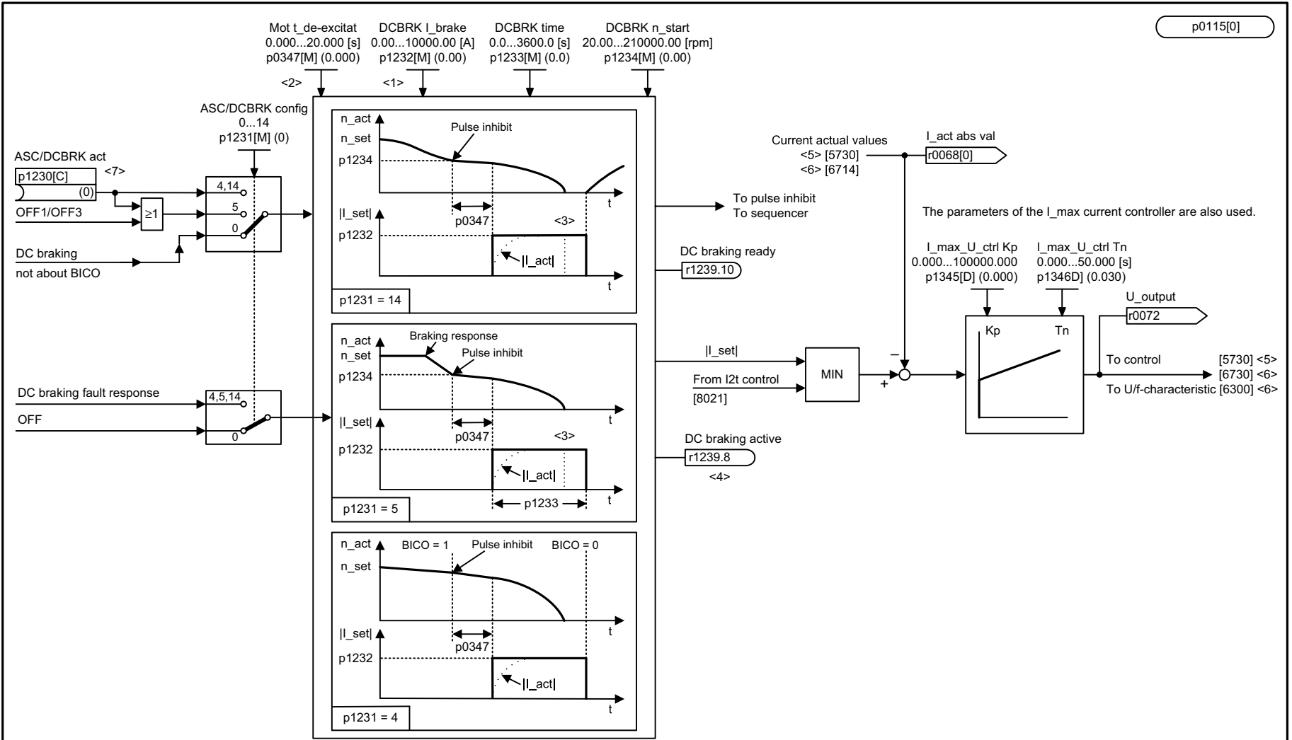
Fig. 3-274 7017 - DC braking (p0300 = 1xx)
