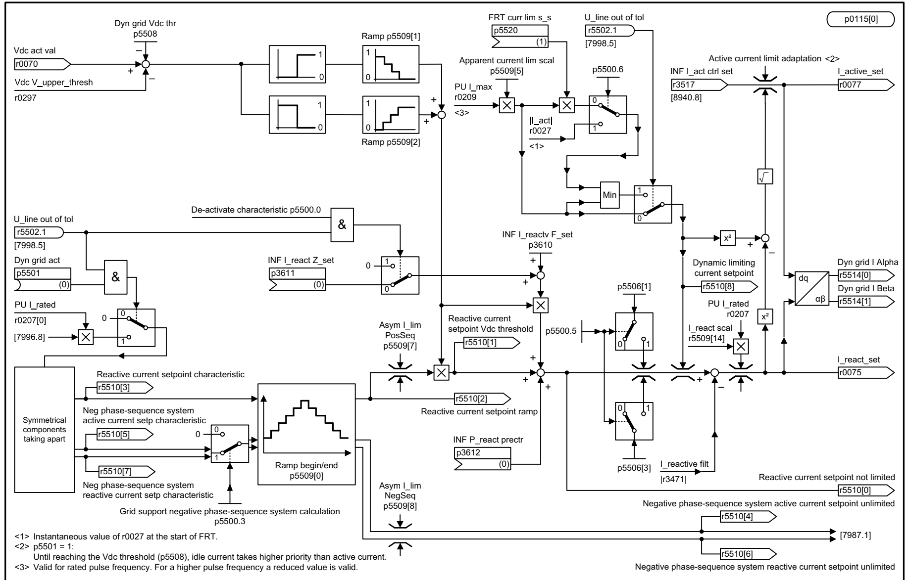
Fig. 3-297 7997 - Current limits (p5501 = 1)
