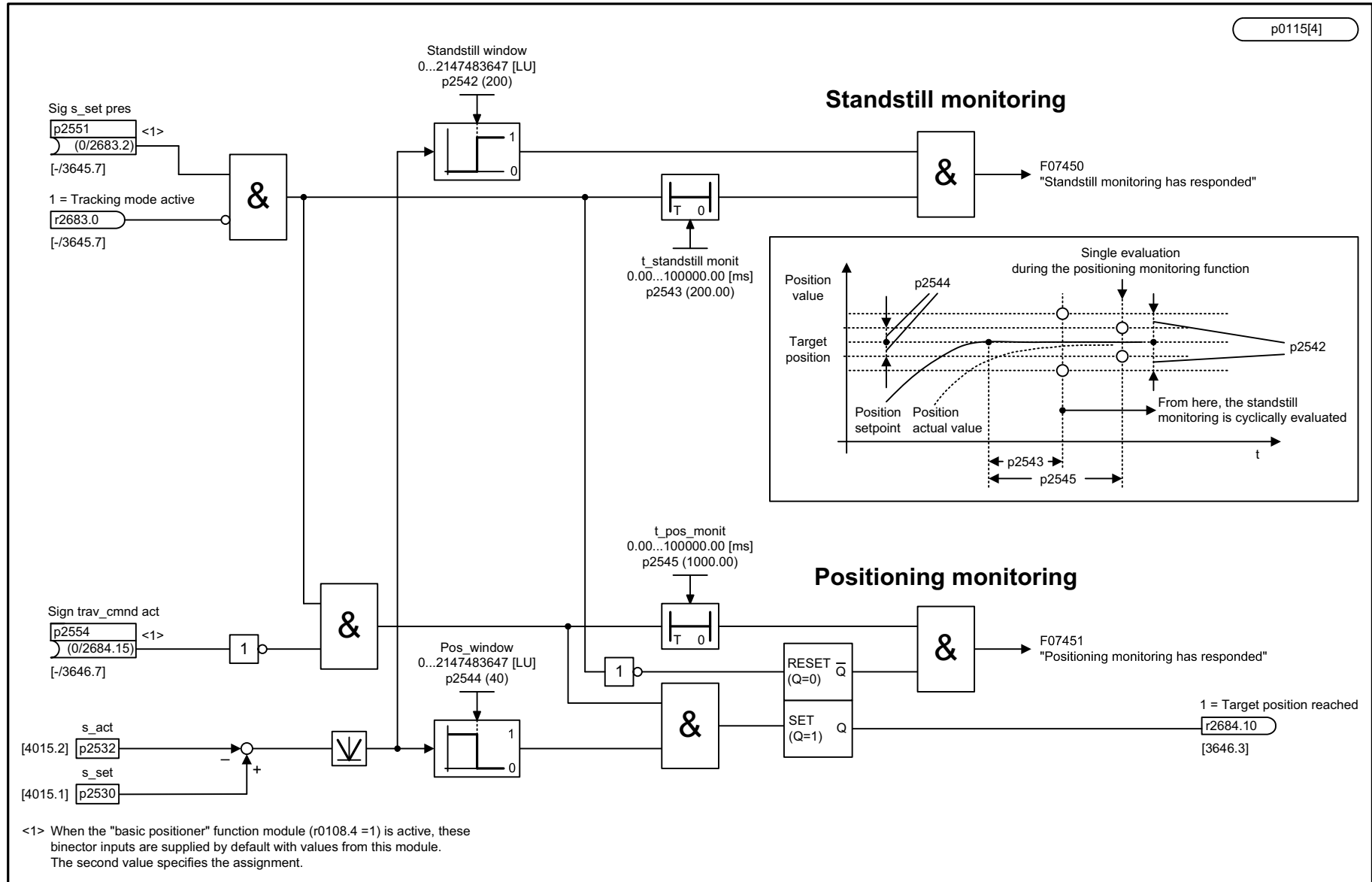
Fig. 3-185 4020 – Standstill monitoring / positioning monitoring (r0108.3 = 1)
