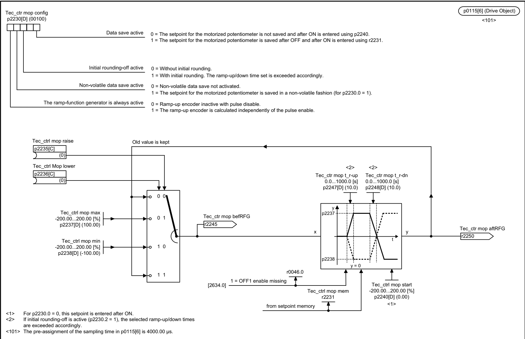
Fig. 3-279 7954 – Motorized potentiometer (r0108.16 = 1)
