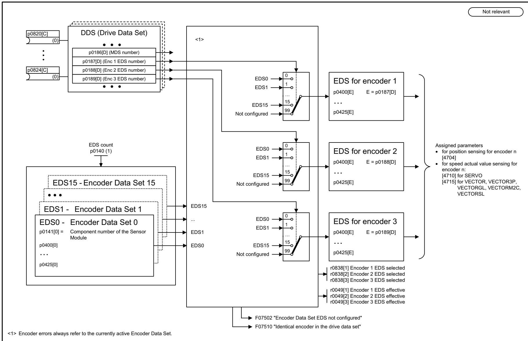
Fig. 3-323 8570 – Encoder Data Sets (EDS)
