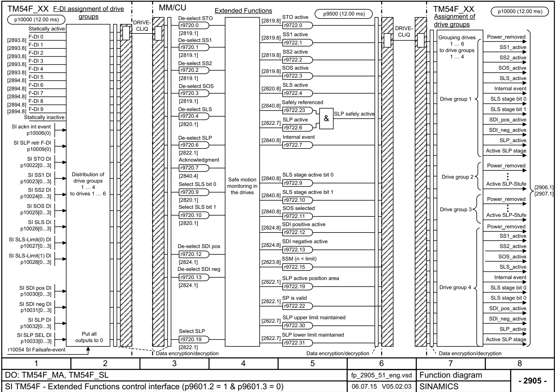
Fig. 3-151 2905 – Extended Functions control interface (p9601.2 = 1 & p9601.3 = 0)
