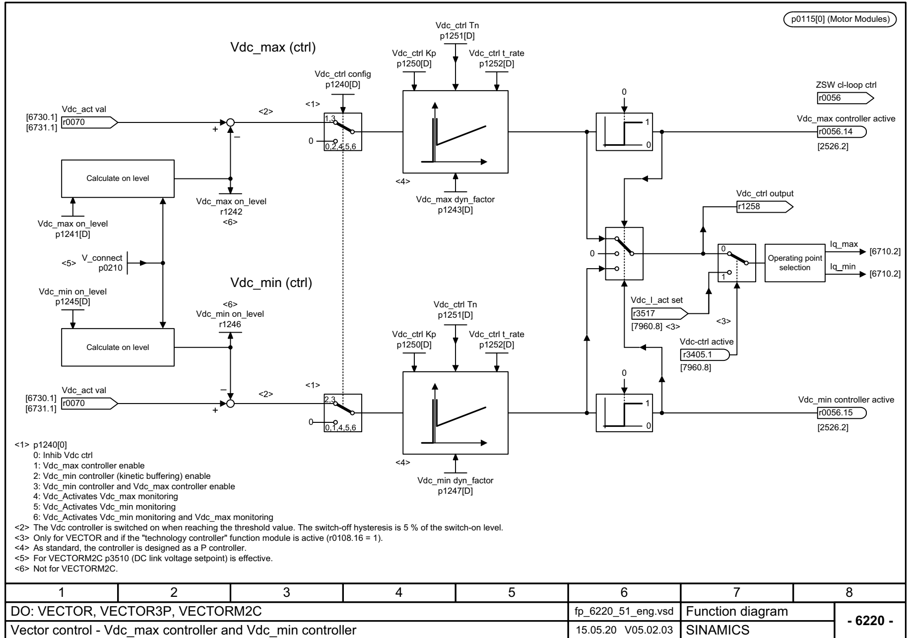
Fig. 3-240 6220 – Vdc_max controller and Vdc_min controller
