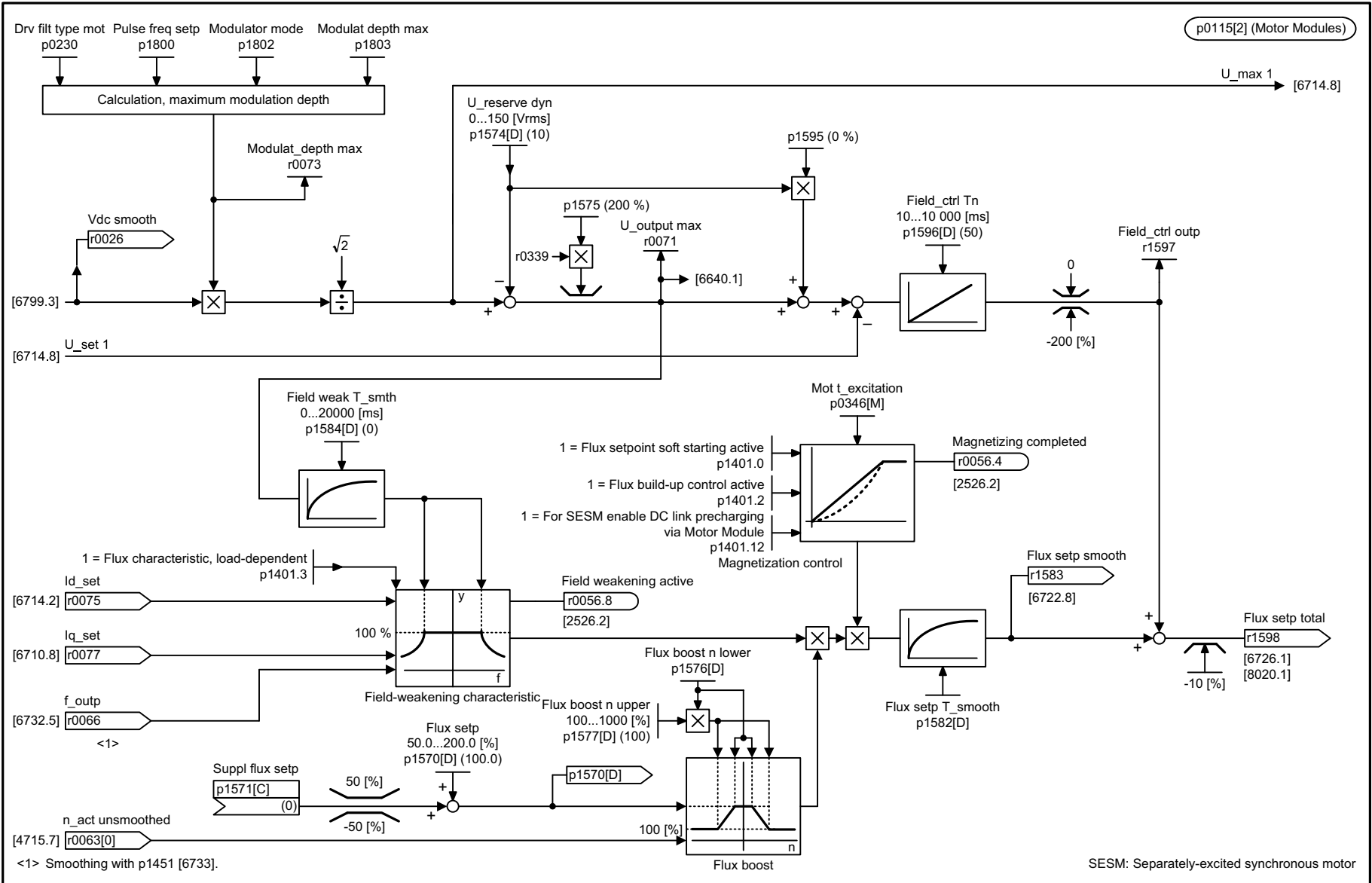
Fig. 3-257 6725 – Flux setpoint, field weakening controller (SESM, p0300 = 5)
