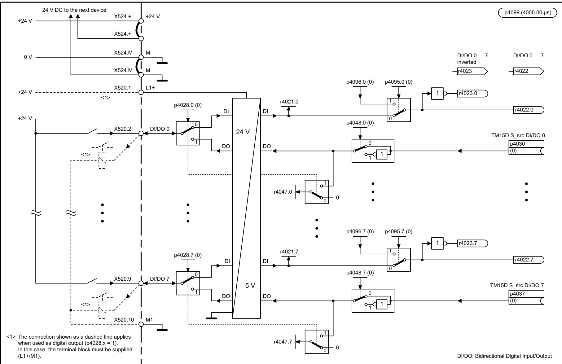
Fig. 3-369 9400 – Digital inputs/outputs bidirectional (DI/DO 0 ... DI/DO 7)
