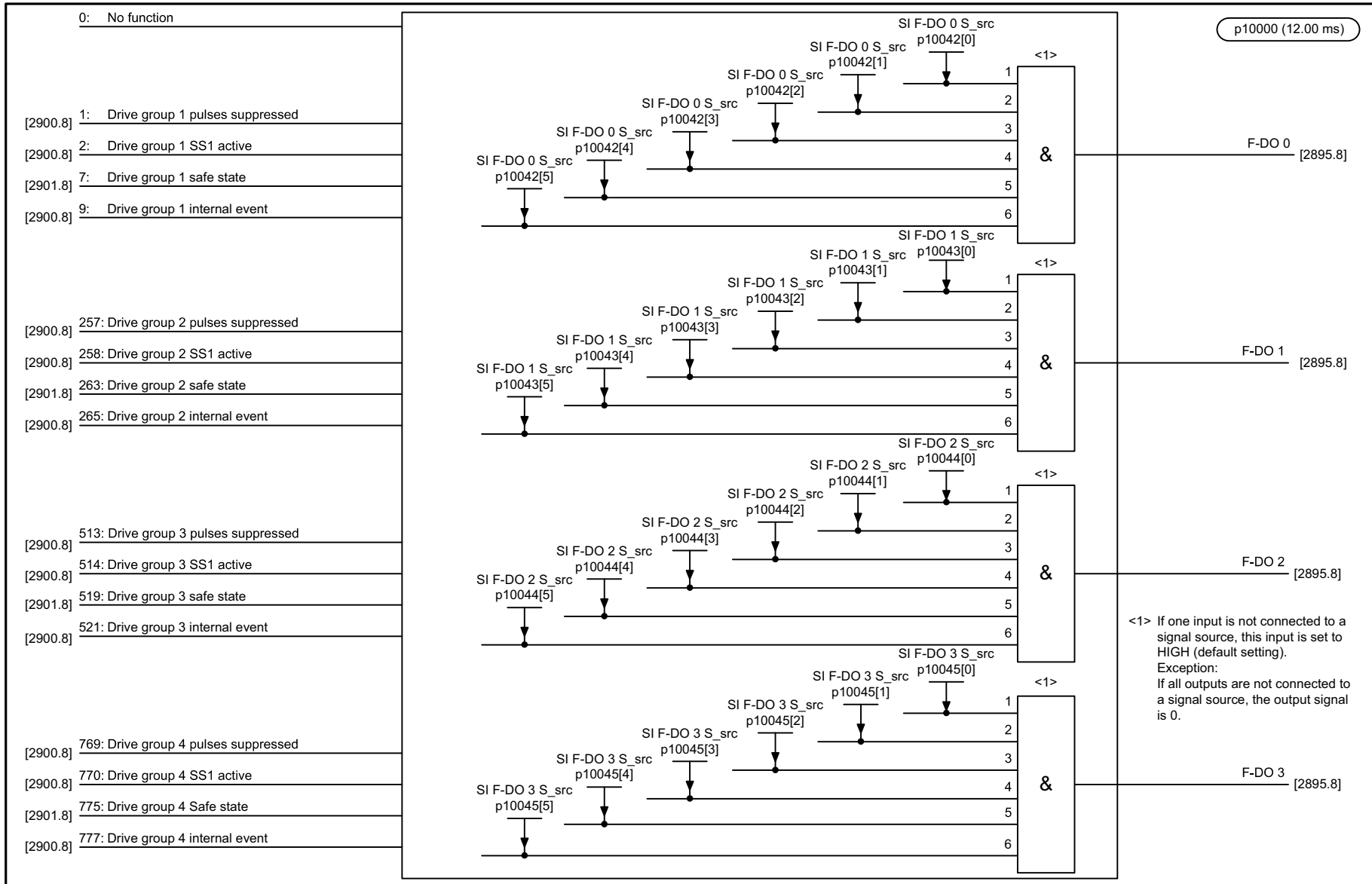
Fig. 3-150 2902 – Basic Functions assignment (F-DO 0 ... F-DO 3)
