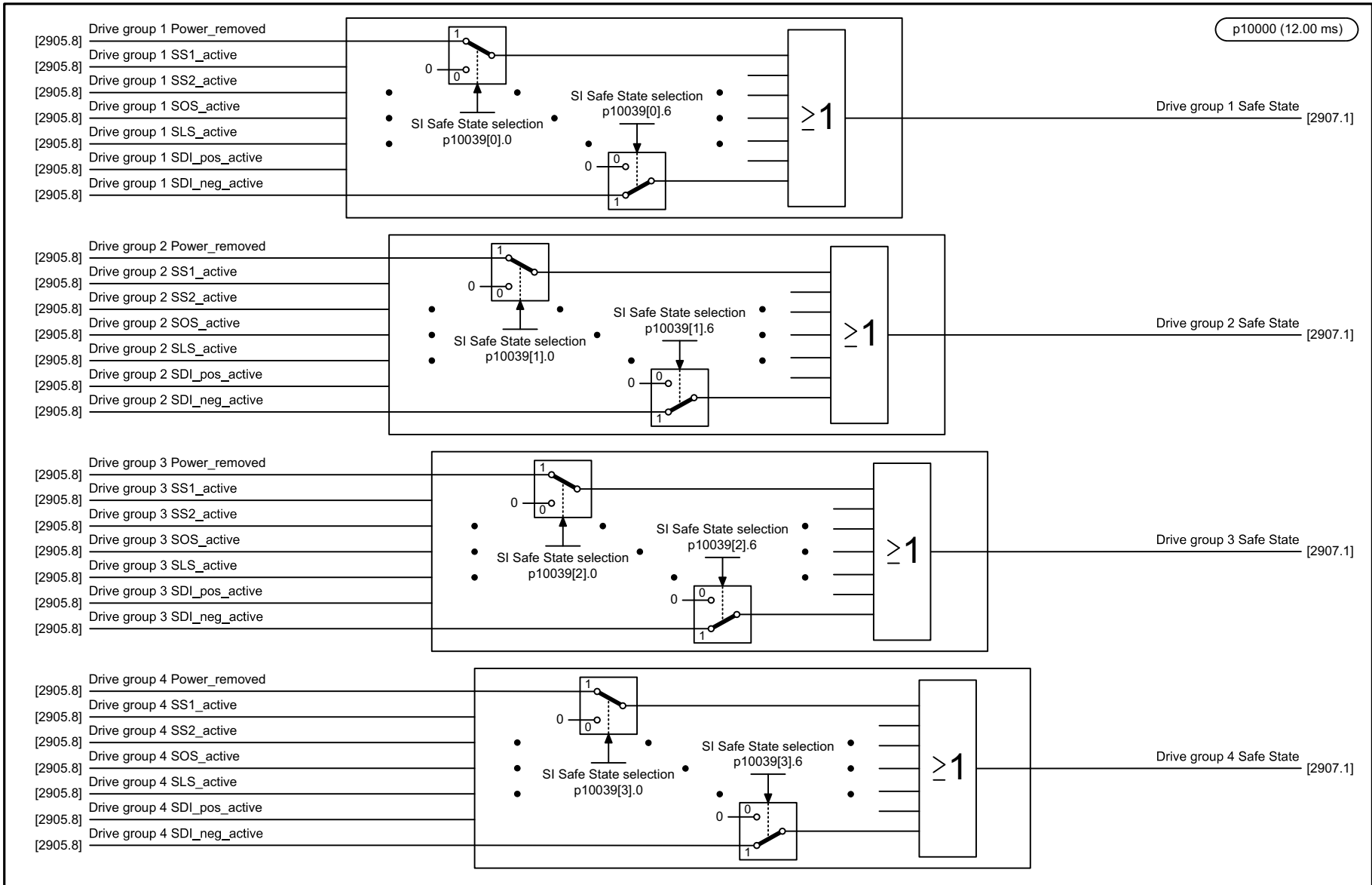
Fig. 3-152 2906 – Extended Functions safe state selection
