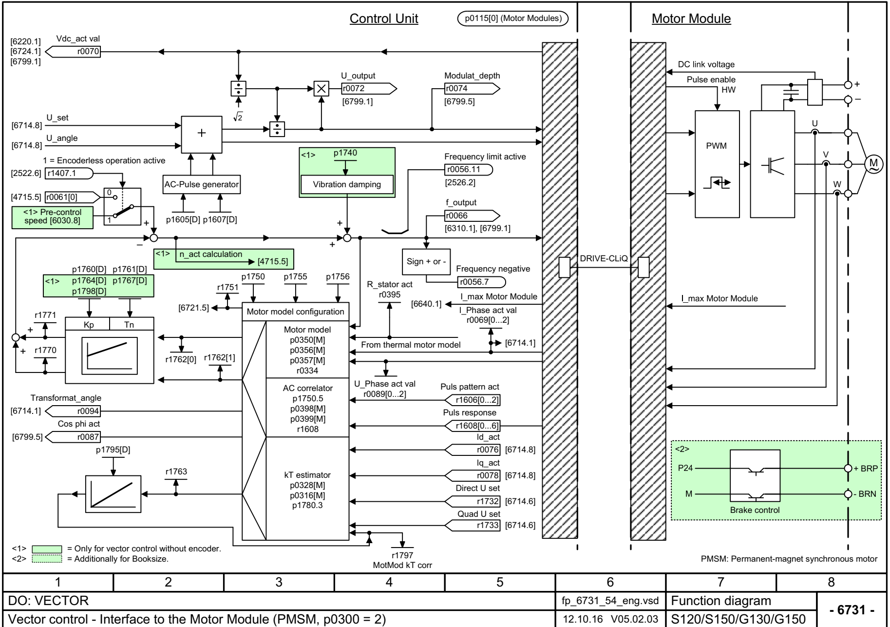
Fig. 3-261 6731 – Interface to the Motor Module (PMSM, p0300 = 2)
