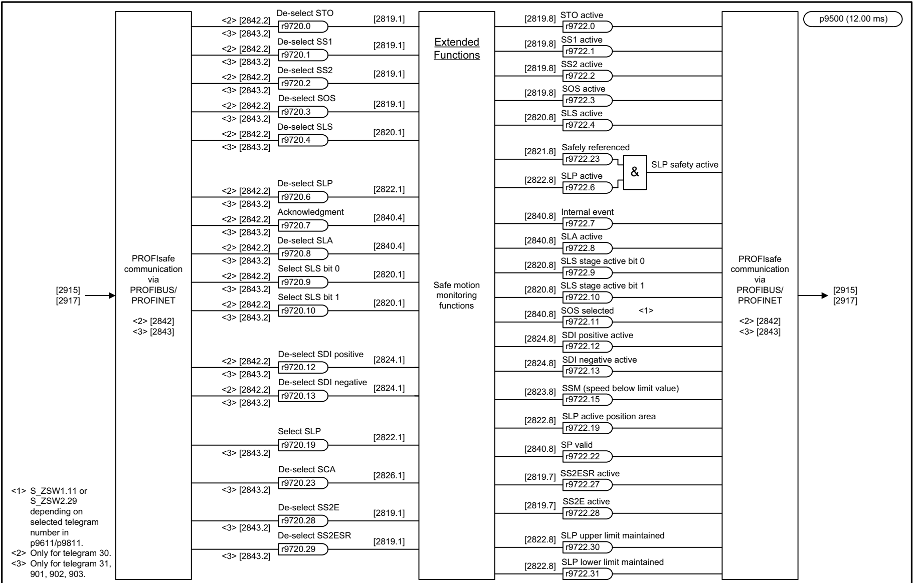
Fig. 3-133 2858 – Control via PROFIsafe (p9601.2 = p9601.3 = 1)
