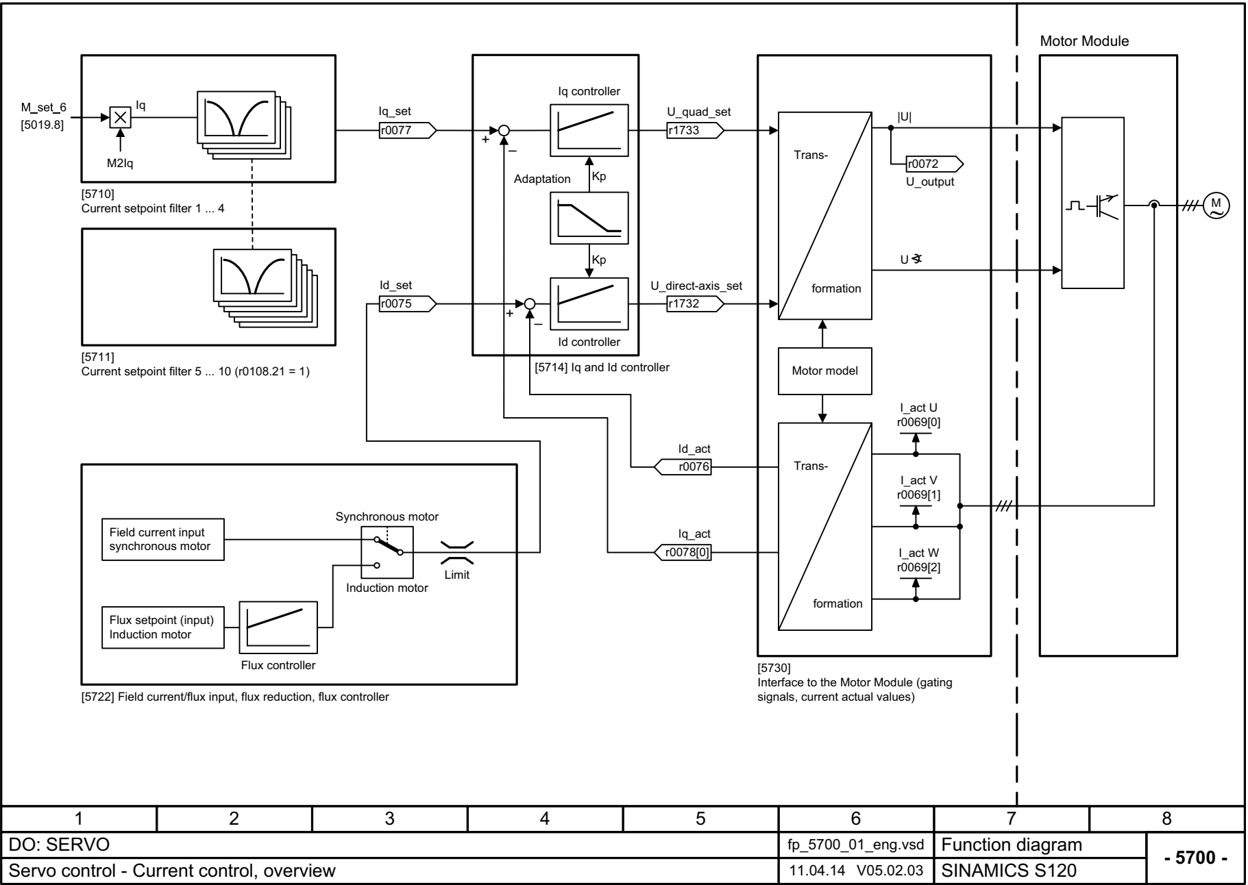
Fig. 3-227 5700 – Current control, overview
