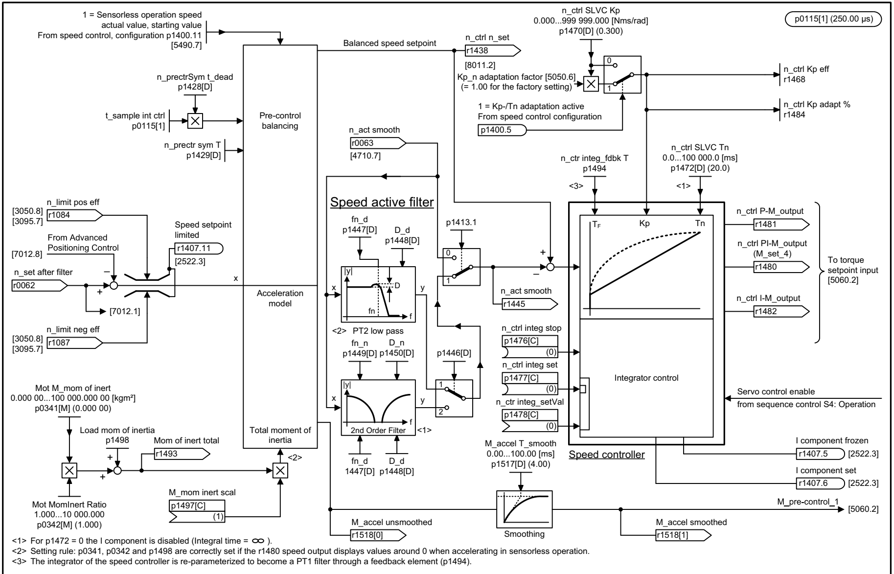
Fig. 3-217 5210 – Speed controller without encoder
