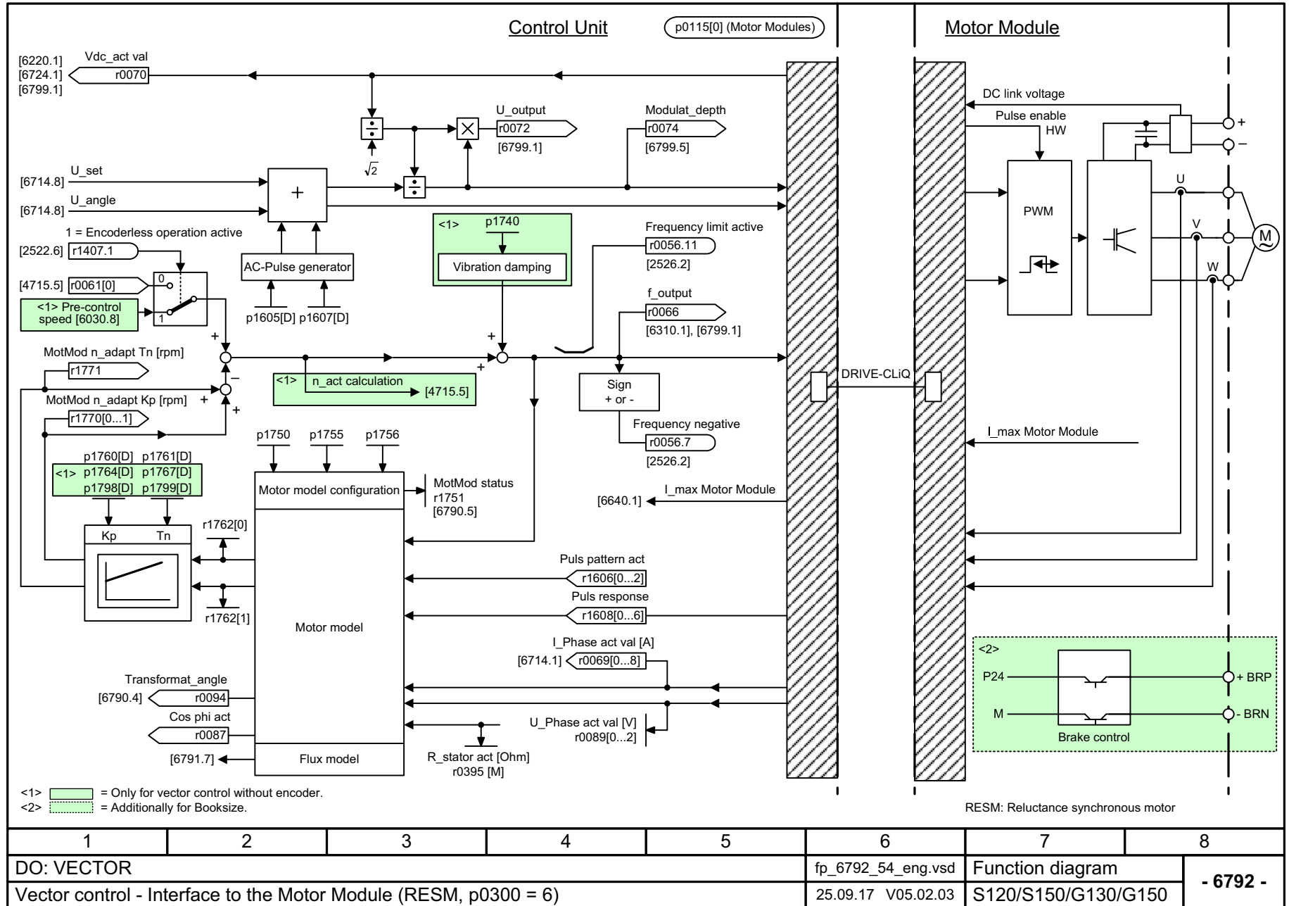
Fig. 3-266 6792 – Interface to the Motor Module (RESM, p0300 = 6)
