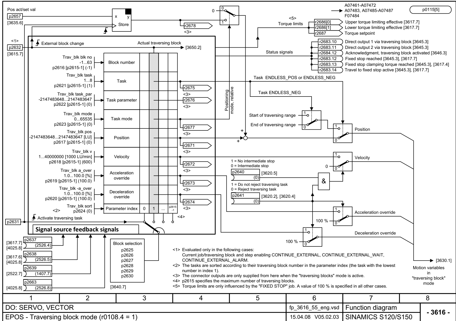
Fig. 3-172 3616 – Traversing block mode (r0108.4 = 1)
