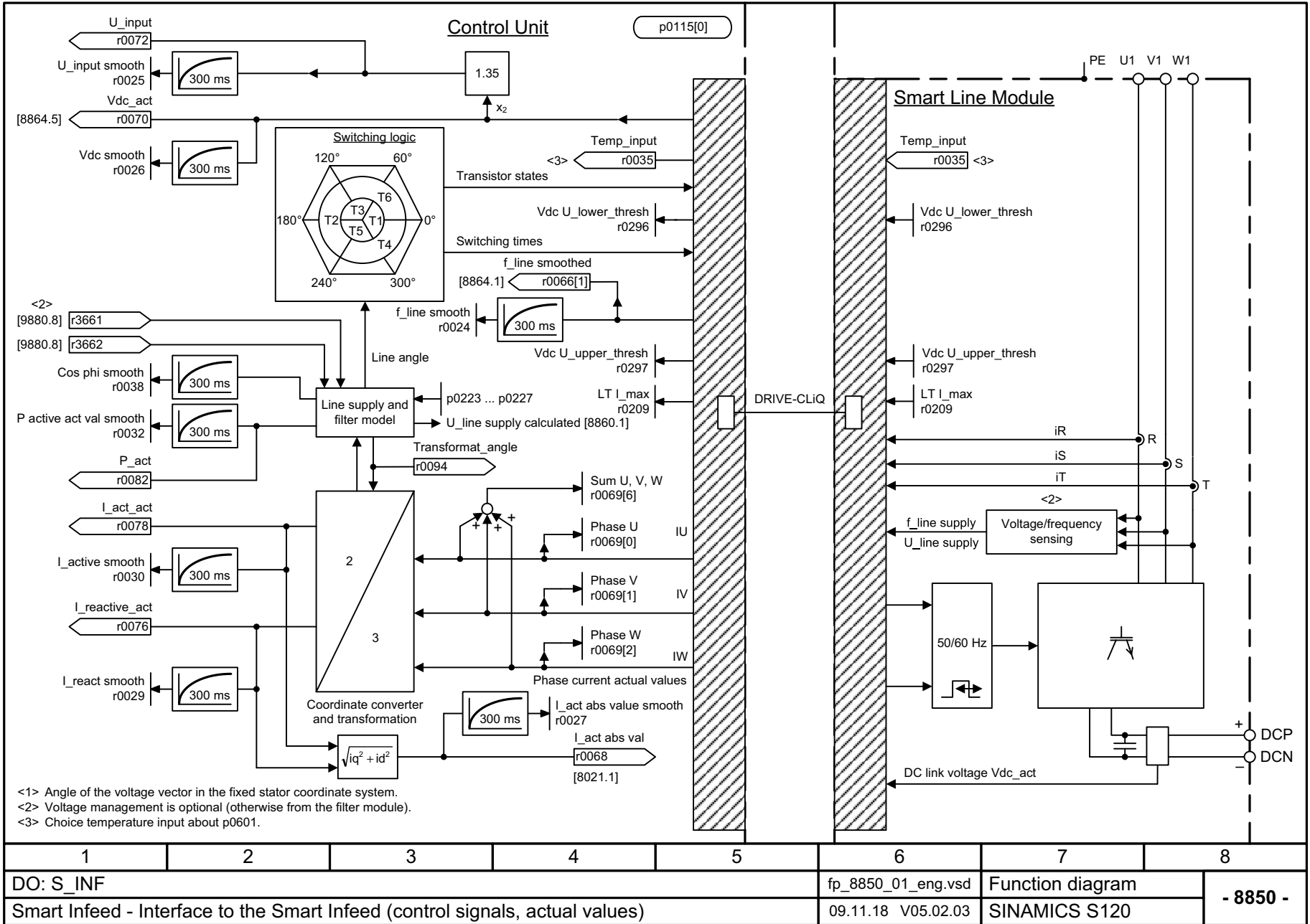
Fig. 3-339 8850 – Interface to the Smart Infeed (control signals, actual values)
