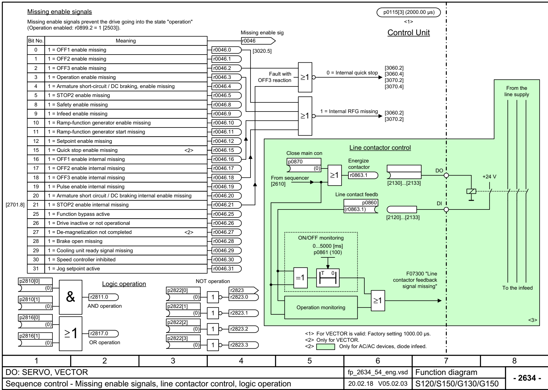
Fig. 3-108 2634 – Missing enables, line contactor control, logic operation
