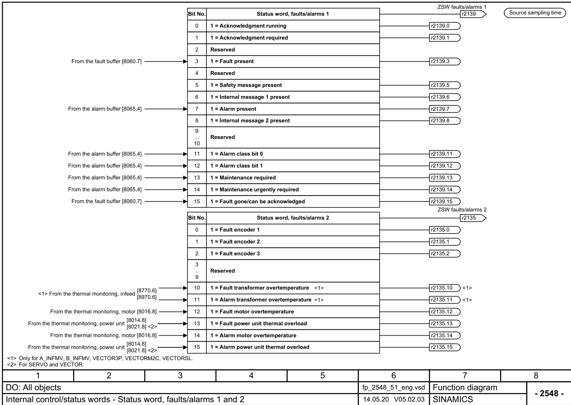
Fig. 3-106 2548 – Status word faults/alarms 1 and 2
