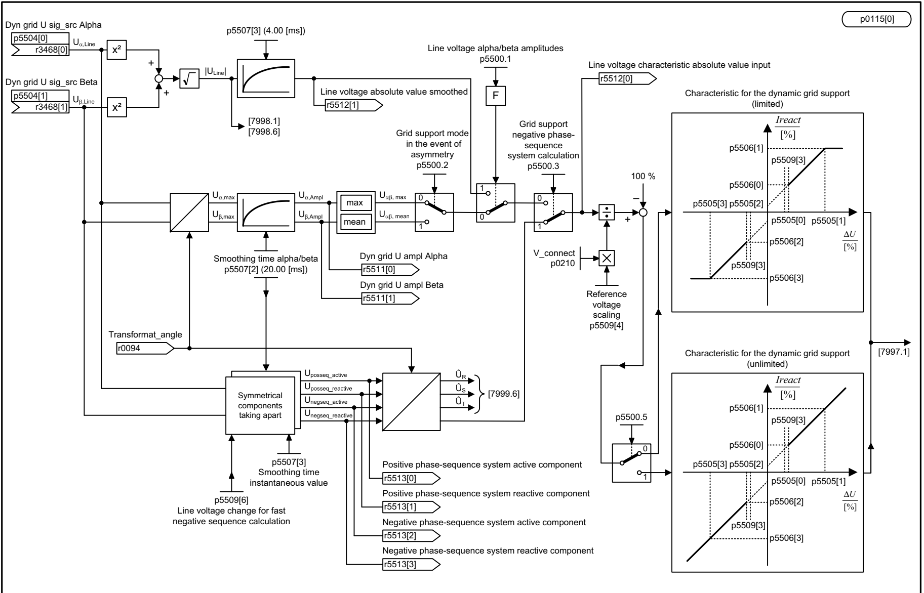
Fig. 3-296 7996 – Characteristic
