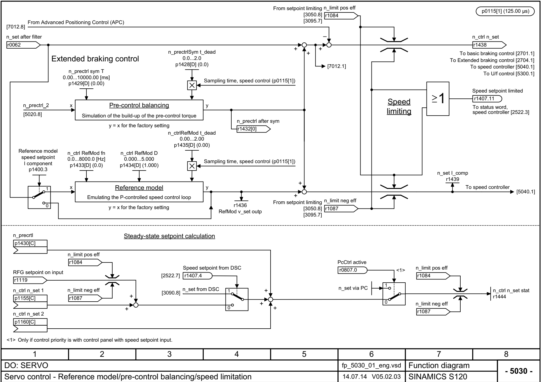
Fig. 3-209 5030 – Reference model/precontrol symmetrization/speed limitation
