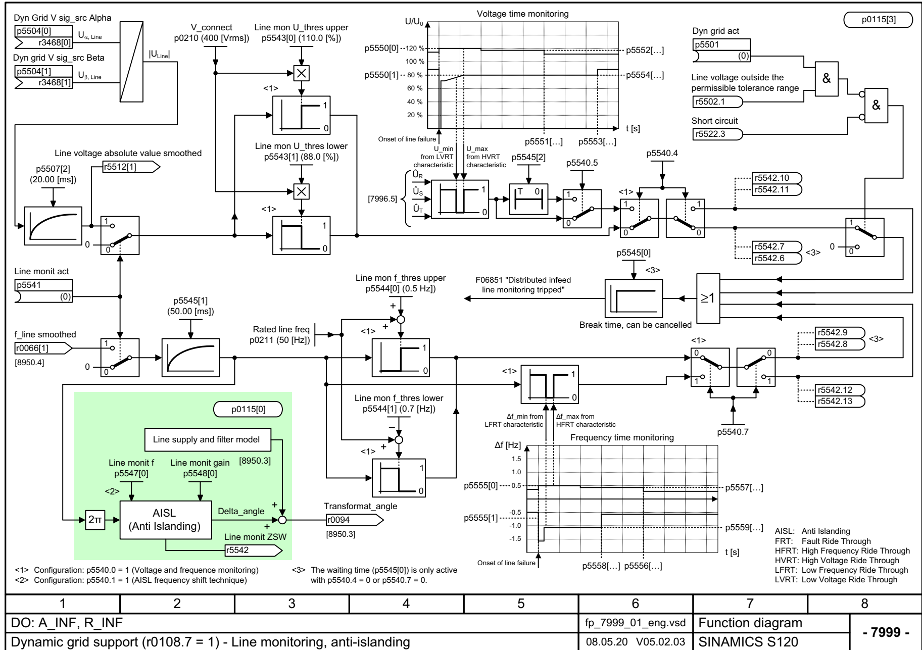
Fig. 3-299 7999 – Grid monitoring anti-islanding
