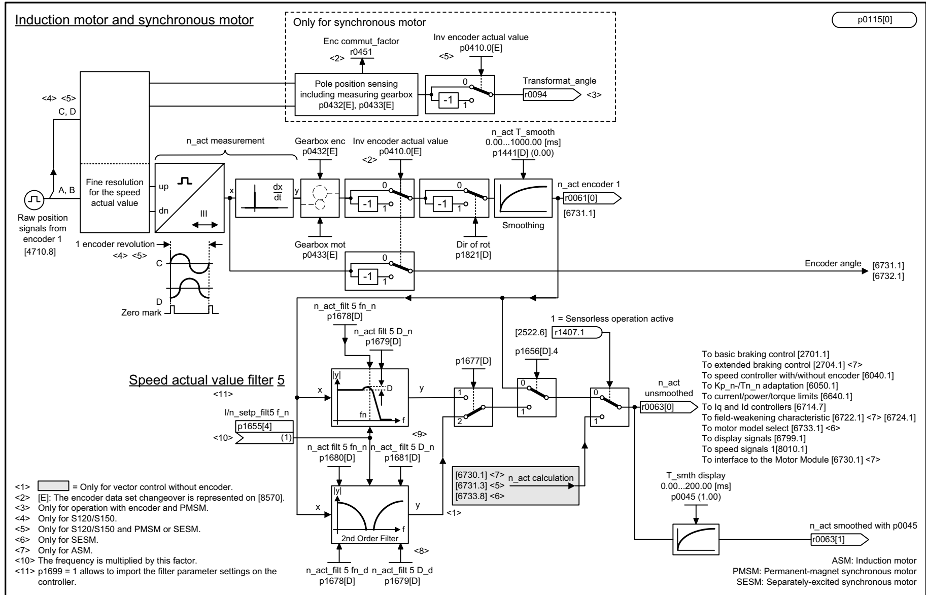
Fig. 3-192 4715 – Speed actual value and pole position sensing encoders 1, n_act_filter 5
