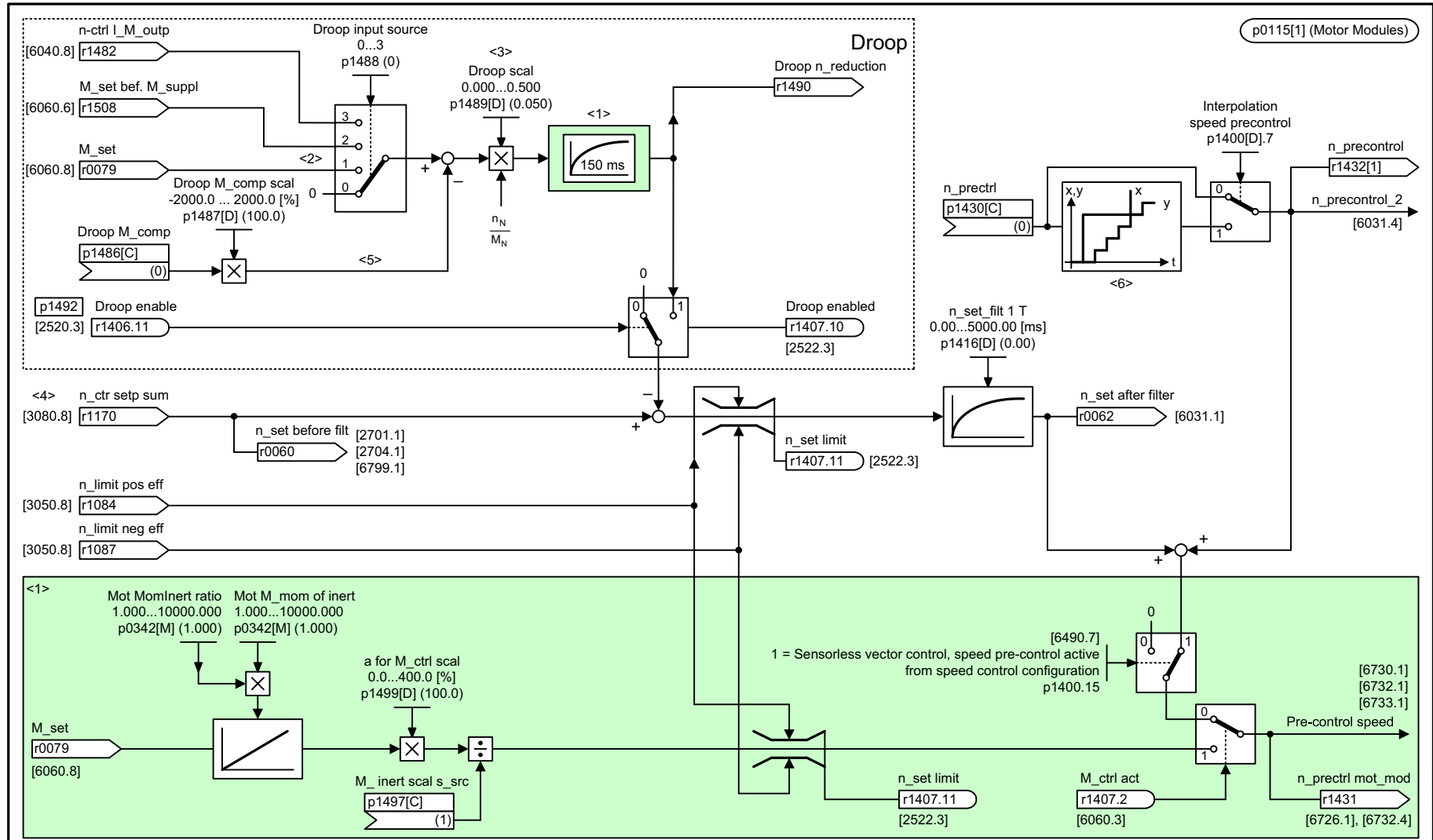
Fig. 3-234 6030 – Speed setpoint, droop
