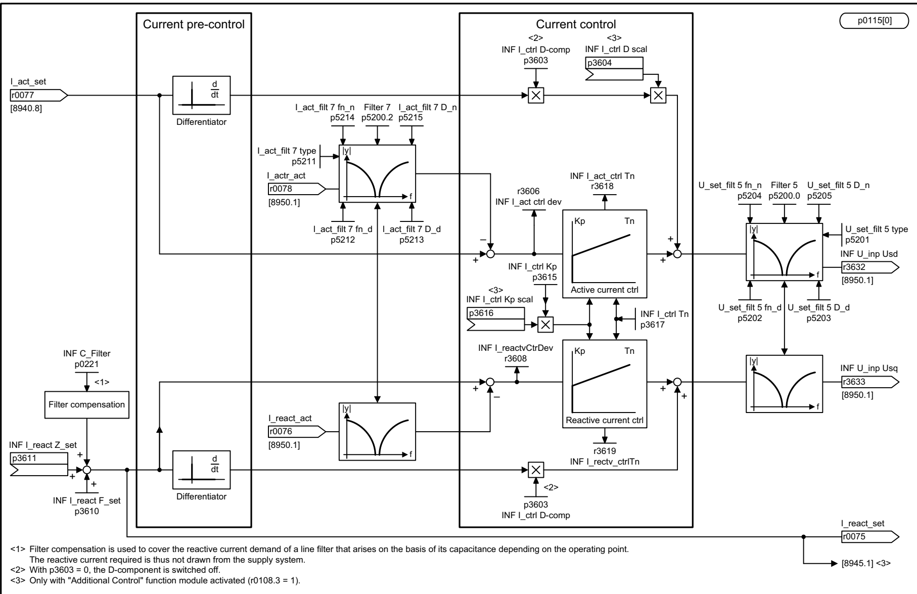
Fig. 3-350 8946 – Current pre-control/current controller/gating unit (p3400.0 = 0)
