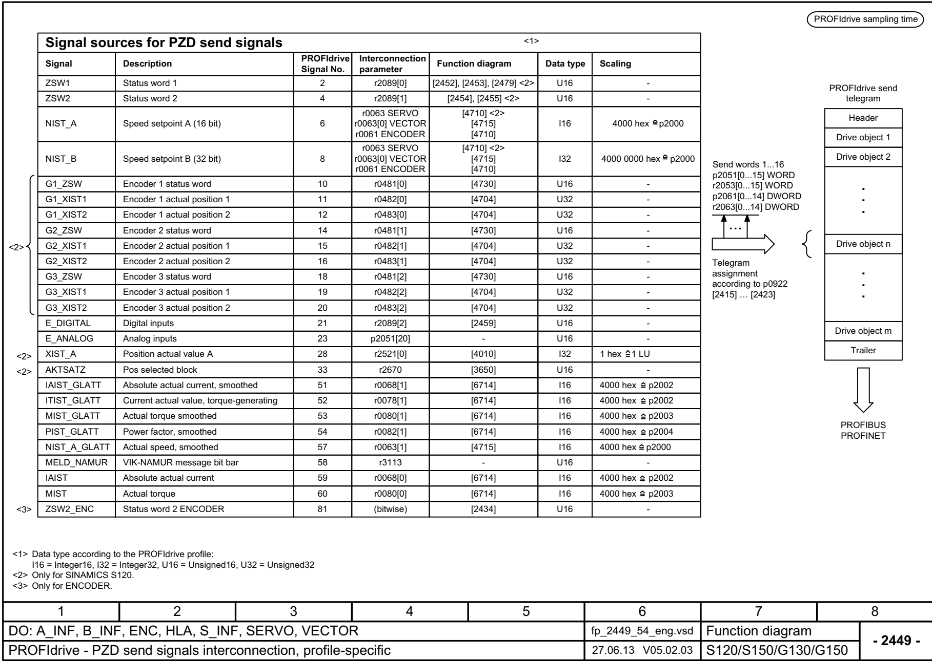
Fig. 3-60 2449 – PZD send signals interconnection profile-specific
