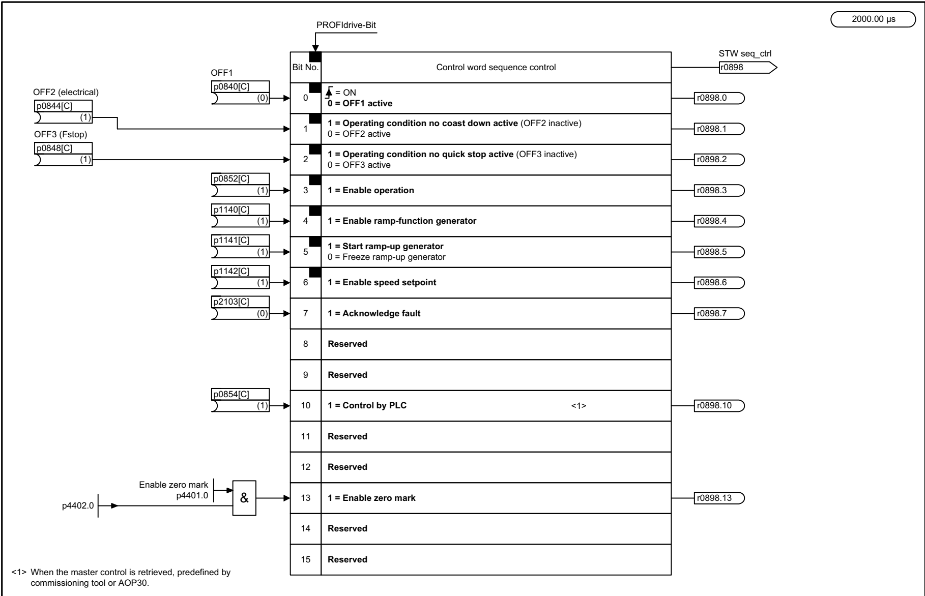
Fig. 3-397 9678 – Control word sequence control (p4400 = 0)
