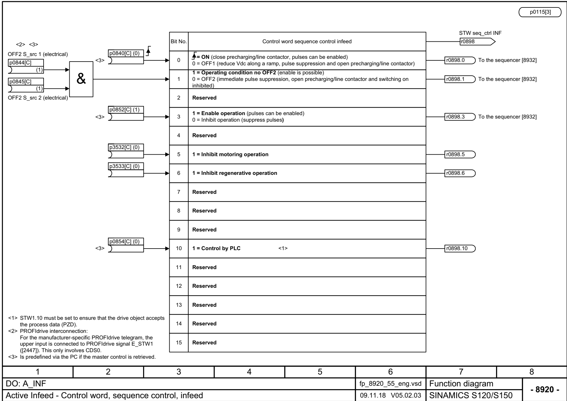
Fig. 3-343 8920 – Control word sequence control infeed
