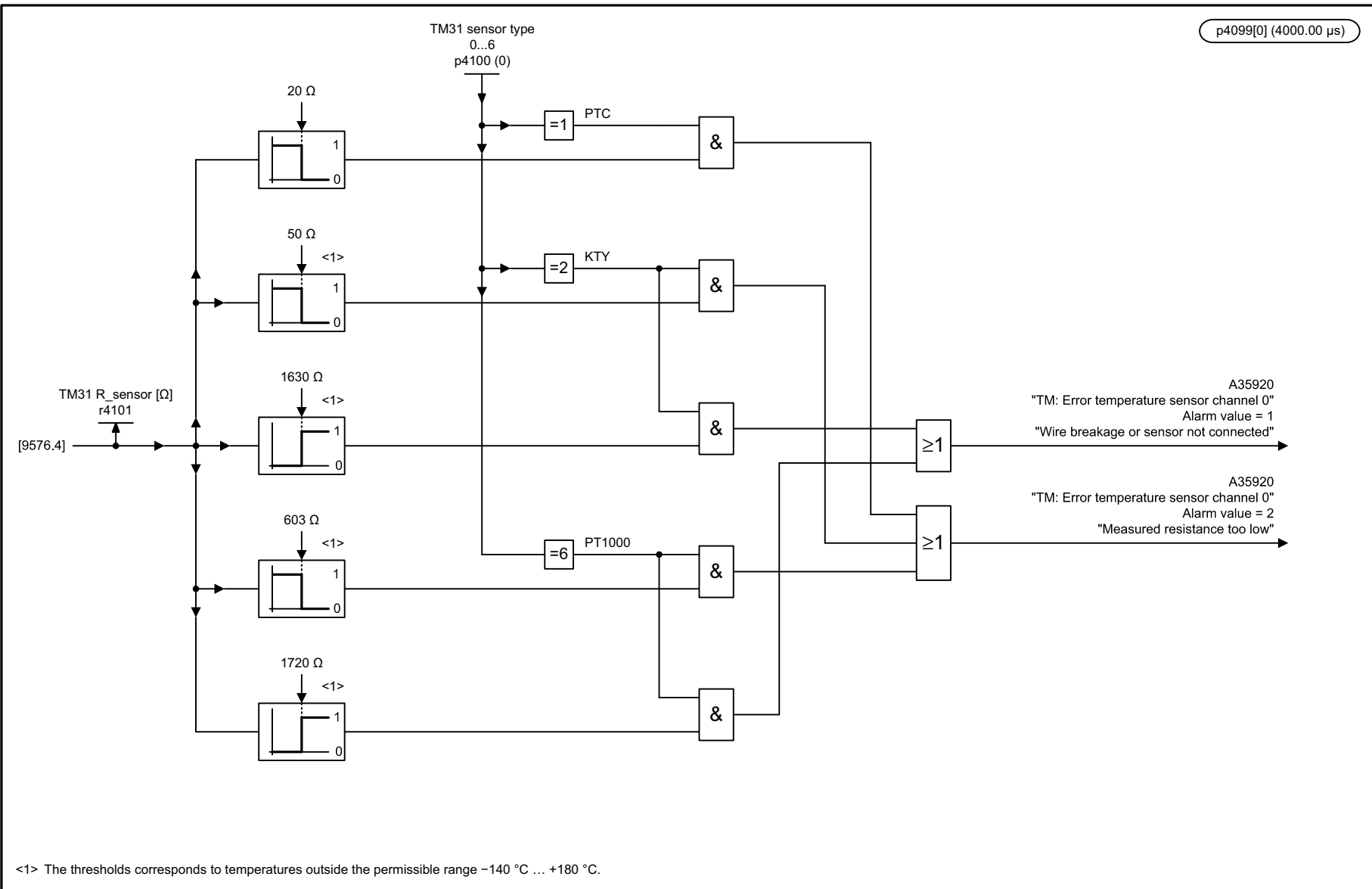
Fig. 3-383 9577 – Sensor monitoring KTY/PTC/PT1000
