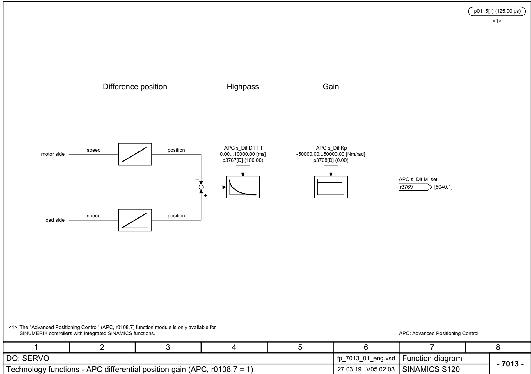
Fig. 3-271 7013 – APC differential position gain (APC, r0108.7 = 1)
