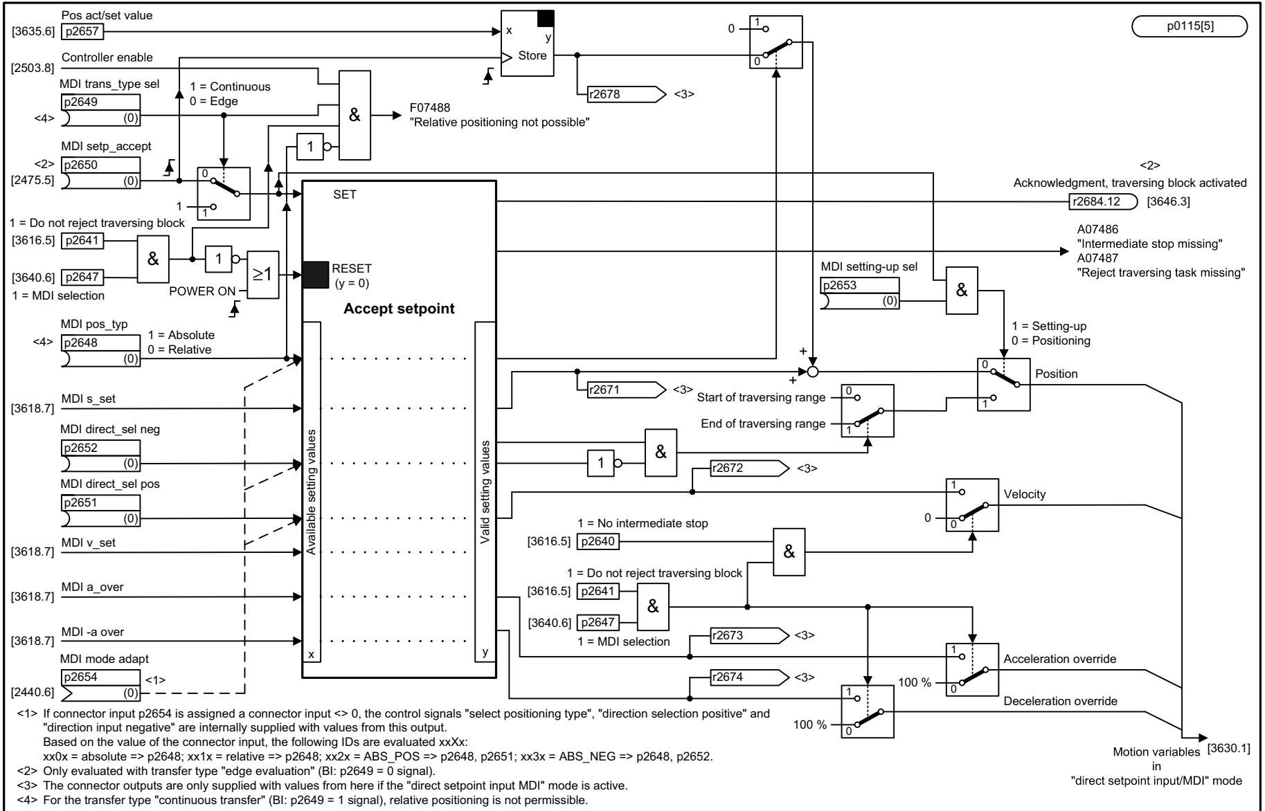
Fig. 3-175 3620 - Direct setpoint input/MDI mode (r0108.4 = 1)
