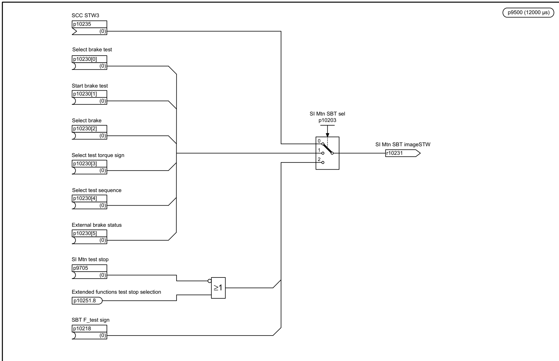
Fig. 3-128 2837 – Selection of active control word
