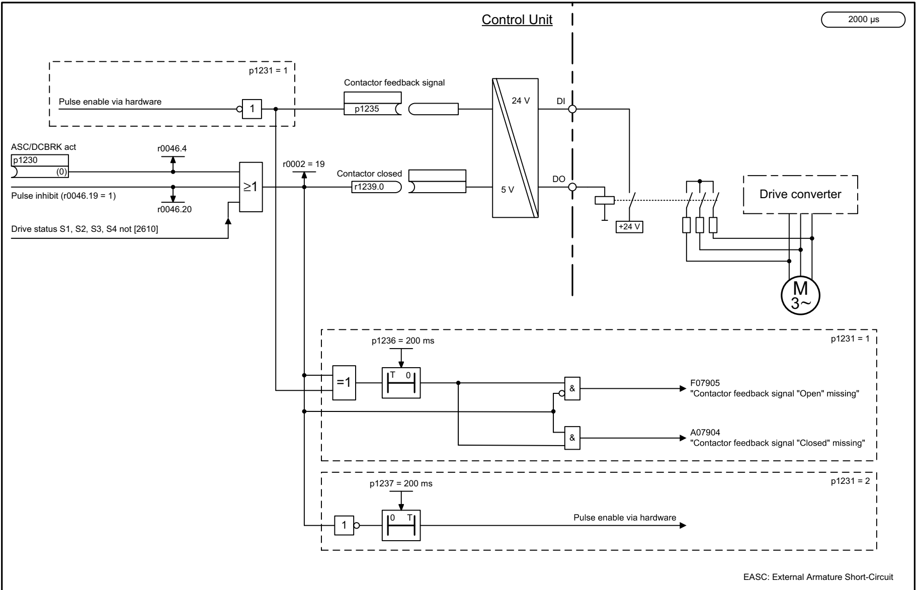
Fig. 3-272 7014 – External armature short circuit (EASC, p0300 = 2xx or 4xx)
