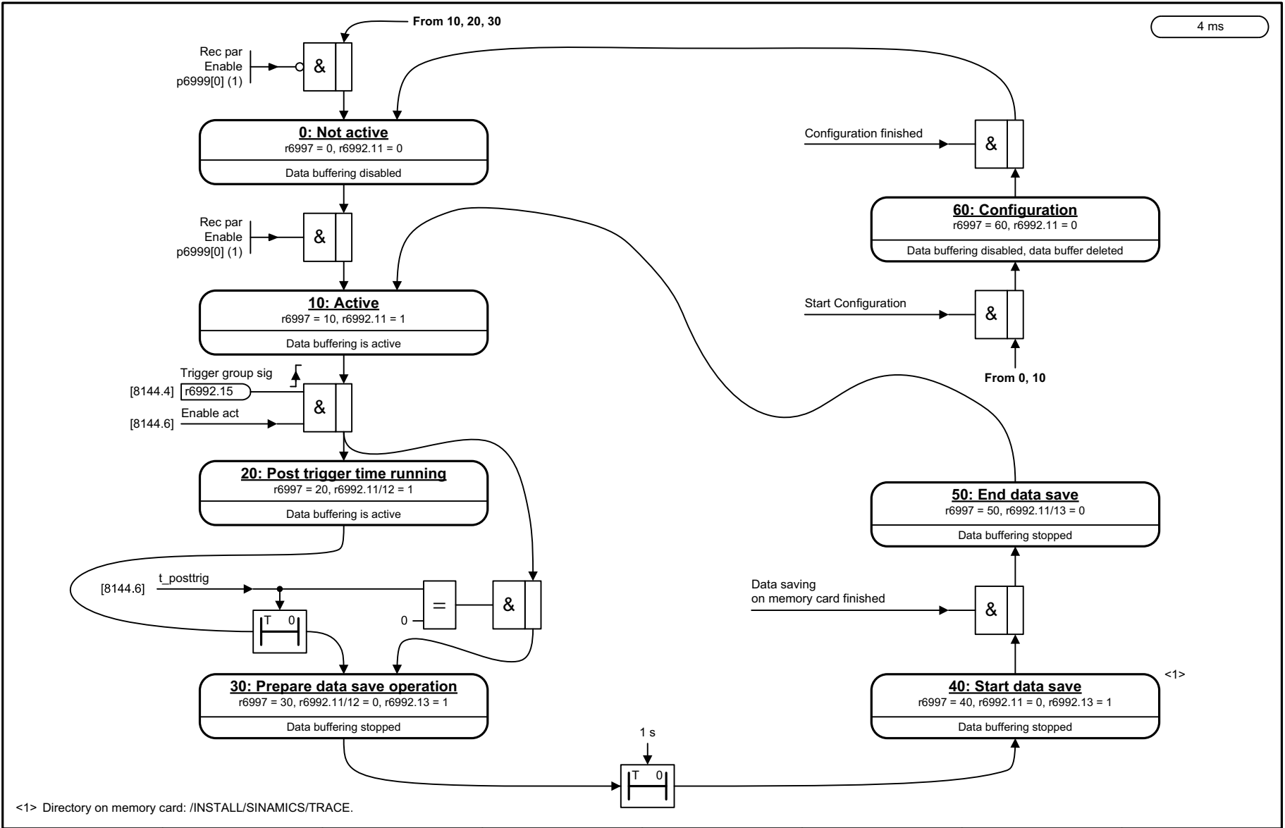
Fig. 3-320 8145 – Recorder sequence control (r0108.5 = 1)
