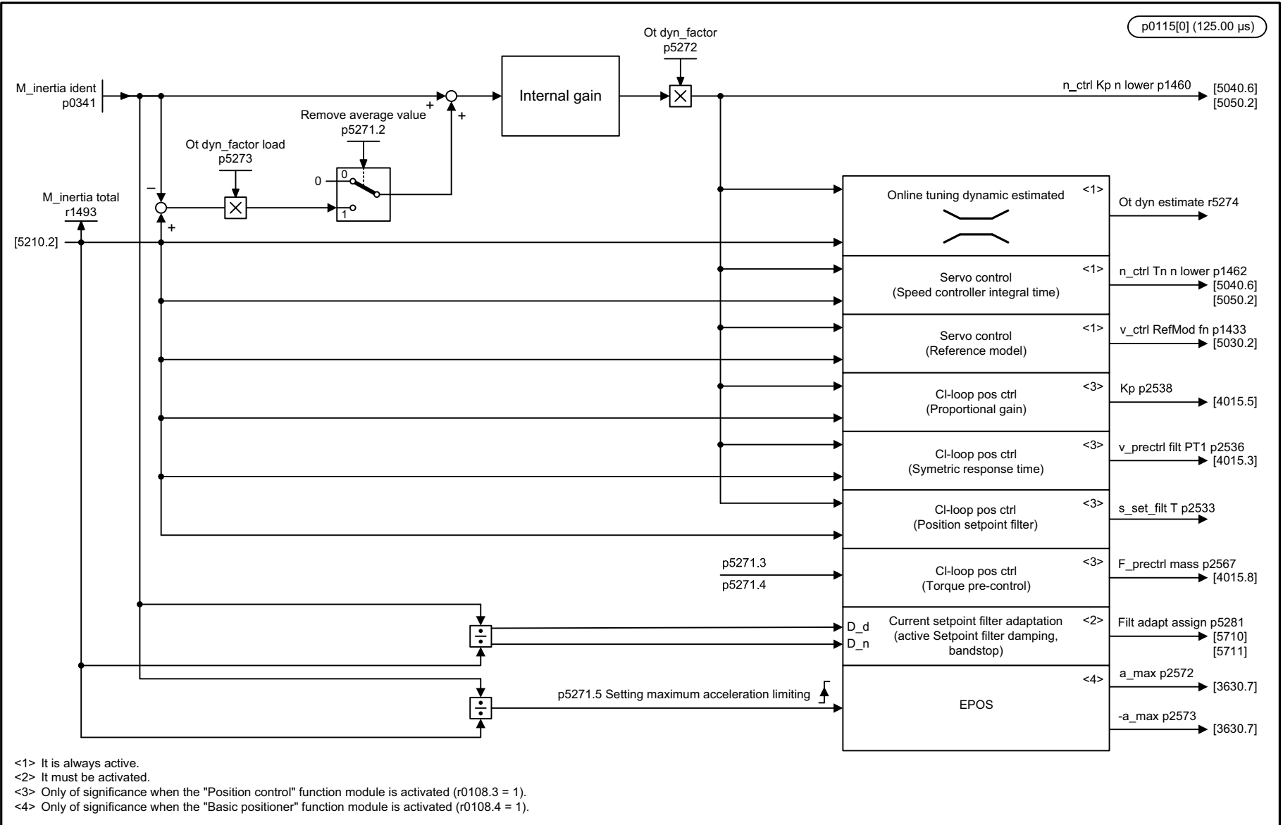
Fig. 3-213 5045 – Online tuning with activated moment of inertia estimator (r0108.10 = 1)
