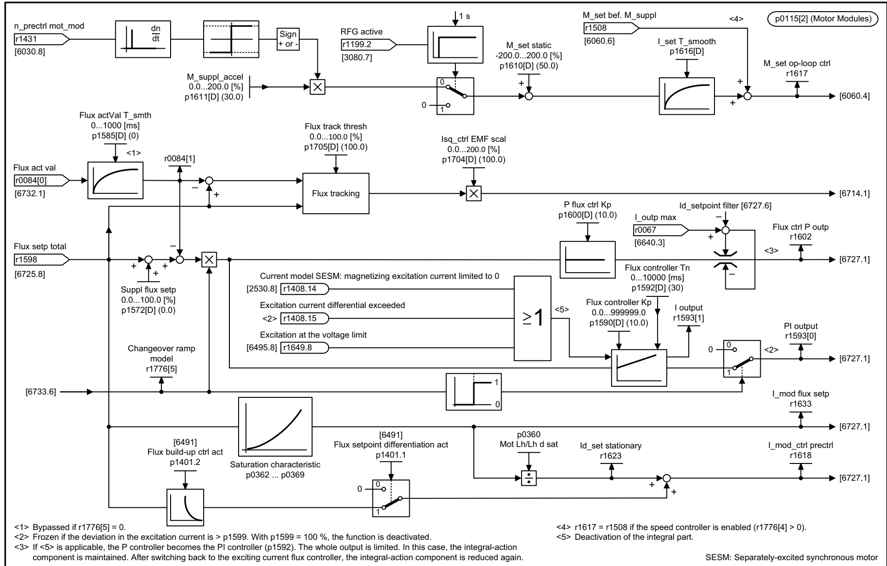
Fig. 3-258 6726 – Field weakening controller, flux controller (SESM, p0300 = 5)
