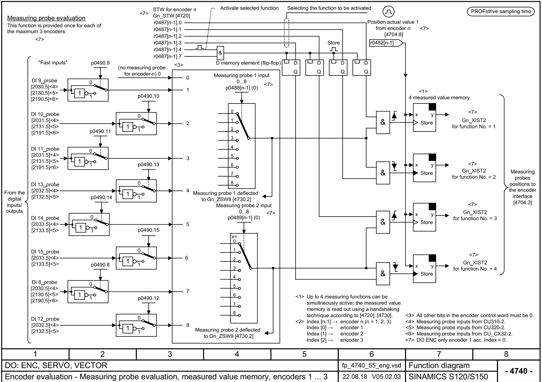
Fig. 3-196 4/740 – Measuring probe evaluation, measured value memory, encoders 1 ... 3
