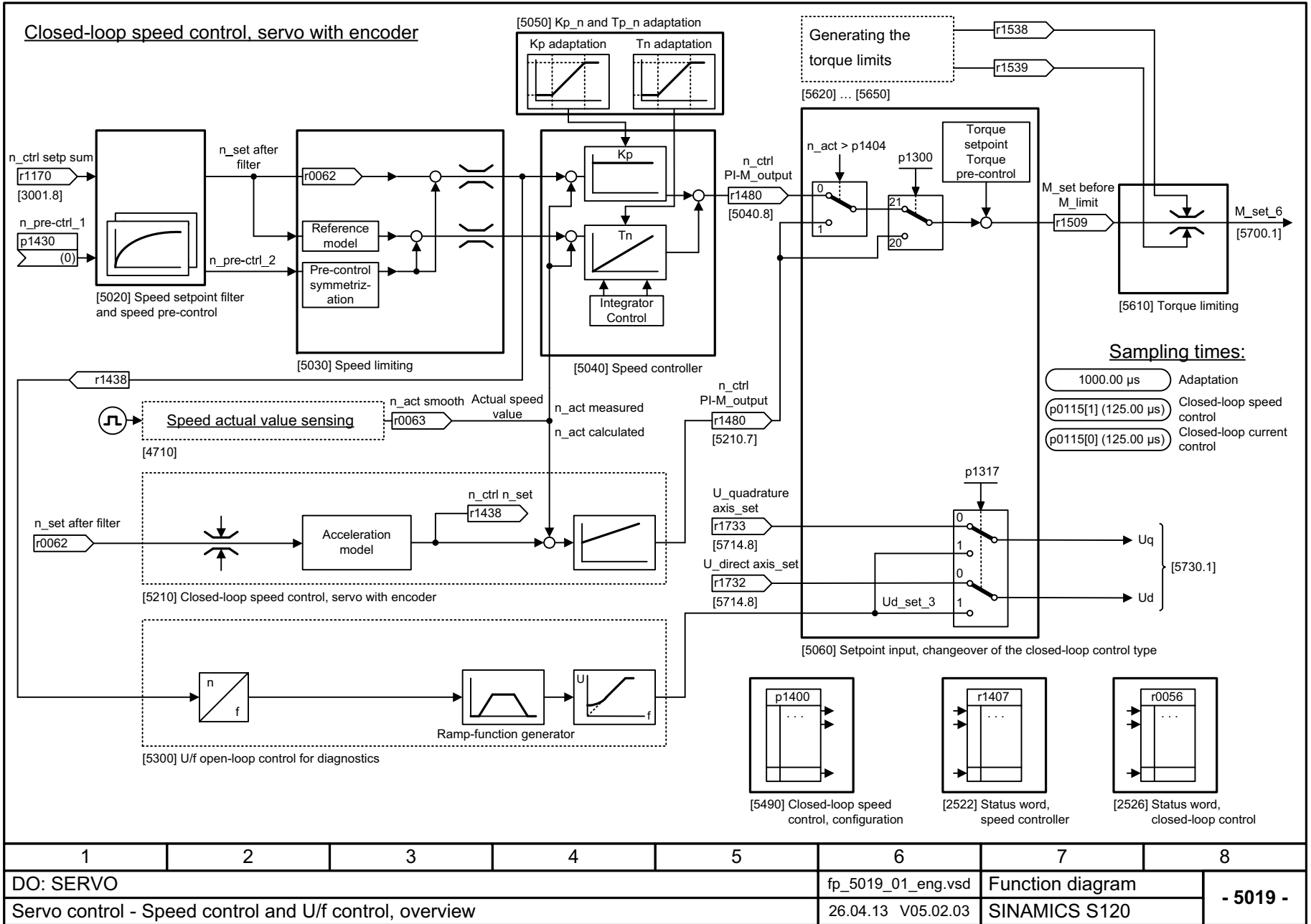
Fig. 3-207 5019 – Closed-loop speed control and U/f control, overview
