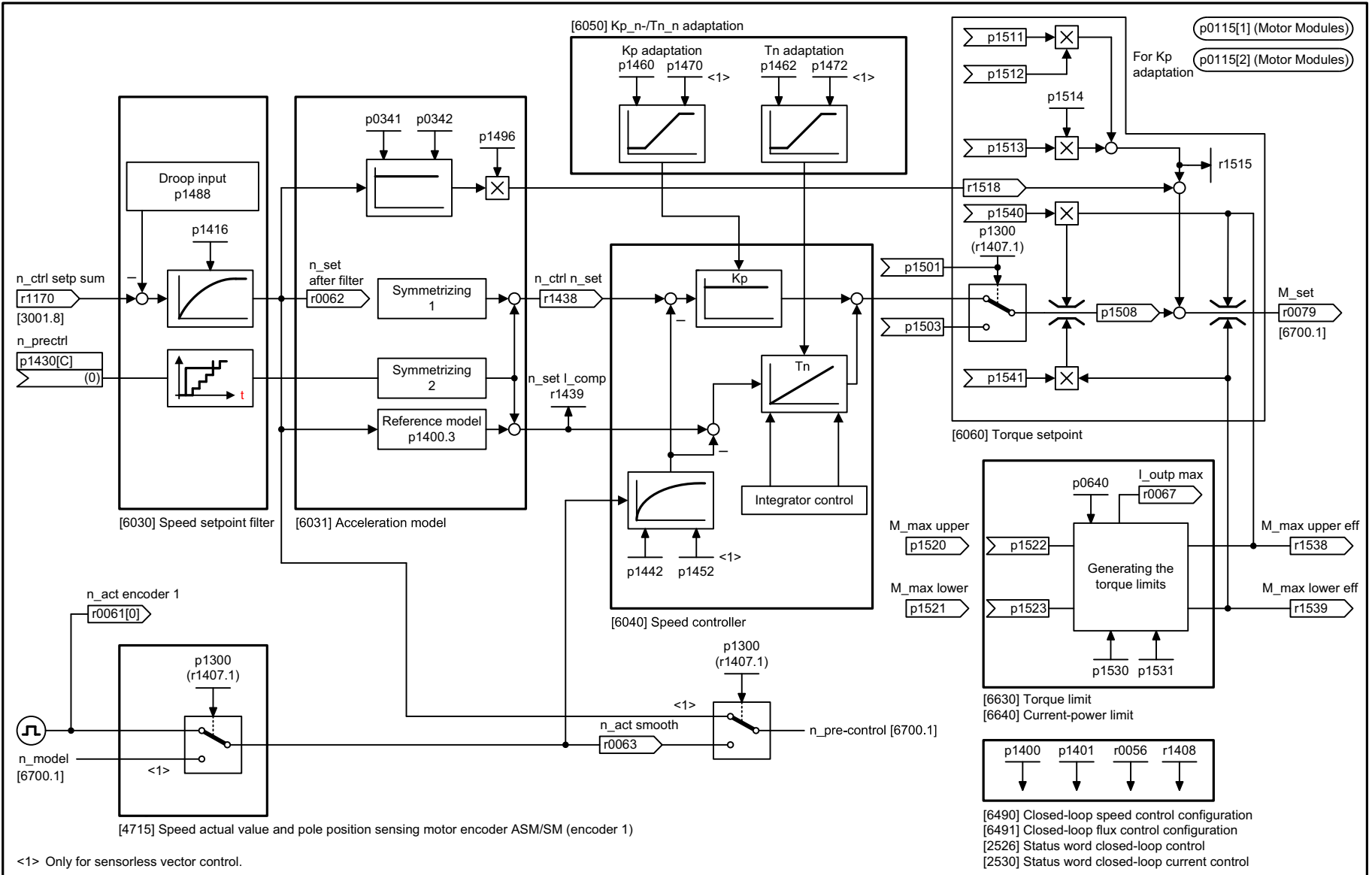
Fig. 3-233 6020 – Closed-loop speed control and generation of the torque limits, overview
