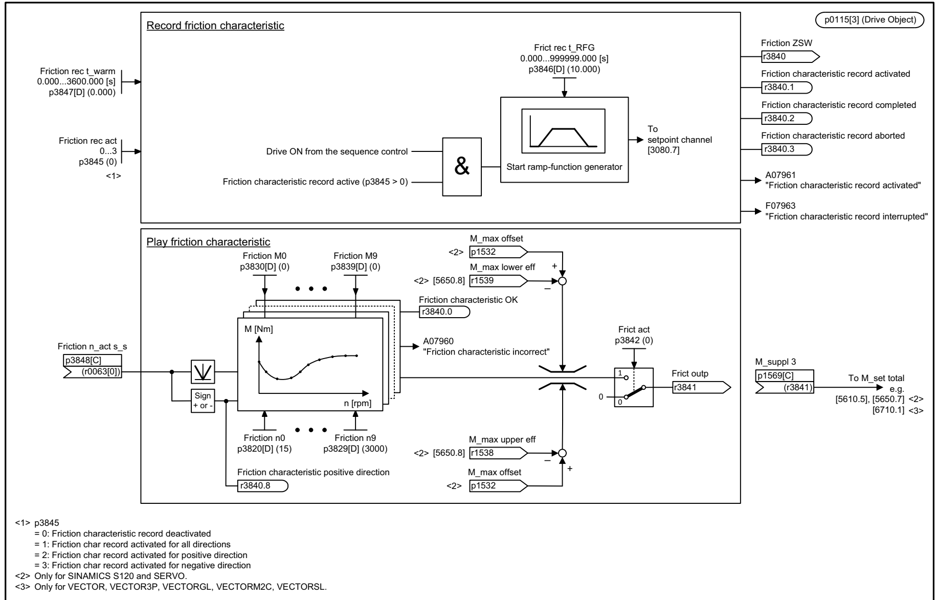
Fig. 3-269 7010 – Friction characteristic
