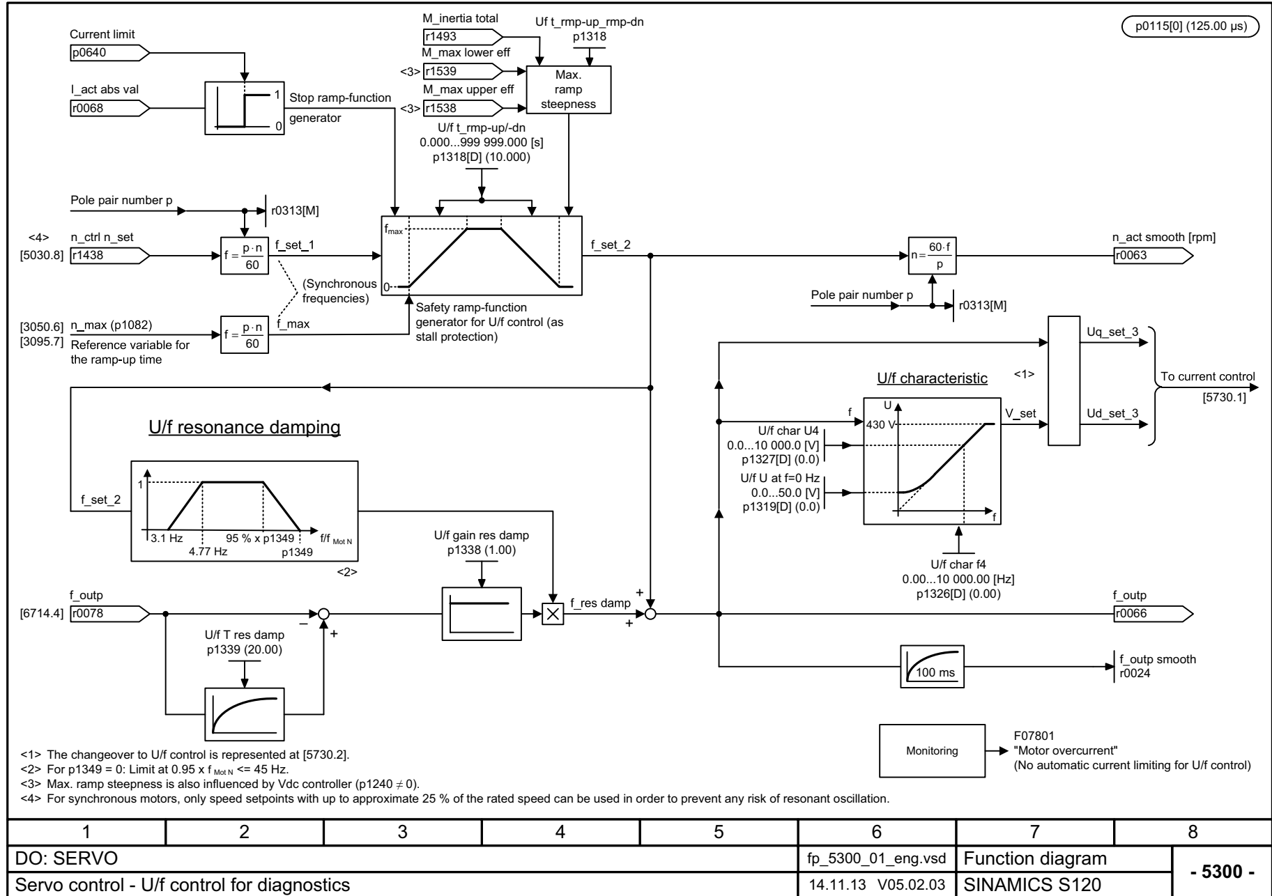
Fig. 3-218 5300 – U/f control for diagnostics
