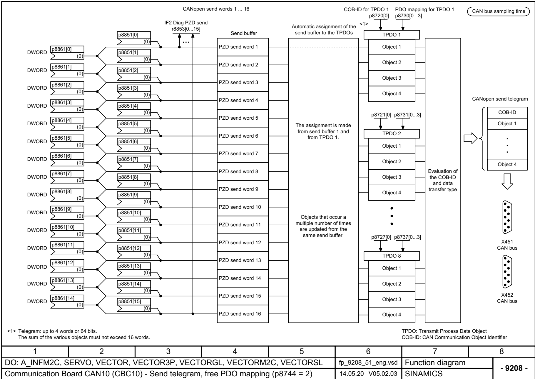
Fig. 3-363 9208 – Send telegram free PDO mapping (p8744 = 2)
