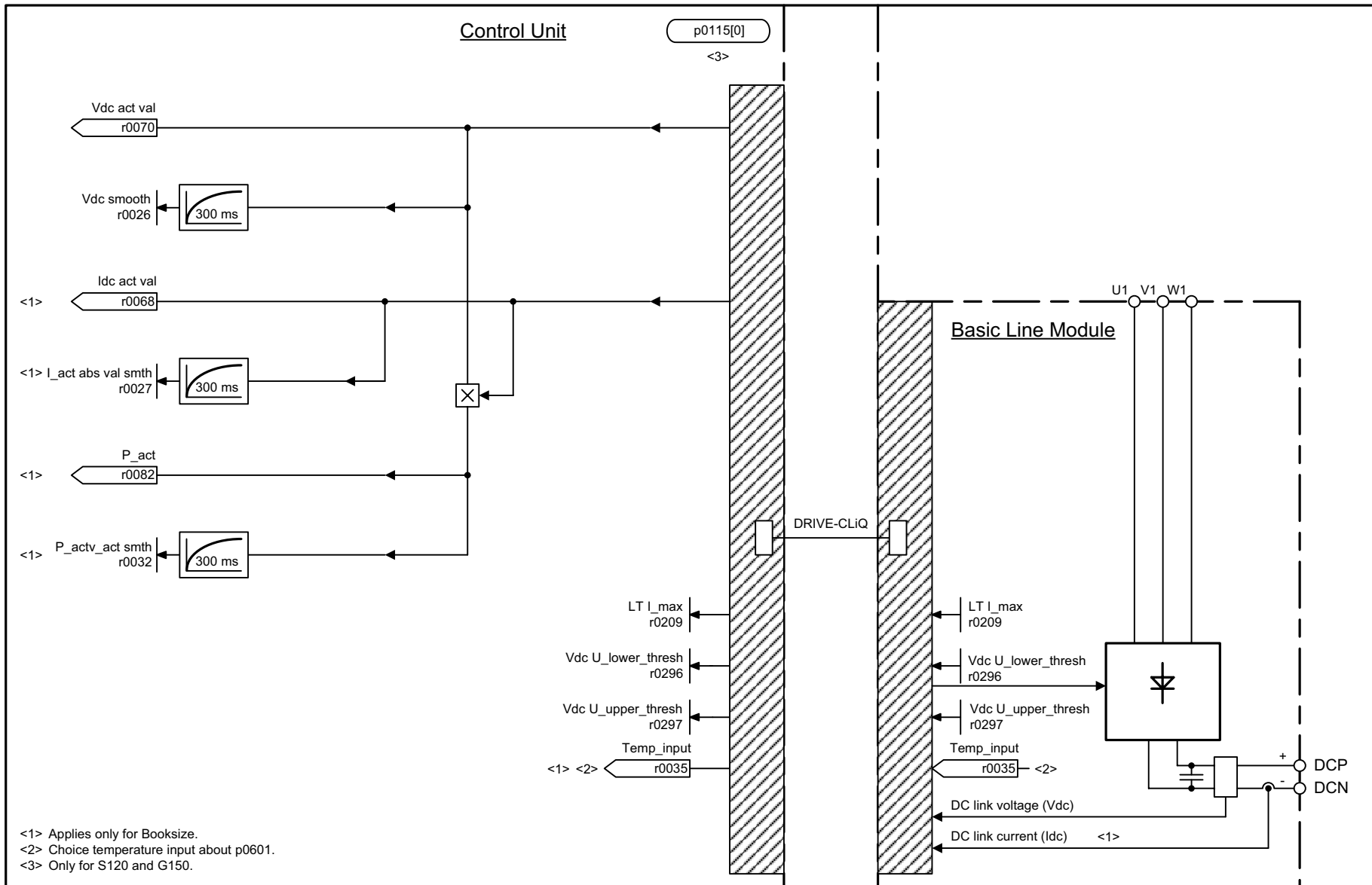
Fig. 3-331 8750 – Interface to the Basic Infeed power unit (control signals, actual values)
