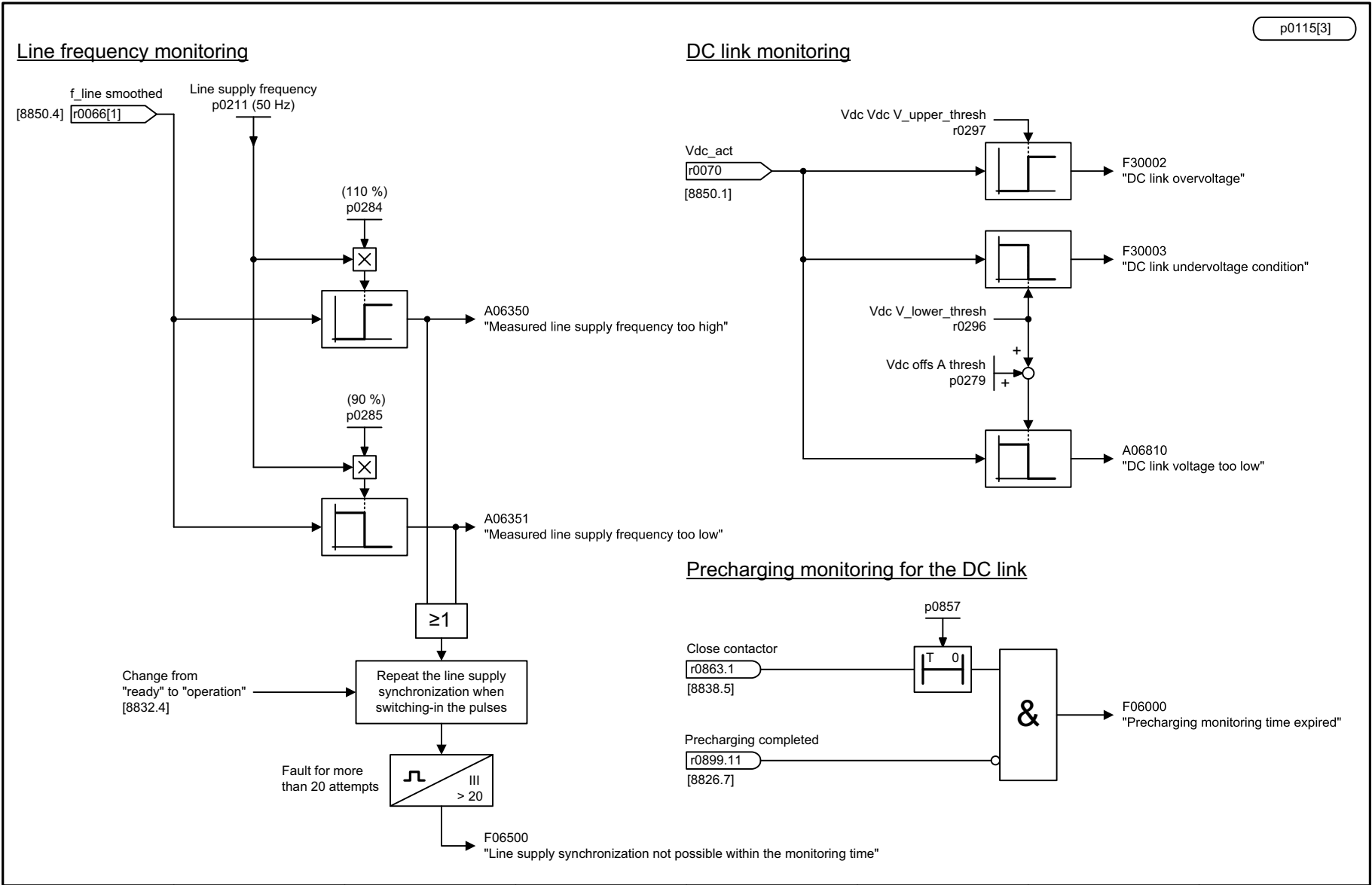
Fig. 3-341 8864 – Signals and monitoring functions, line frequency and Vdc monitoring
