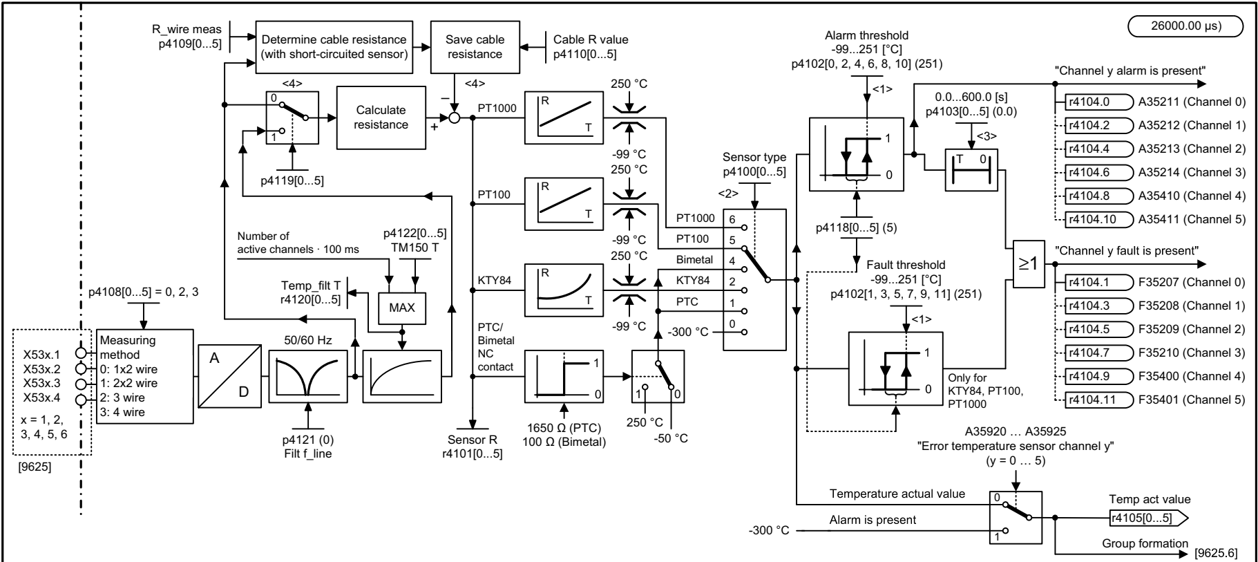
Fig. 3-387 9626 – Temperature evaluation 1x2, 3, 4 wire (channels 0 ... 5)
