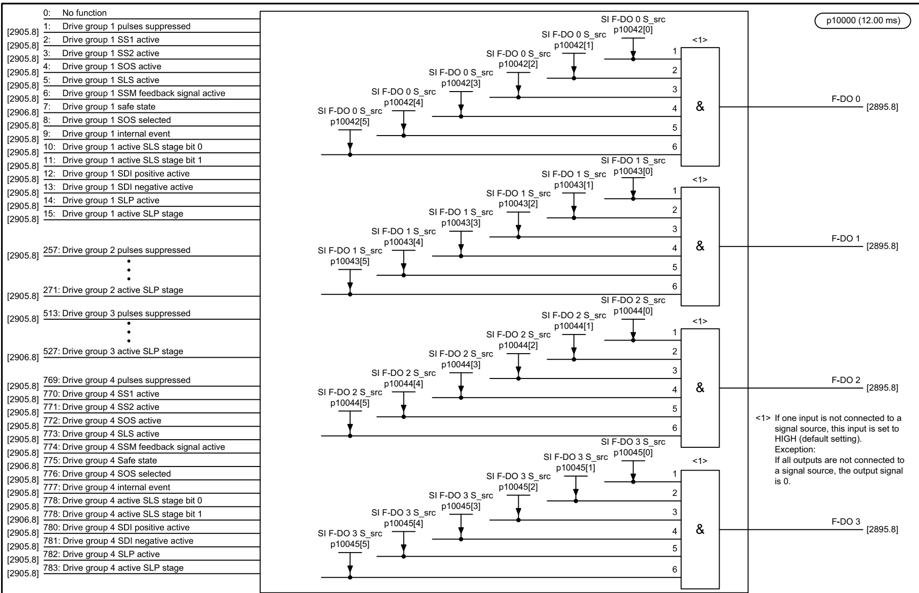
Fig. 3-153 2907 – Extended Functions assignment (F-DO 0 ... F-DO 3)
