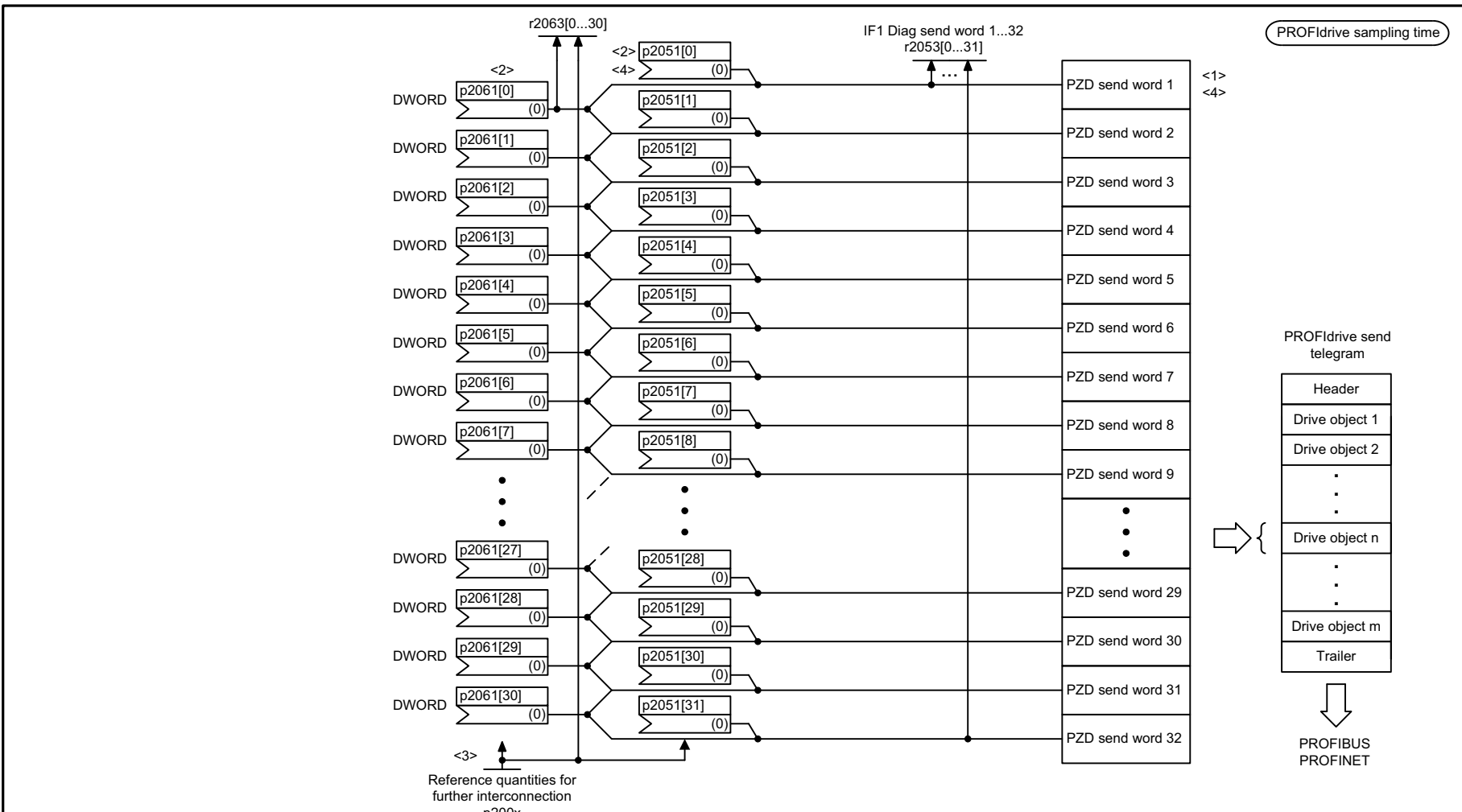
Fig. 3-76 2470 – IF1 send telegram free interconnection via BICO (p0922 = 999)
