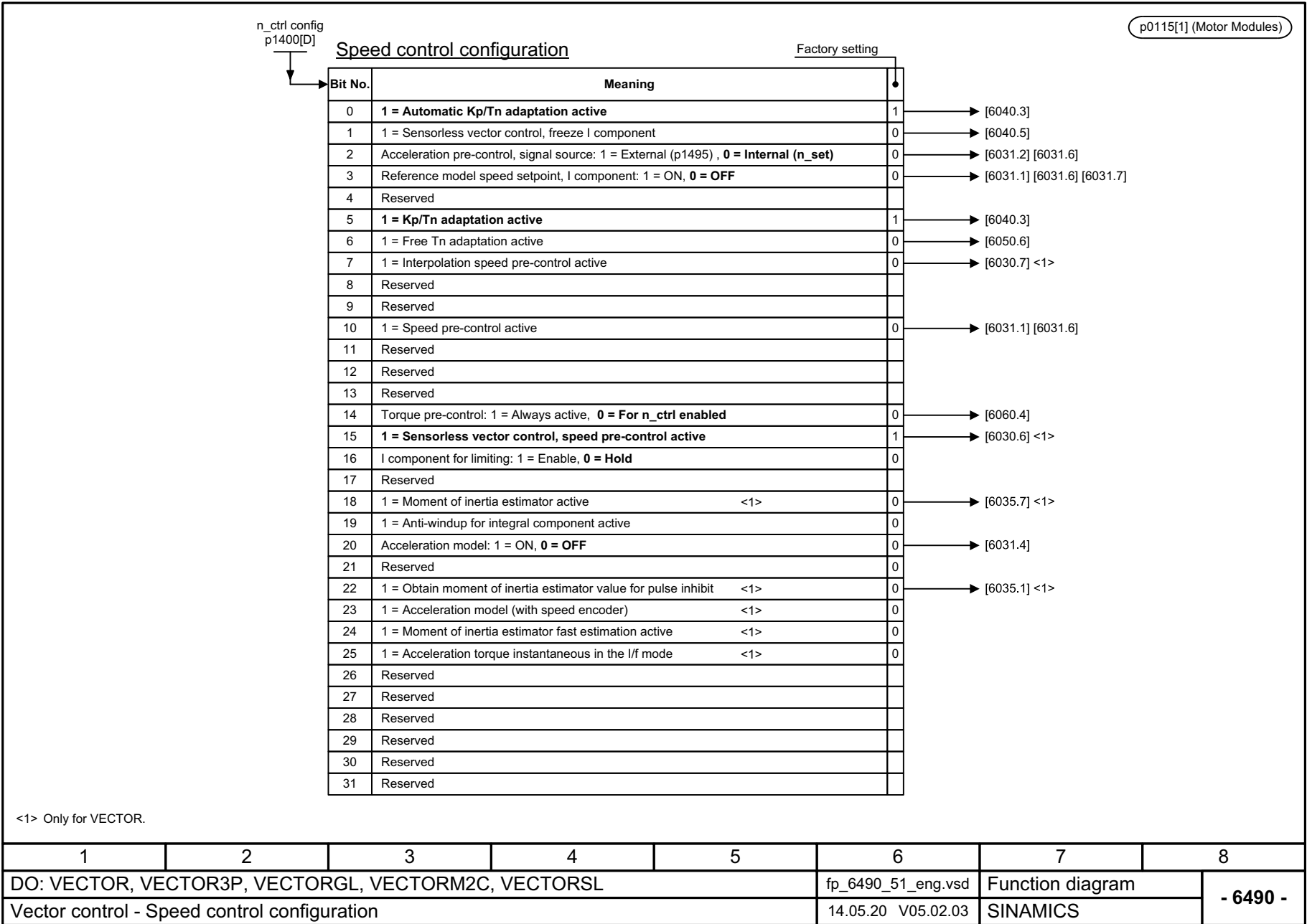
Fig. 3-245 6490 – Closed-loop speed control configuration
