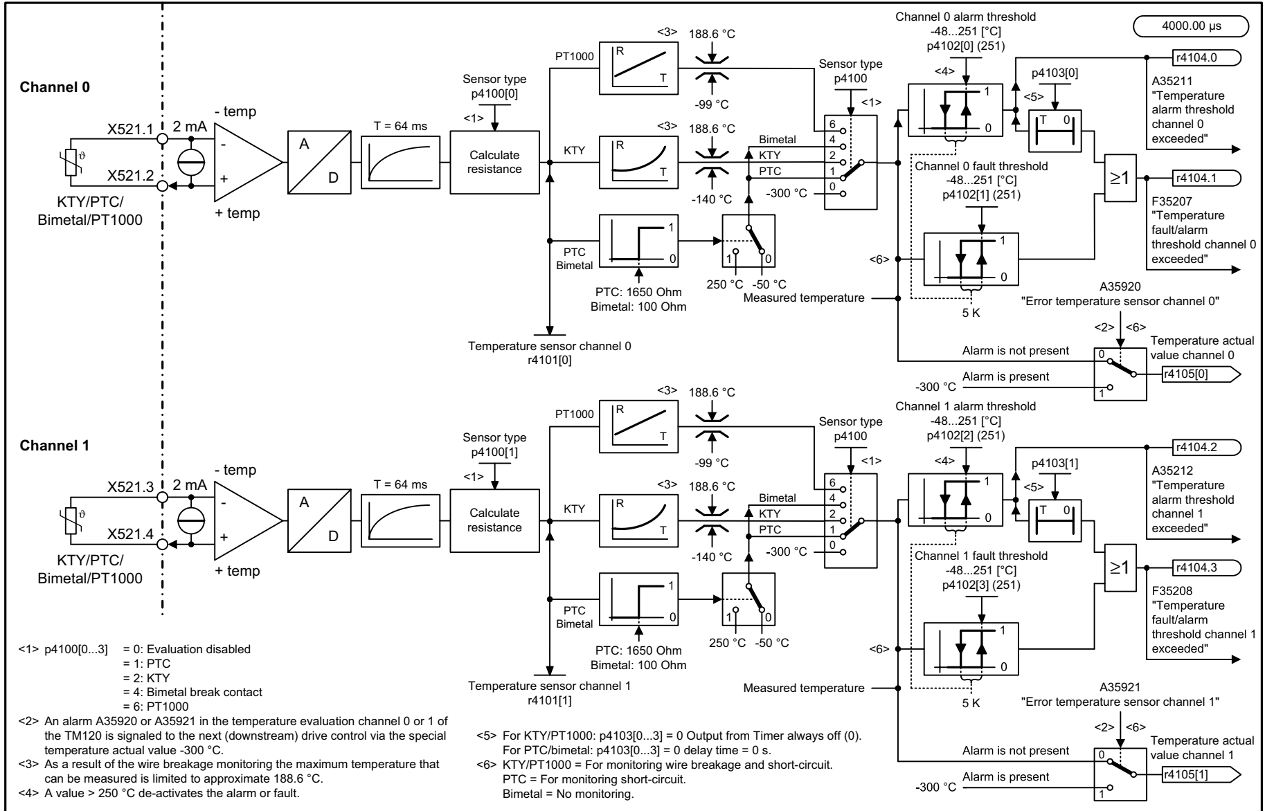
Fig. 3-384 9605 - Temperature evaluation channels 0 and 1
