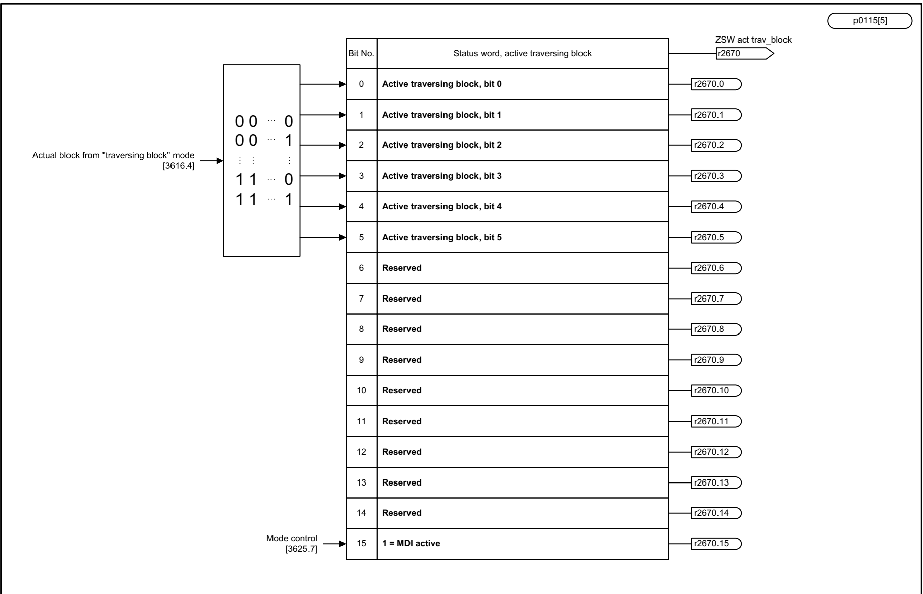
Fig. 3-182 3650 – Status word active traversing block/MDI active (r0108.4 = 1)
