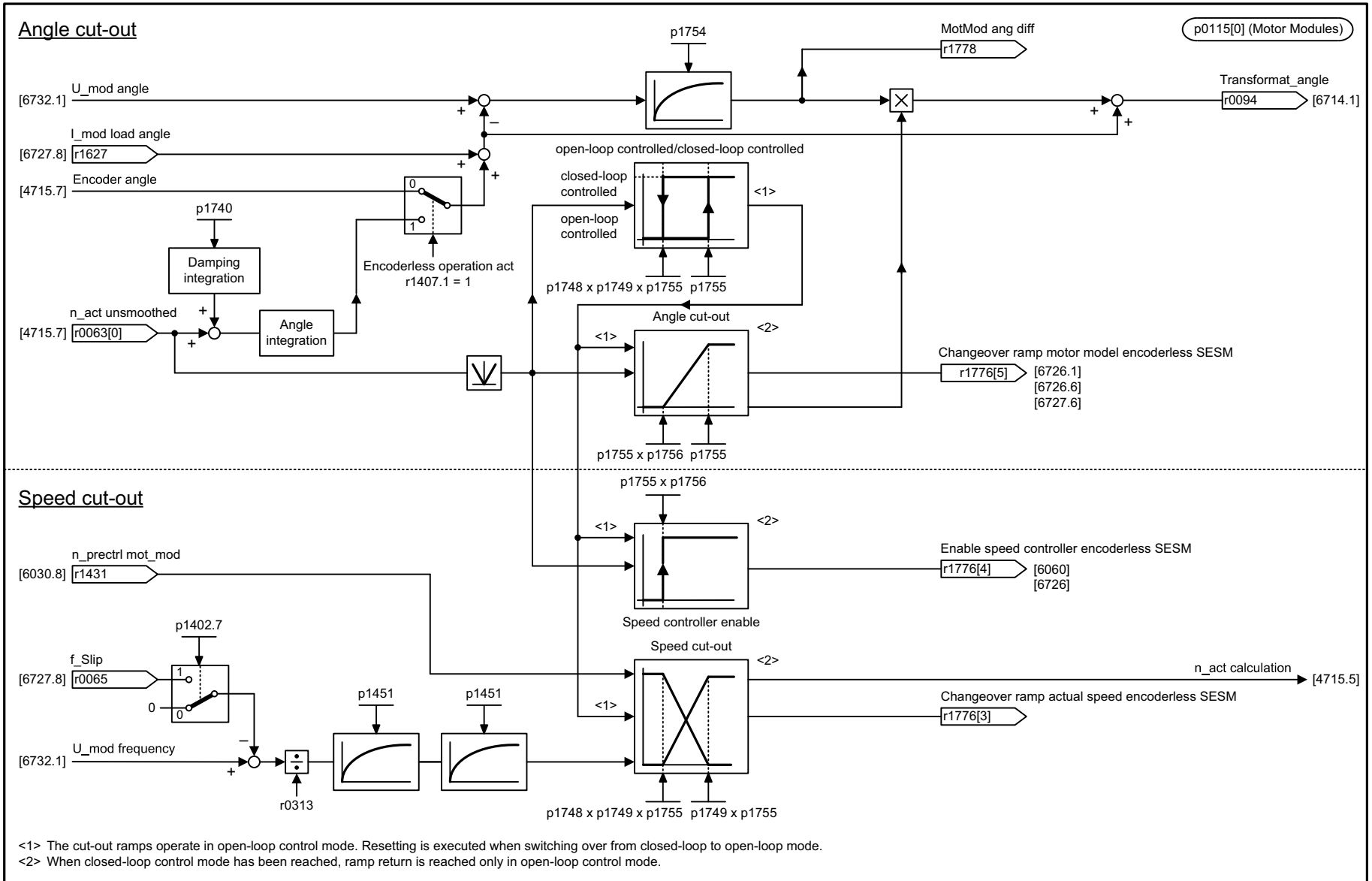
Fig. 3-263 6733 – Motor model selection (SESM and p1300 = 20, p0300 = 5)
