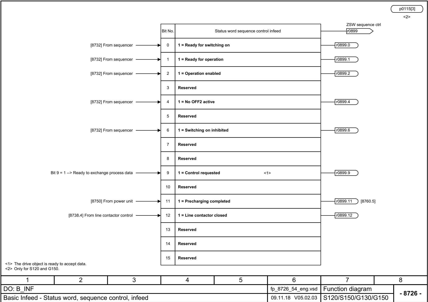
Fig. 3-328 8726 – Status word sequence control infeed
