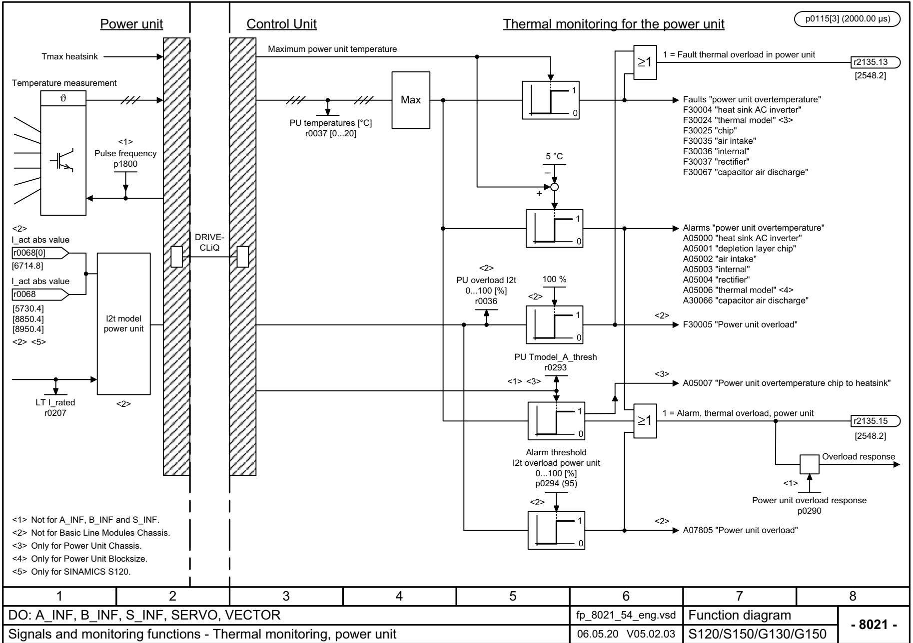
Fig. 3-311 8021 – Thermal monitoring, power unit
