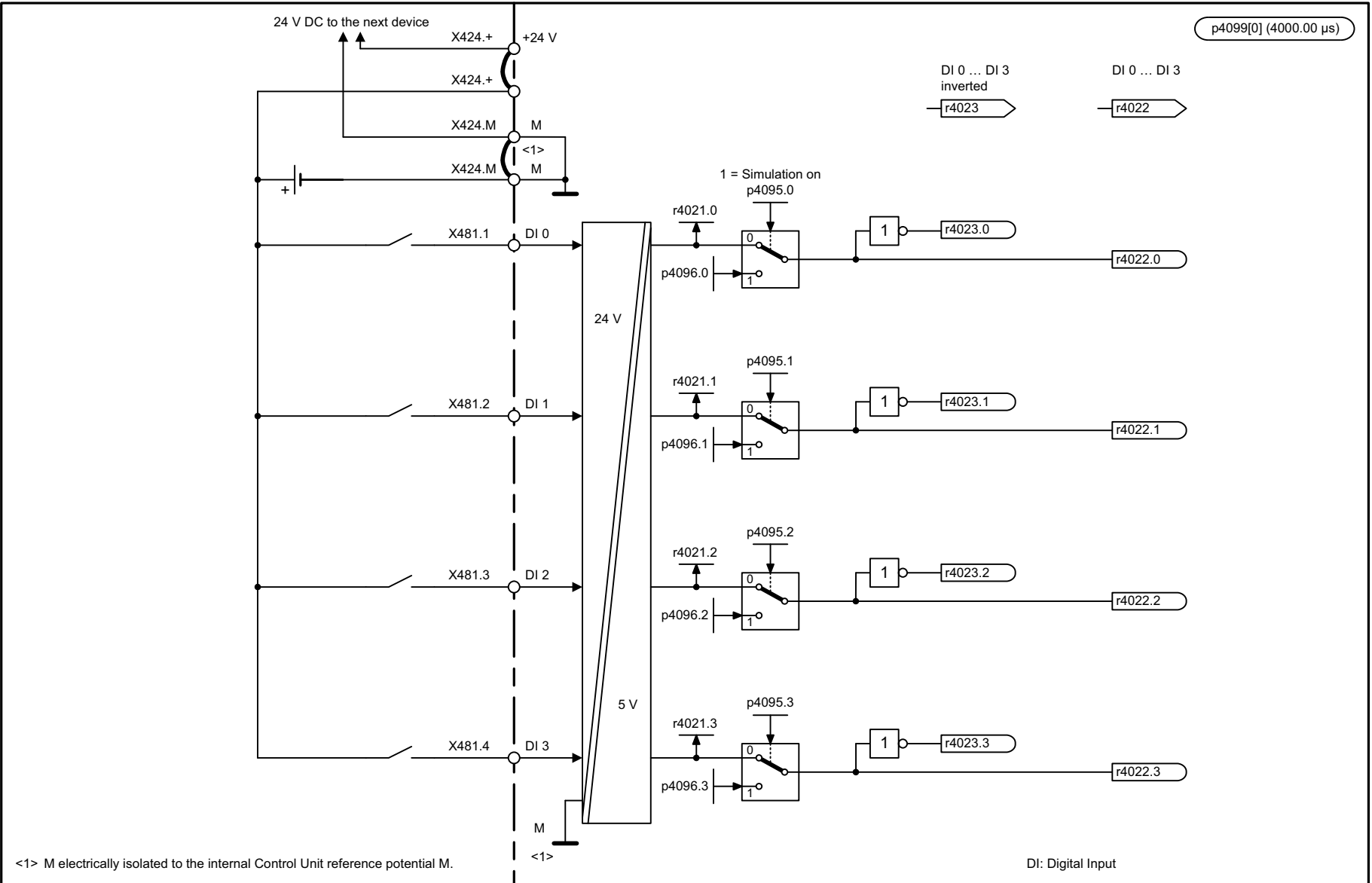
Fig. 3-357 9100 – Digital inputs electrically isolated (DI 0 ... DI 3)
