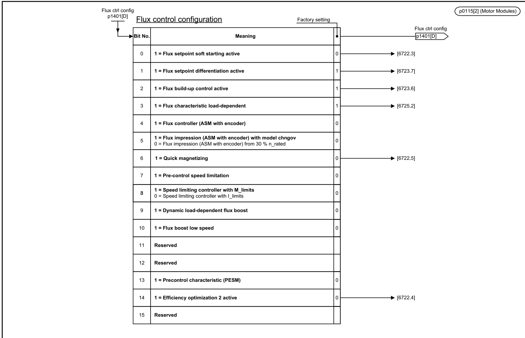
Fig. 3-246 6491 – Flux control configuration
