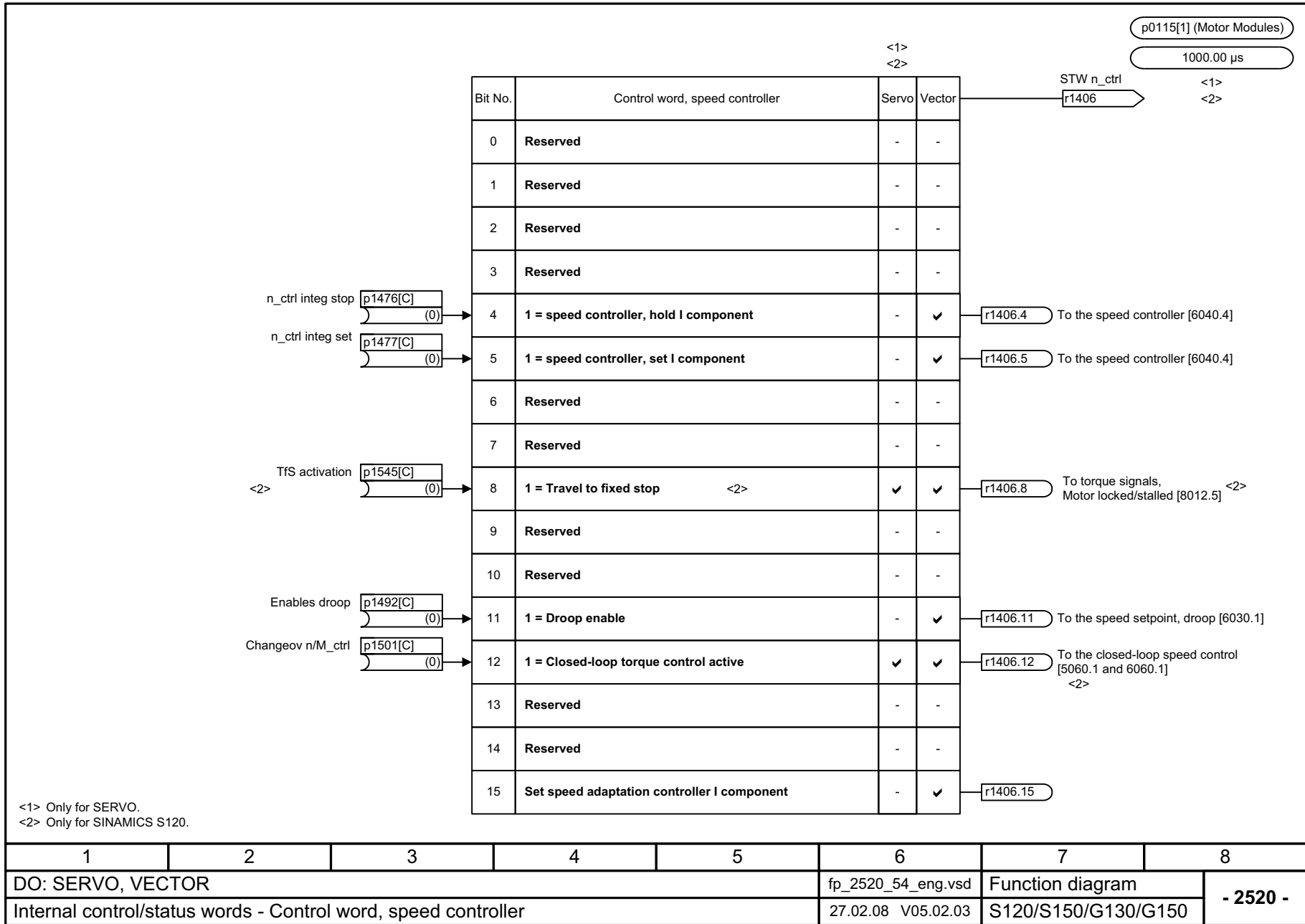
Fig. 3-98 2520 – Control word speed controller
