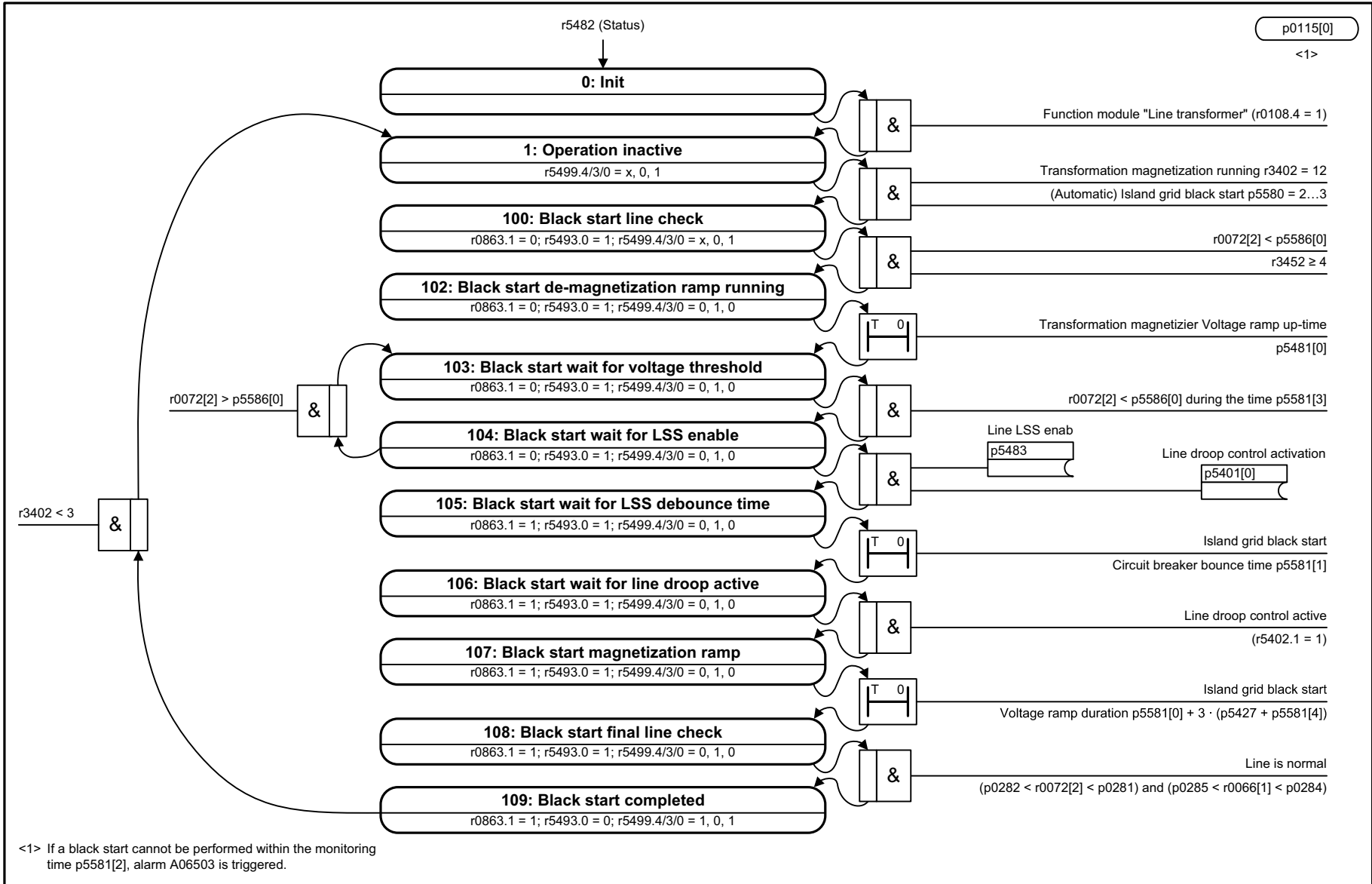
Fig. 3-288 7988 – Island grid black start sequence control
