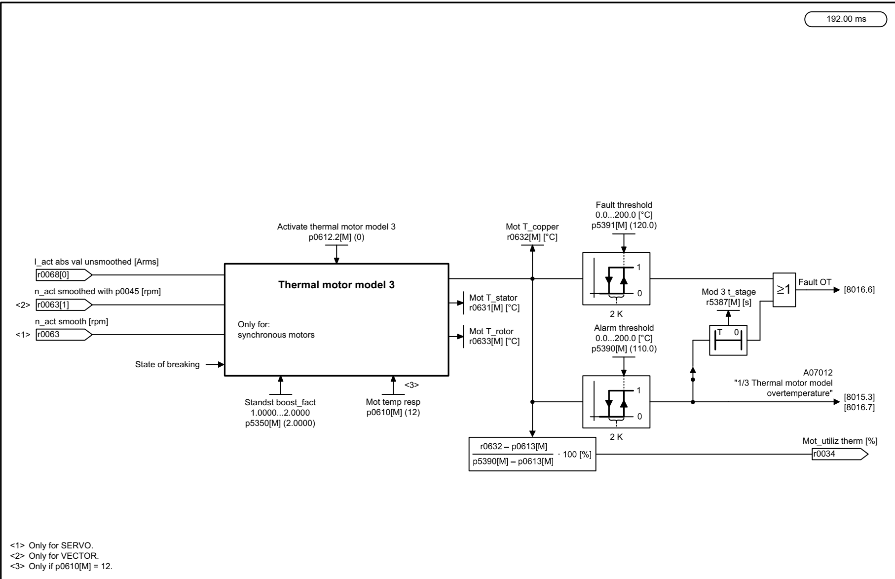
Fig. 3-309 8019 – Motor temperature model 3
