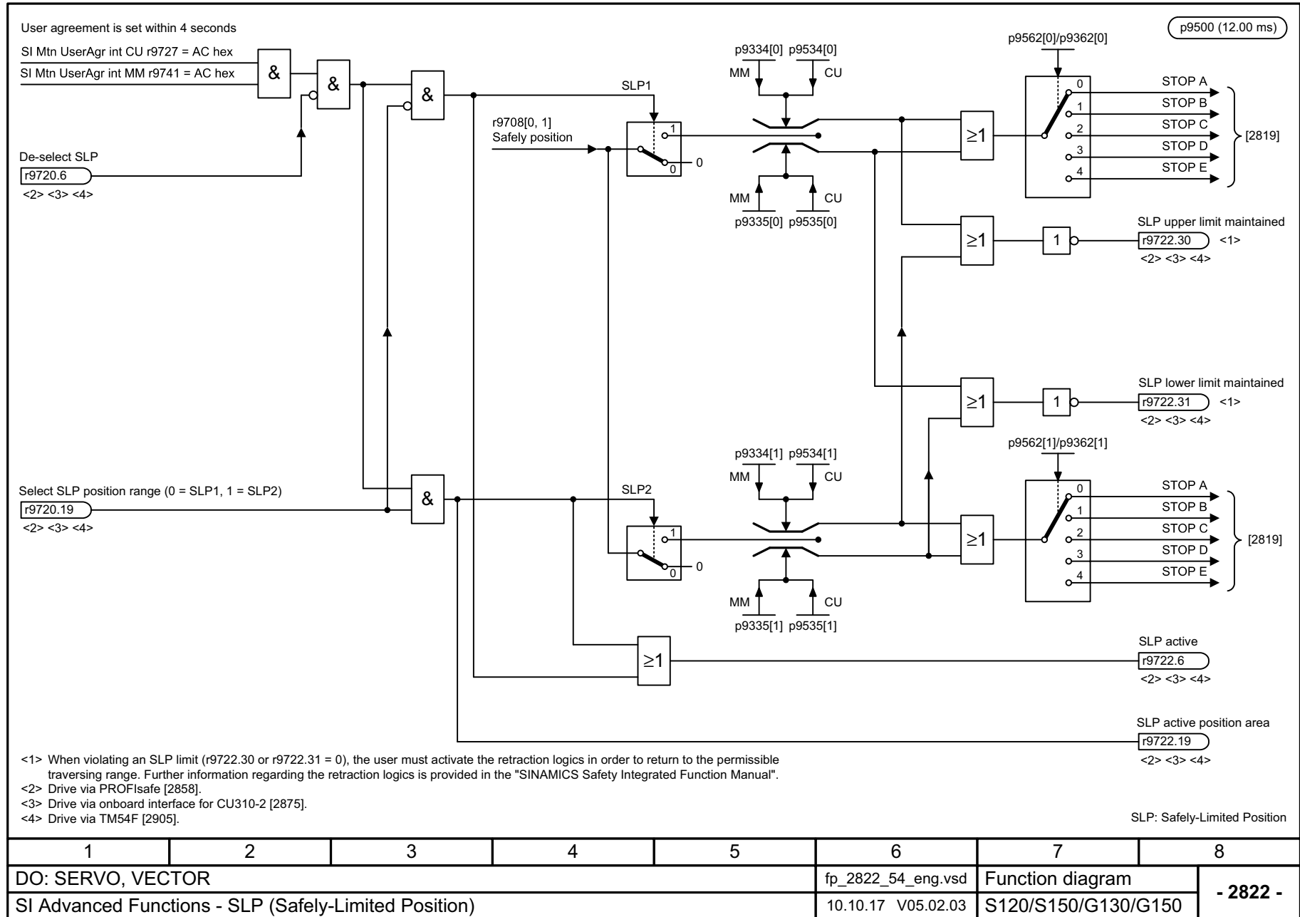
Fig. 3-139 2822 – SLP (Safely-Limited Position)
