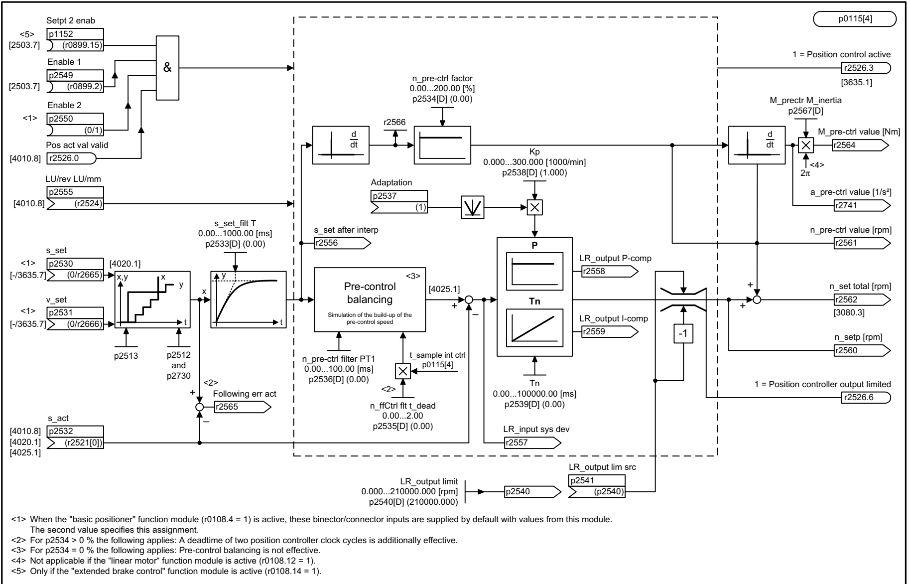
Fig. 3-184 4015 – Position controller (r0108.3 = 1)
