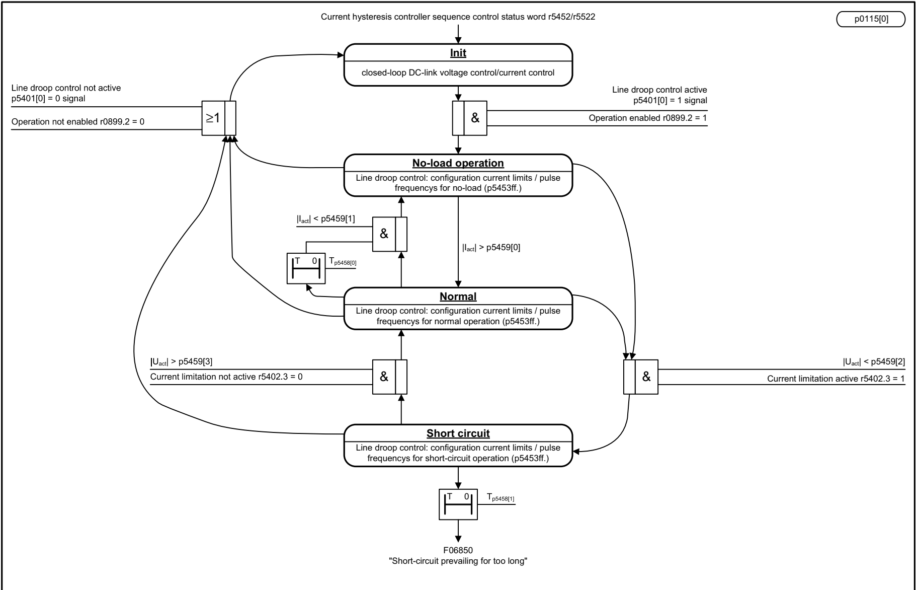
Fig. 3-286 7986 – Sequence control overcurrent
