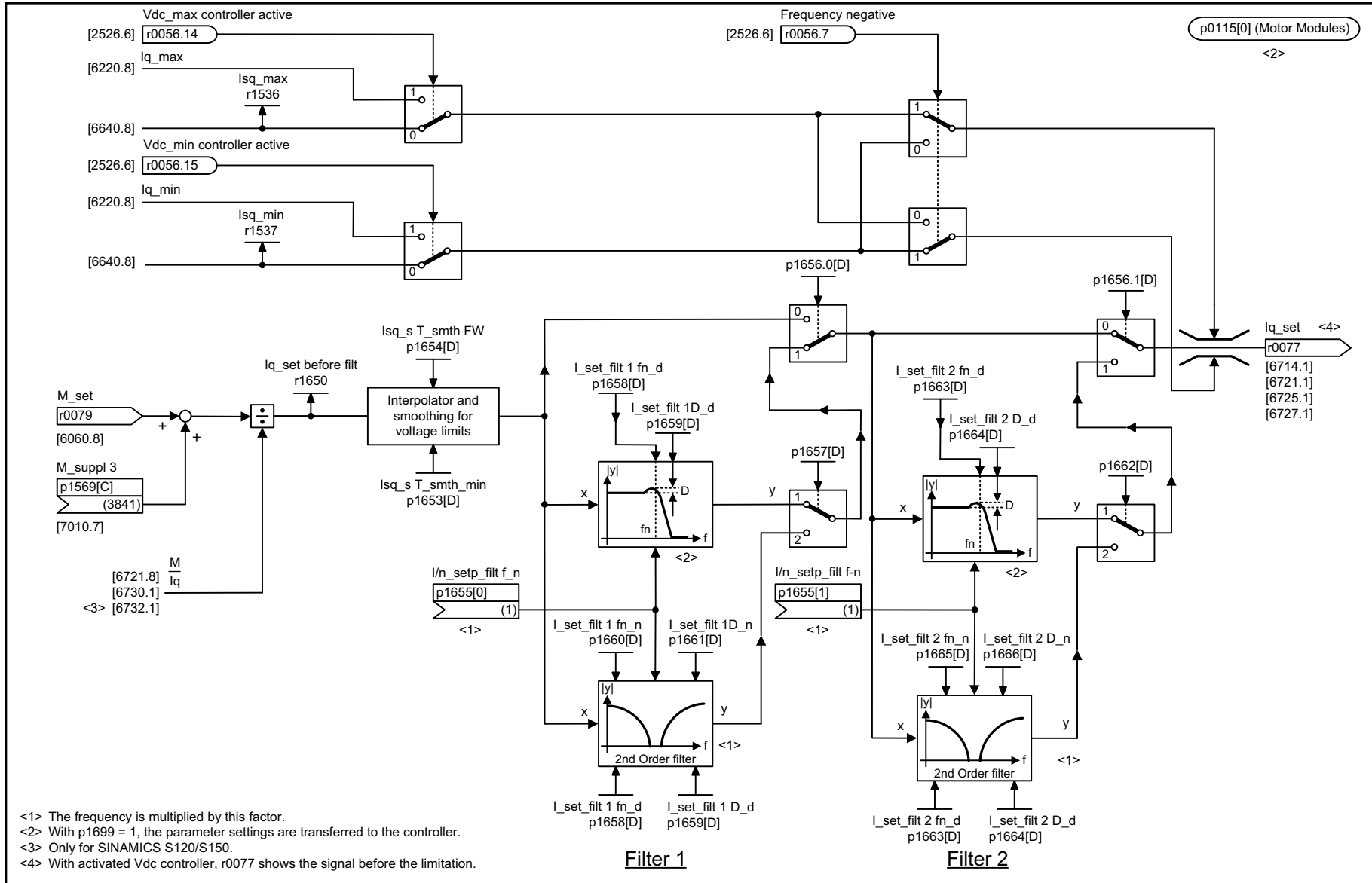
Fig. 3-251 6710 – Current setpoint filter
