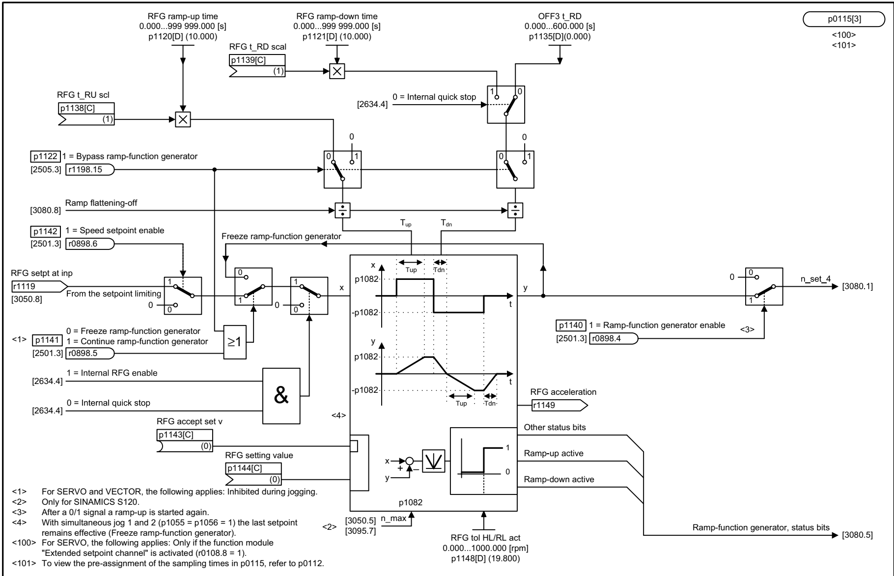
Fig. 3-162 3060 – Basic ramp-function generator
