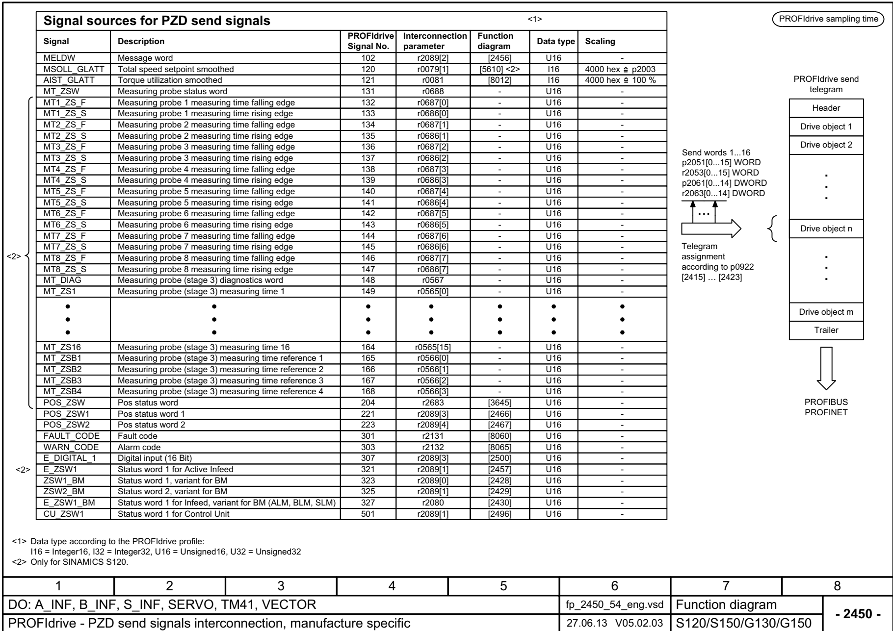
Fig. 3-61 2450 – PZD send signals interconnection manufacturer-specific
