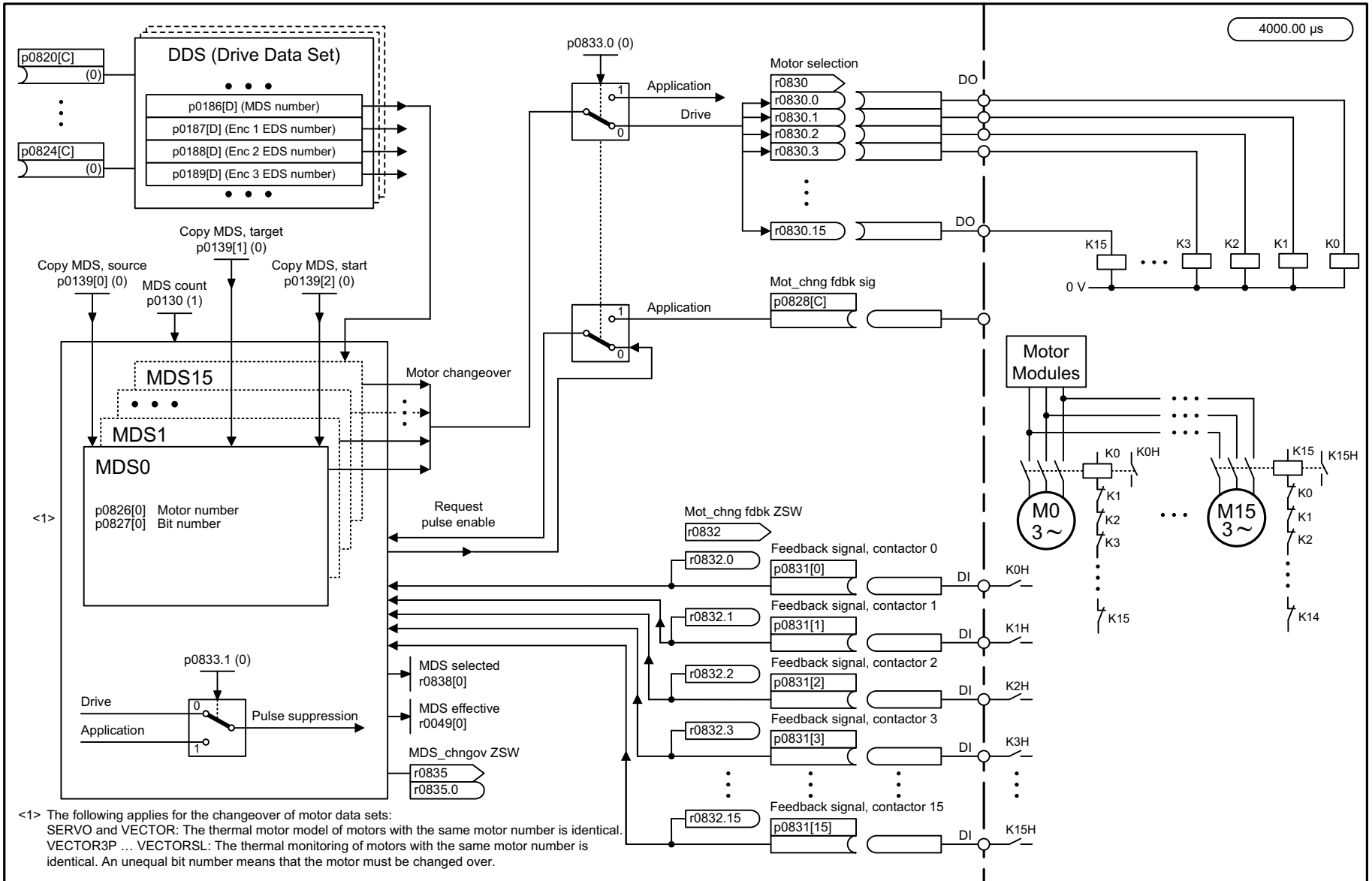
Fig. 3-324 8575 – Motor Data Sets (MDS)
