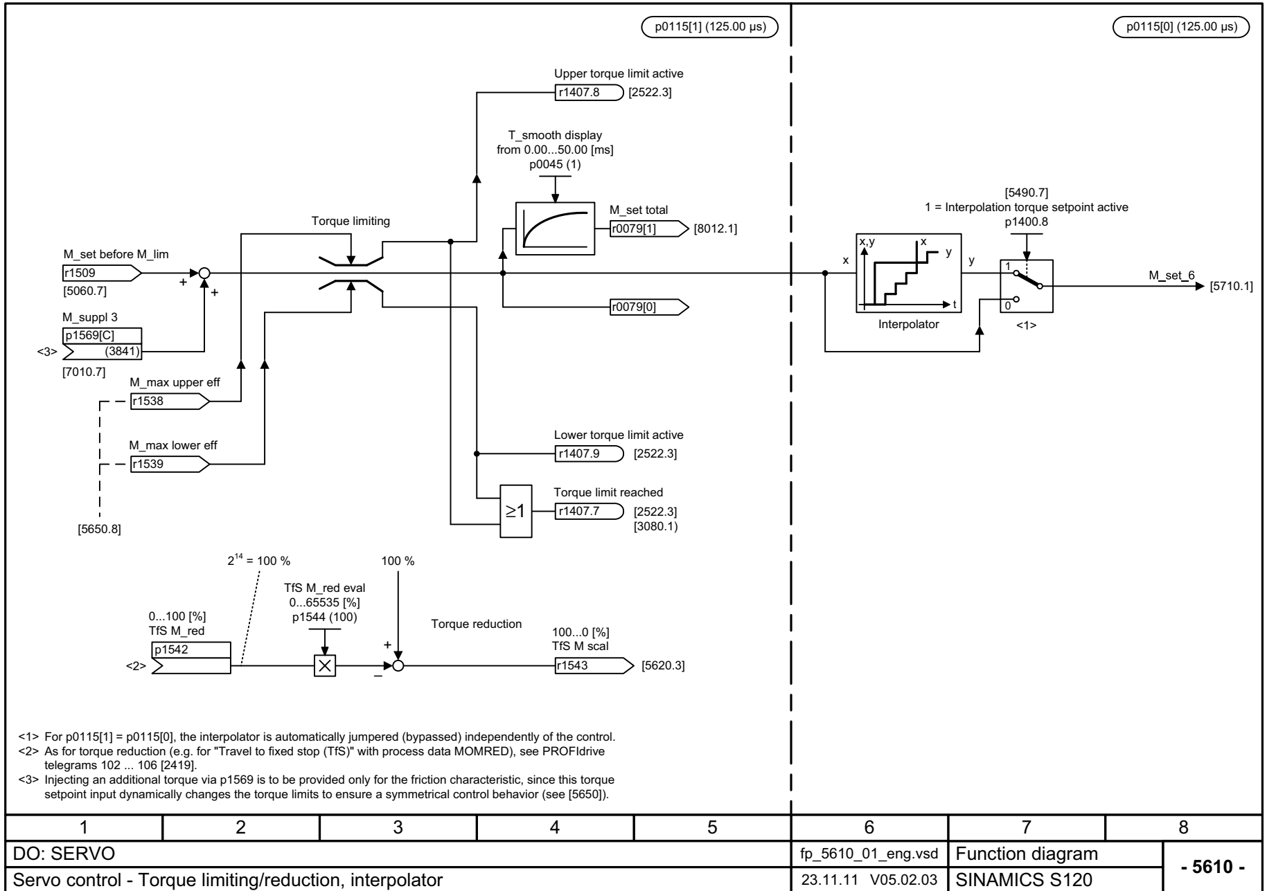
Fig. 3-2-22 5610 – Torque limiting/reduction, interpolator
