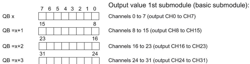
Figure 4-3 Address space for configuration as 1 x 64-channel DI 32x24VDC SNK/SRC/DQ 32x24VDC/0.3A SNK BA MSI/MSO
