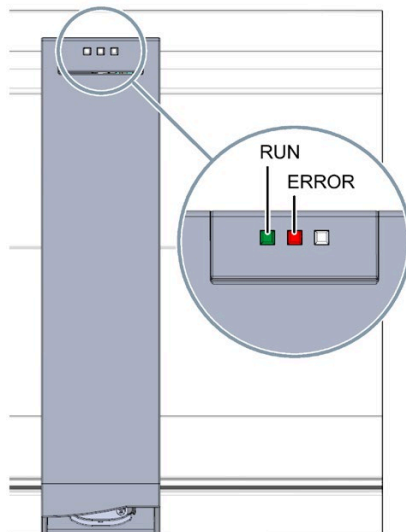
Figure 5-1 LED displays of the DI 32x24VDC SNK/SRC/DQ 32x24VDC/0.3A SNK BA module
