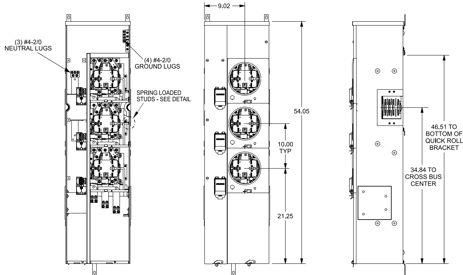
VIEW SHOWN WITHOUT COVERS
