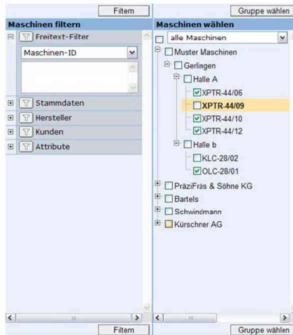
Figure 7-3 Pop-up window
