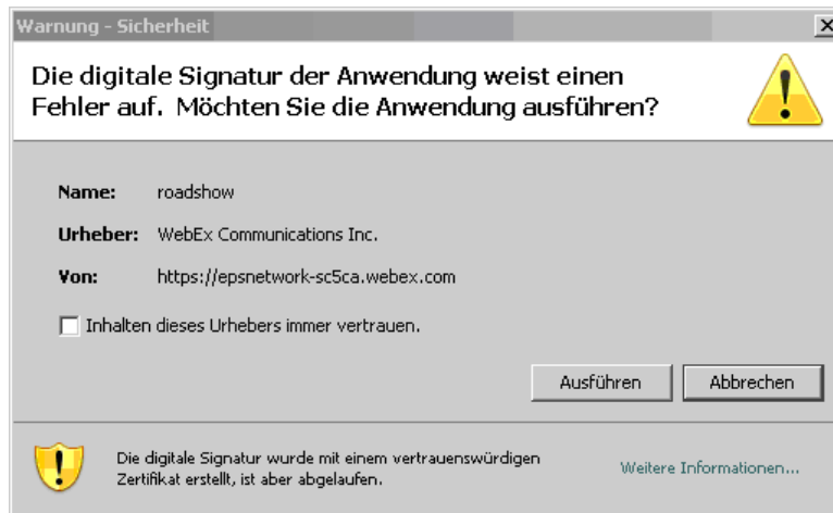
Figure 8-4 Error message
