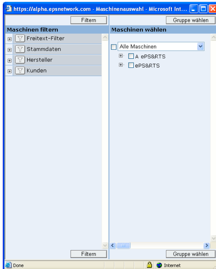
Figure 8-10 Management → Machine
