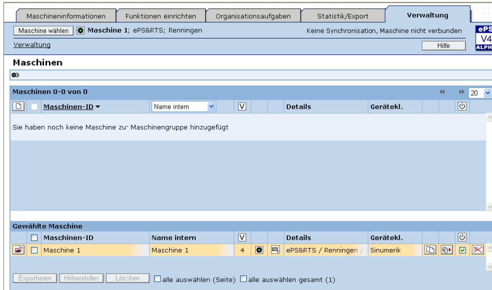
Figure 8-9 Management → Machine
