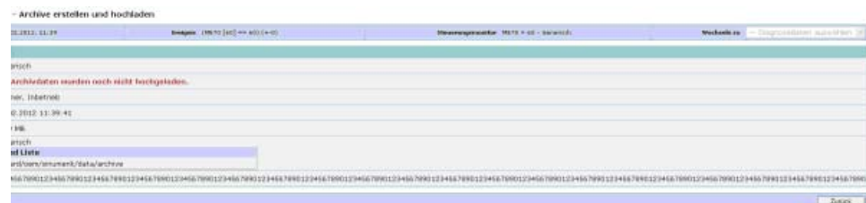
Figure 4-2 Comment input
