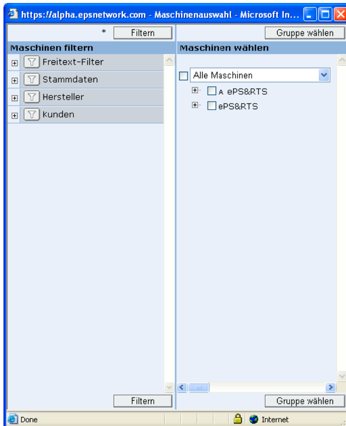
Figure 8-8 Pop-up window
