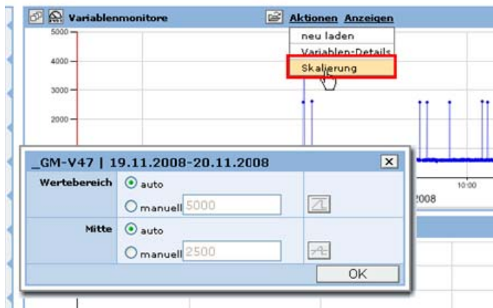
Figure 7-8 Scaling
