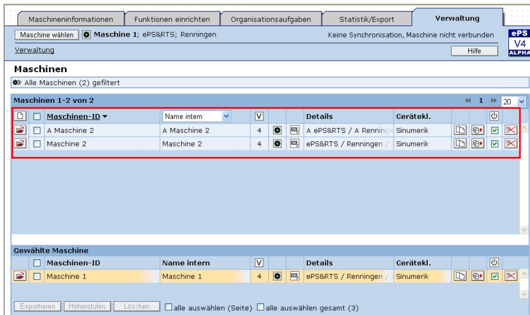
Figure 8-11 Management → Machines
