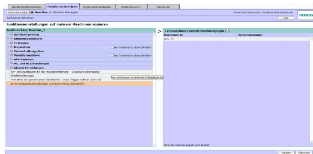
Figure 1-16 Multi-machine view
