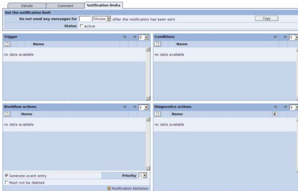
Figure 1-17 Set notification
