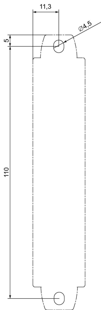
Drilling diagram, enclosure 22.5 mm
