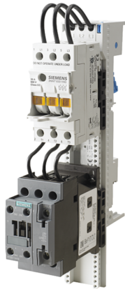
Figure 4-2 Installation configuration of a cylindrical fuse holder and a SIRIUS contactor on busbar device adapter for the 60 mm busbar system
