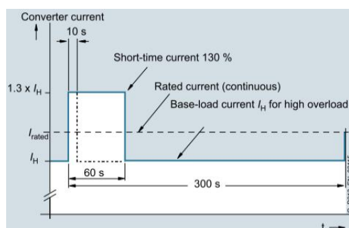
Load cycle definition for high overload for Motor Modules 6SL3325-1TG41-3AA7 and 6SL3325-1TG41-6AA7
