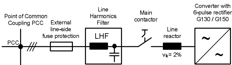
Additional components required in conjunction with stand-alone Line Harmonics Filters (LHF)
