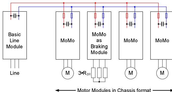
Drive configuration comprising multiple S120 Motor Modules and one S120 Motor Module as a Braking Module
