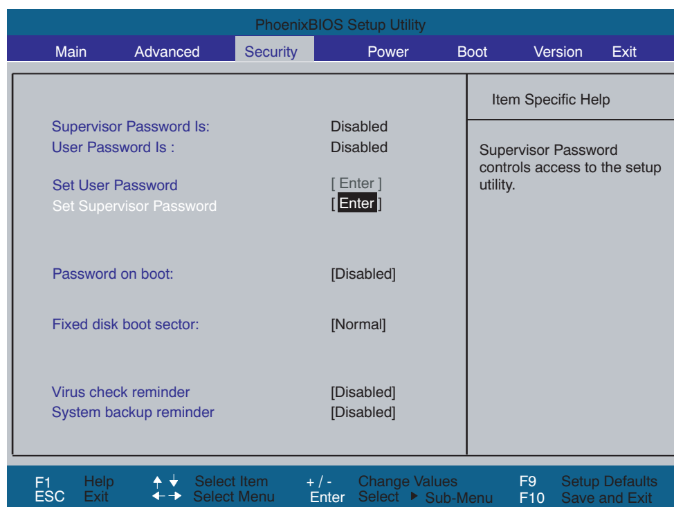
Figure 13-18 Security menu
