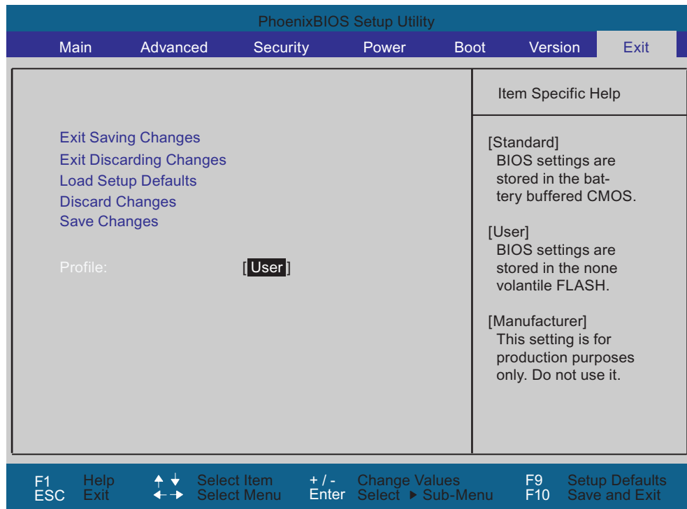
Figure 13-23 Exit menu
