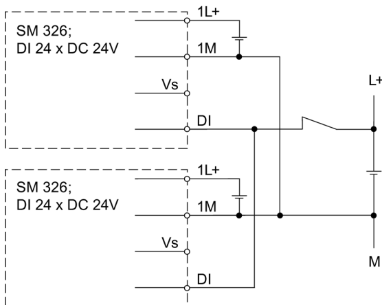
Figure 8-11 Wiring scheme of the SM 326; DI 24 x DC 24V for application 4 – one sensor single-channel connection
