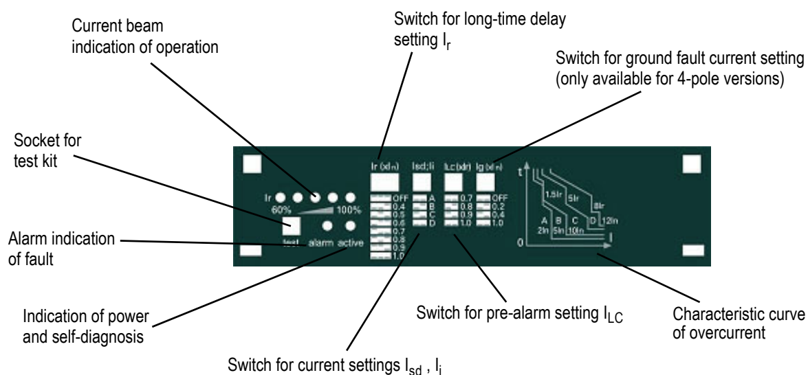
(19) VT630 front of ETU
