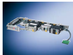
SIVACON in-line module with SIMOCODE pro (50 mm height)
