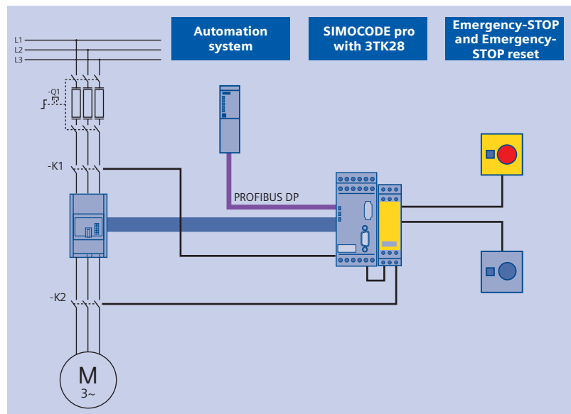
Safe consumer shutdown with SIMOCODE pro
