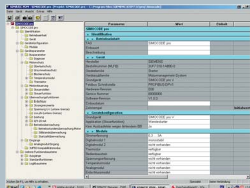
SIMATIC PDM
