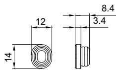
3SX5600-1G
