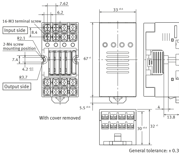
External dimensions
