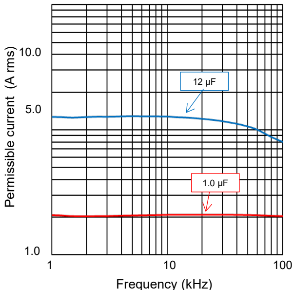
[ Permissible Current ]
