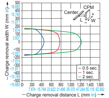
Charge removal field (vertical direction, 0.5 MPa, 50 Hz)
