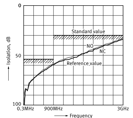
Isolation characteristics
