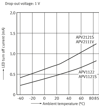
4. LED turn off current vs. ambient temperature characteristics
