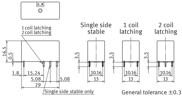
External dimensions
